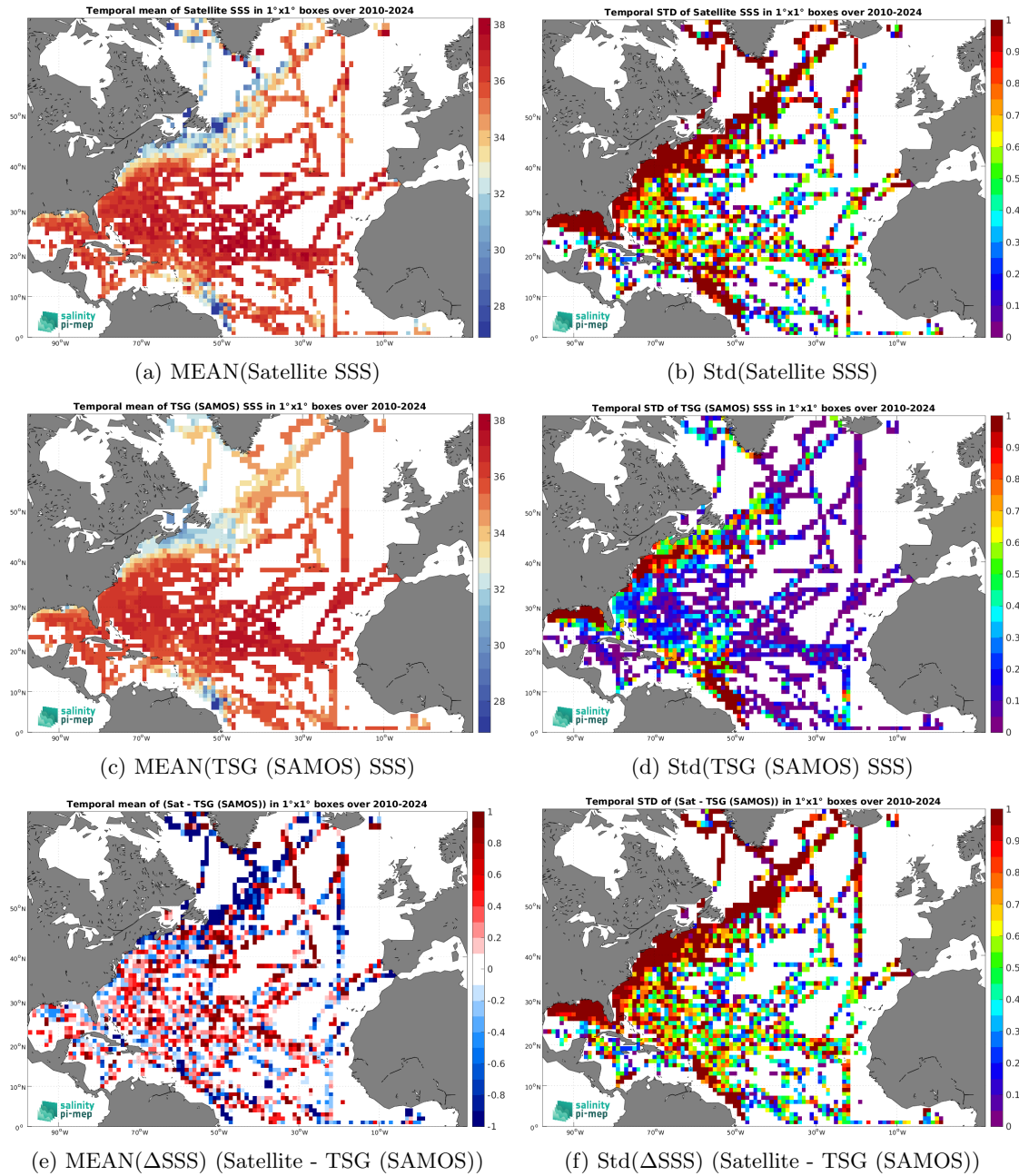
Figure 7: Temporal mean (left) and Std (right) of SSS from SMOS SSS L2Q v331 - No FLAG (CMEMS-CATDS-CPDC) (top), TSG (SAMOS) (middle), and of \Delta SSS (Satellite - TSG (SAMOS)). Only match-up pairs are used to generate these maps.
