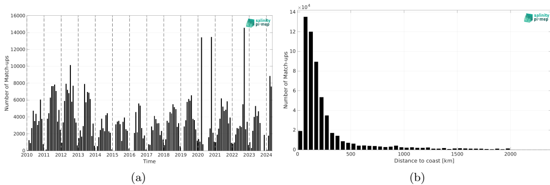
Figure 2: Number of match-ups between TSG (SAMOS) and SMOS SSS L2Q v331 - No FLAG (CMEMS-CATDS-CPDC) SSS as a function of time (a) and as function of the distance to coast (b) over the North Atlantic Ocean Pi-MEP region and for the full satellite product period.
