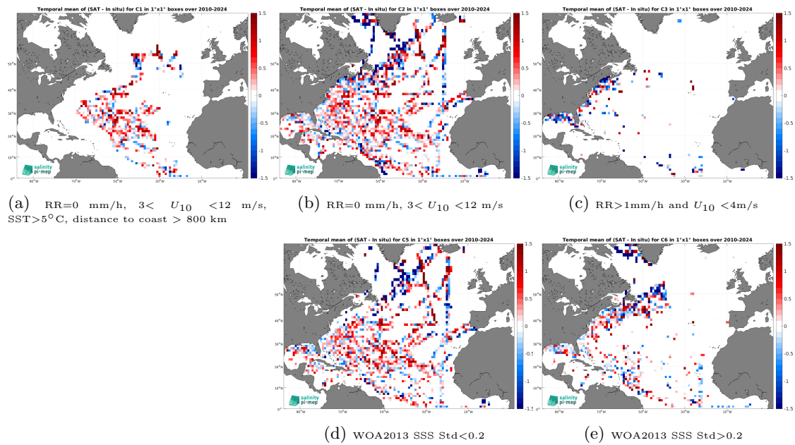
Figure 14: Temporal mean gridded over spatial boxes of size 1^\circ \times 1^\circ of \Delta\text{SSS} (SMOS SSS L2Q v331 - No FLAG (CMEMS-CATDS-CPDC) - TSG (SAMOS)) for 5 different subdatasets corresponding to:RR=0 mm/h, 3 < U_{10} < 12 m/s, SST >5^\circ\text{C} , distance to coast > 800 km (a), RR=0 mm/h, 3 < U_{10} < 12 m/s (b), RR >1 mm/h and U_{10} < 4 m/s (c), WOA2013 SSS Std <0.2 (d), WOA2013 SSS Std >0.2 (e).
