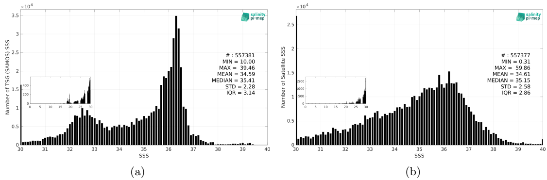
Figure 3: Histograms of SSS from TSG (SAMOS) (a) and SMOS SSS L2Q v331 - No FLAG (CMEMS-CATDS-CPDC) (b) considering all match-up pairs per bins of 0.1 over the North Atlantic Ocean Pi-MEP region and for the full satellite product period.
