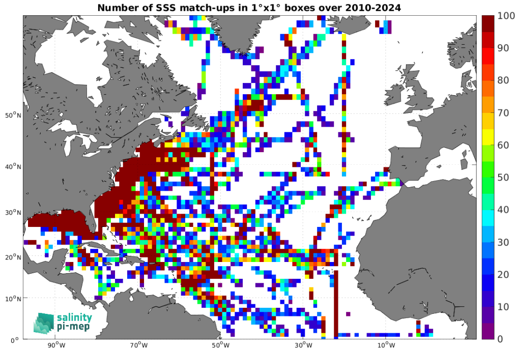
Figure 5: Number of SSS match-ups between TSG (SAMOS) SSS and the SMOS SSS L2Q v331 - No FLAG (CMEMS-CATDS-CPDC) SSS product for the North Atlantic Ocean Pi-MEP region over 1^\circ \times 1^\circ boxes and for the full satellite product period.
