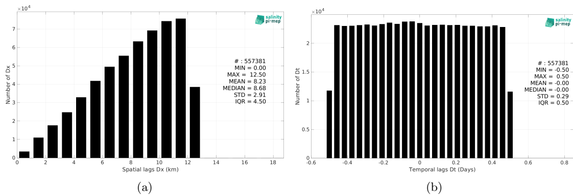
Figure 6: Histograms of the spatial (a) and temporal (b) lags between the location/time of the TSG (SAMOS) measurement and the date of the corresponding SMOS SSS L2Q v331 - No FLAG (CMEMS-CATDS-CPDC) SSS pixel.
