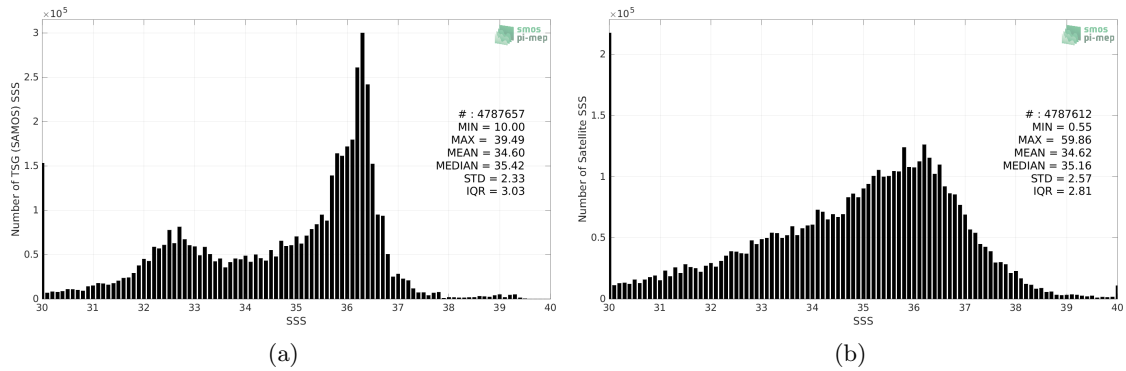
Figure 2: Histograms of SSS from TSG (SAMOS) (a) and SMOS SSS L2Q v331 - No FLAG (CMEMS-CATDS-CPDC) (b) considering all match-up pairs per bins of 0.1 over the North Atlantic Ocean Pi-MEP region and for the full satellite product period.
