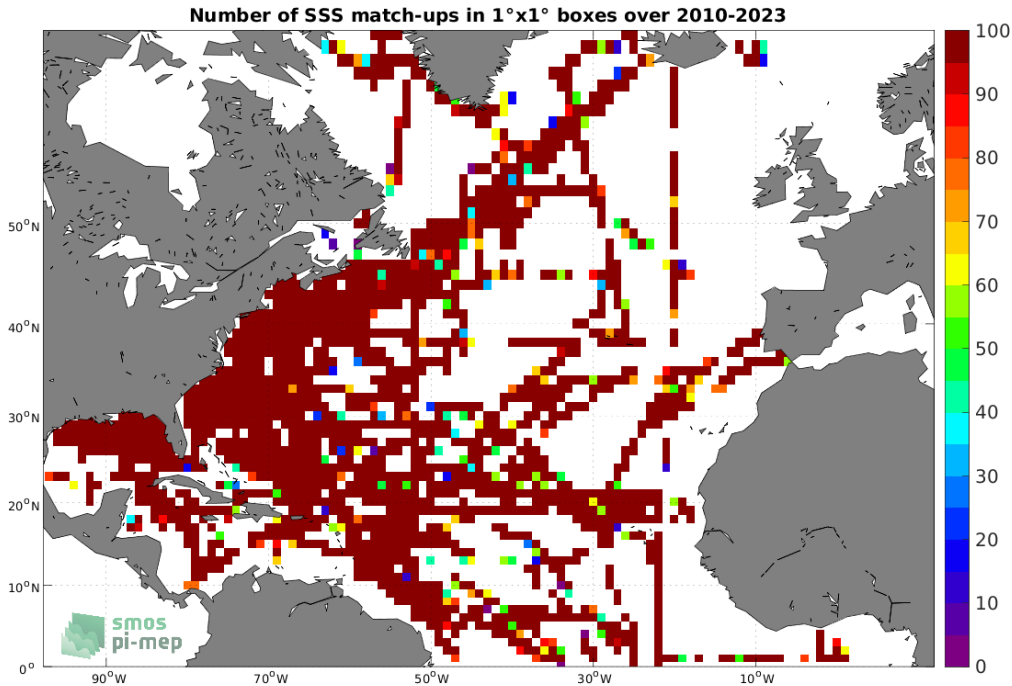
Figure 4: Number of SSS match-ups between TSG (SAMOS) SSS and the SMOS SSS L2Q v331 - No FLAG (CMEMS-CATDS-CPDC) SSS product for the North Atlantic Ocean Pi-MEP region over 1^\circ \times 1^\circ boxes and for the full satellite product period.
