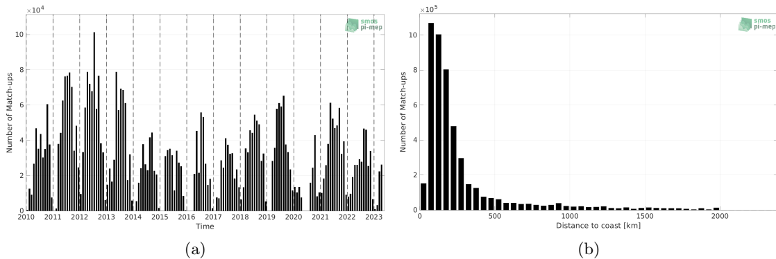
Figure 1: Number of match-ups between TSG (SAMOS) and SMOS SSS L2Q v331 - No FLAG (CMEMS-CATDS-CPDC) SSS as a function of time (a) and as function of the distance to coast (b) over the North Atlantic Ocean Pi-MEP region and for the full satellite product period.
