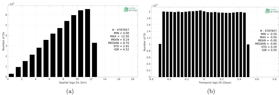
Figure 5: Histograms of the spatial (a) and temporal (b) lags between the location/time of the TSG (SAMOS) measurement and the date of the corresponding SMOS SSS L2Q v331 - No FLAG (CMEMS-CATDS-CPDC) SSS pixel.
