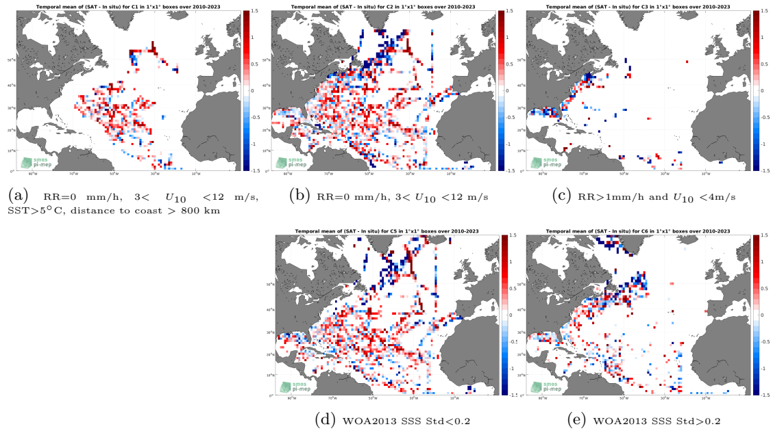
Figure 12: Temporal mean gridded over spatial boxes of size 1^\circ \times 1^\circ of \Delta\text{SSS} (SMOS SSS L2Q v331 - No FLAG (CMEMS-CATDS-CPDC) - TSG (SAMOS)) for 5 different subdatasets corresponding to:RR=0 mm/h, 3 < U_{10} < 12 m/s, SST >5^\circ\text{C} , distance to coast > 800 km (a), RR=0 mm/h, 3 < U_{10} < 12 m/s (b), RR >1 mm/h and U_{10} < 4 m/s (c), WOA2013 SSS Std <0.2 (d), WOA2013 SSS Std >0.2 (e).
