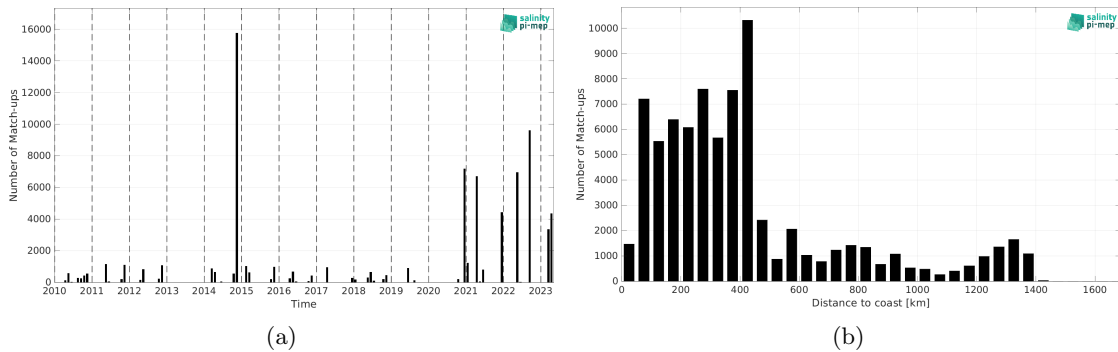
Figure 2: Number of match-ups between TSG (Polarstern) and SMOS SSS L2Q v331 - No FLAG (CMEMS-CATDS-CPDC) SSS as a function of time (a) and as function of the distance to coast (b) over the North Atlantic Ocean Pi-MEP region and for the full satellite product period.
