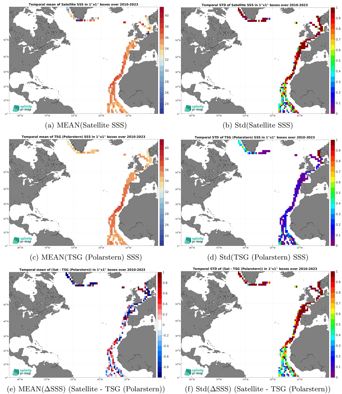
Figure 7: Temporal mean (left) and Std (right) of SSS from SMOS SSS L2Q v331 - No FLAG (CMEMS-CATDS-CPDC) (top), TSG (Polarstern) (middle), and of \Delta SSS (Satellite - TSG (Polarstern)). Only match-up pairs are used to generate these maps.
