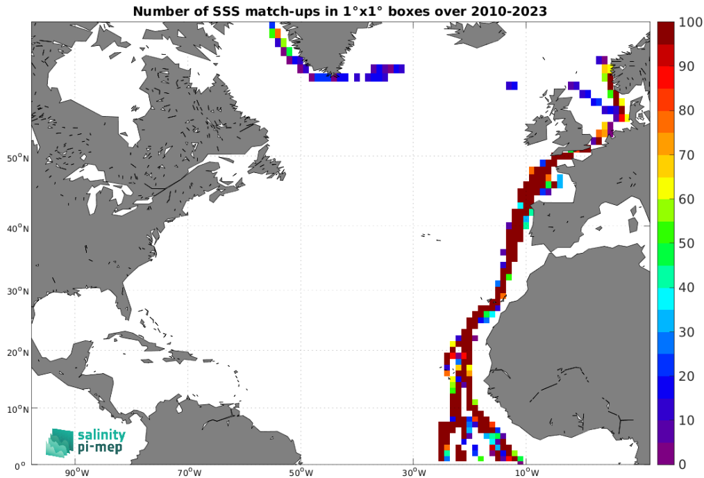
Figure 5: Number of SSS match-ups between TSG (Polarstern) SSS and the SMOS SSS L2Q v331 - No FLAG (CMEMS-CATDS-CPDC) SSS product for the North Atlantic Ocean Pi-MEP region over 1^\circ \times 1^\circ boxes and for the full satellite product period.
