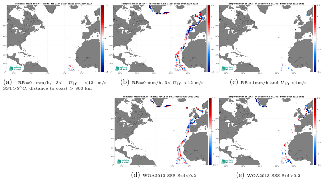
Figure 14: Temporal mean gridded over spatial boxes of size 1^\circ \times 1^\circ of \Delta\text{SSS} (SMOS SSS L2Q v331 - No FLAG (CMEMS-CATDS-CPDC) - TSG (Polarstern)) for 5 different subdatasets corresponding to:RR=0 mm/h, 3 < U_{10} < 12 m/s, SST >5^\circ\text{C} , distance to coast > 800 km (a), RR=0 mm/h, 3 < U_{10} < 12 m/s (b), RR >1 mm/h and U_{10} < 4 m/s (c), WOA2013 SSS Std <0.2 (d), WOA2013 SSS Std >0.2 (e).
