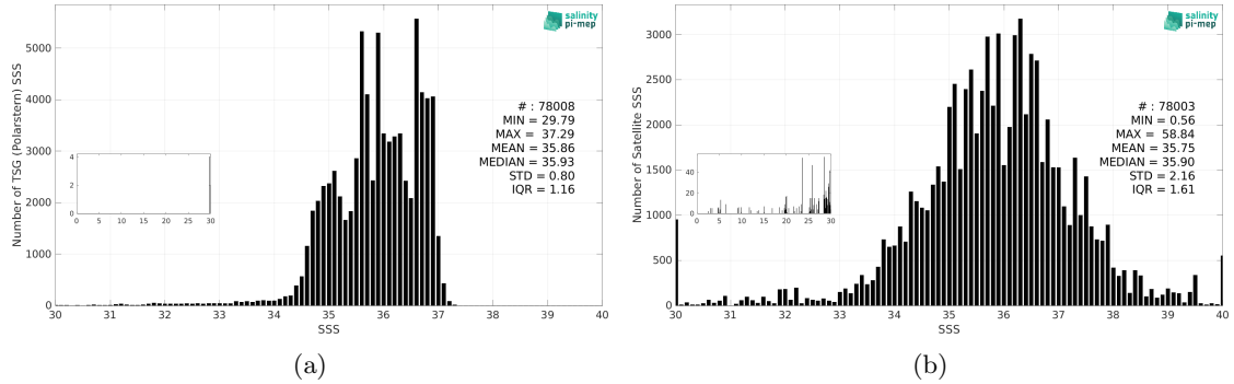
Figure 3: Histograms of SSS from TSG (Polarstern) (a) and SMOS SSS L2Q v331 - No FLAG (CMEMS-CATDS-CPDC) (b) considering all match-up pairs per bins of 0.1 over the North Atlantic Ocean Pi-MEP region and for the full satellite product period.
