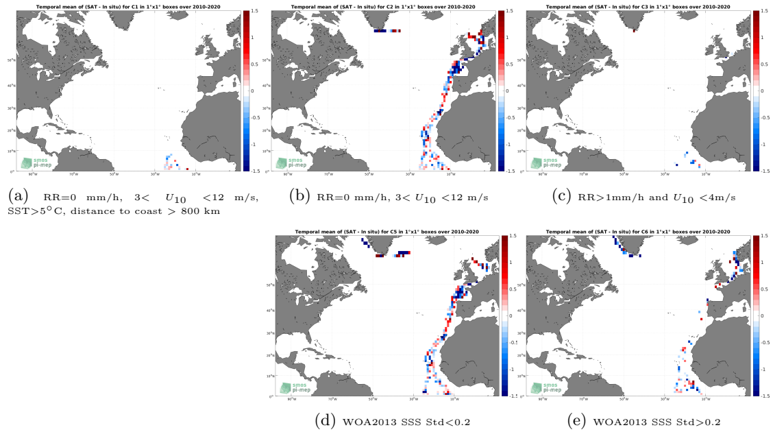
Figure 12: Temporal mean gridded over spatial boxes of size 1^\circ \times 1^\circ of \Delta\text{SSS} (SMOS SSS L2Q v331 - No FLAG (CMEMS-CATDS-CPDC) - TSG (Polarstern)) for 5 different subdatasets corresponding to:RR=0 mm/h, 3 < U_{10} < 12 m/s, SST >5^\circ\text{C} , distance to coast > 800 km (a), RR=0 mm/h, 3 < U_{10} < 12 m/s (b), RR >1 mm/h and U_{10} < 4 m/s (c), WOA2013 SSS Std <0.2 (d), WOA2013 SSS Std >0.2 (e).
