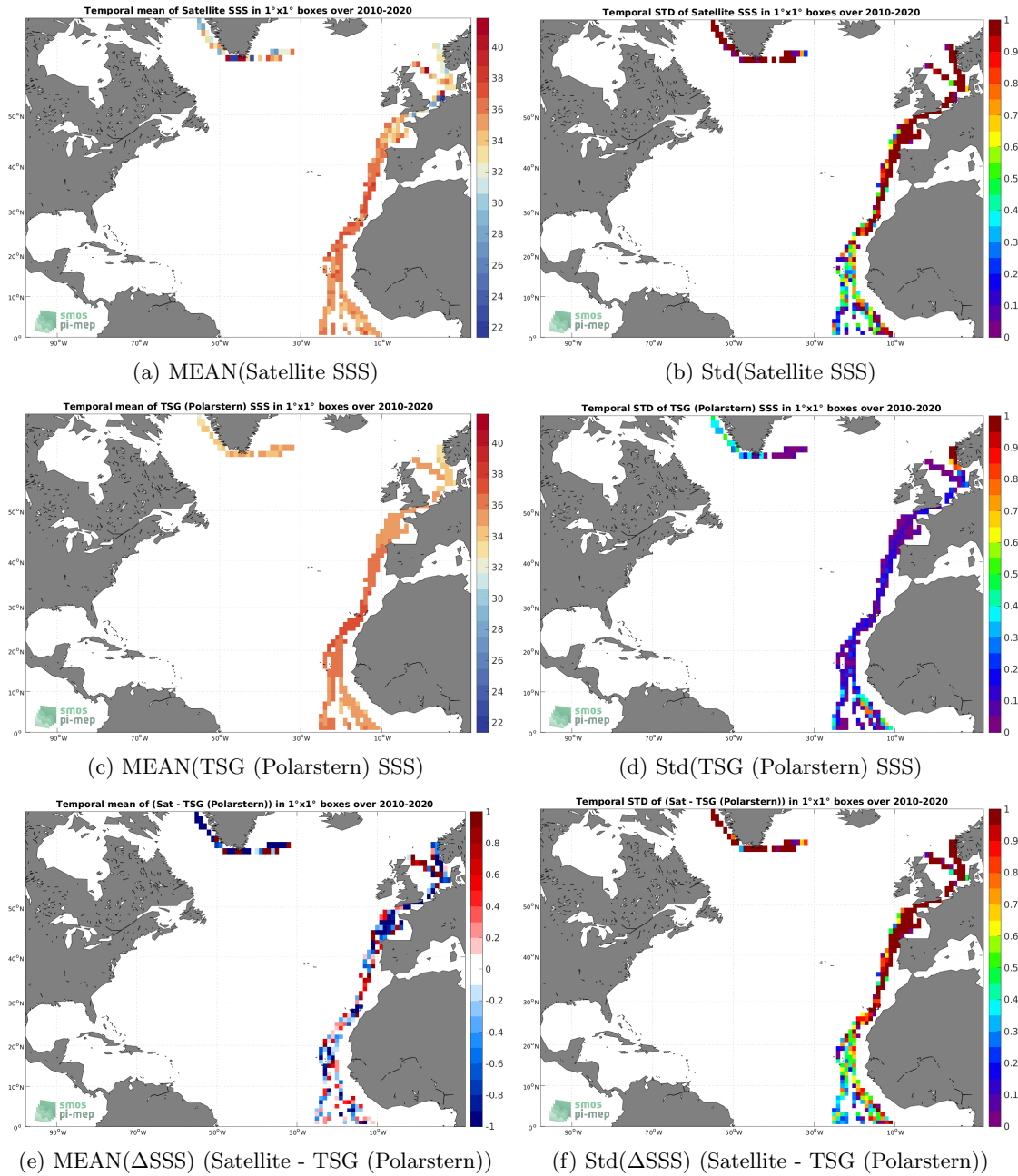
Figure 6: Temporal mean (left) and Std (right) of SSS from SMOS SSS L2Q v331 - No FLAG (CMEMS-CATDS-CPDC) (top), TSG (Polarstern) (middle), and of \Delta SSS (Satellite - TSG (Polarstern)). Only match-up pairs are used to generate these maps.
