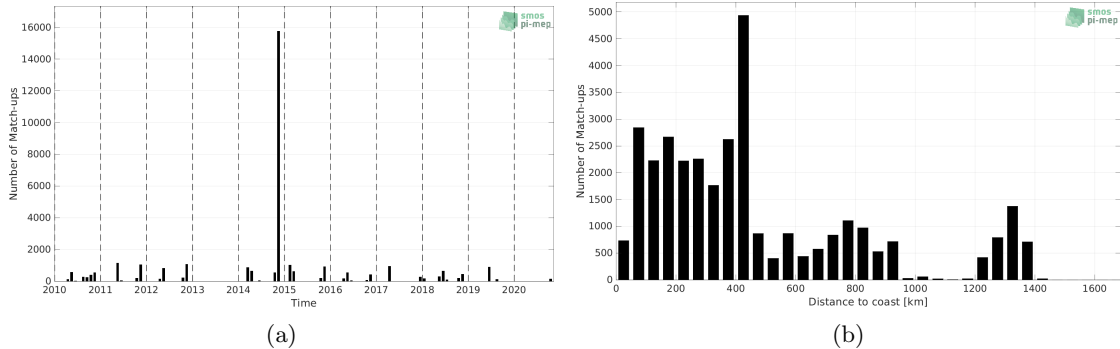
Figure 1: Number of match-ups between TSG (Polarstern) and SMOS SSS L2Q v331 - No FLAG (CMEMS-CATDS-CPDC) SSS as a function of time (a) and as function of the distance to coast (b) over the North Atlantic Ocean Pi-MEP region and for the full satellite product period.
