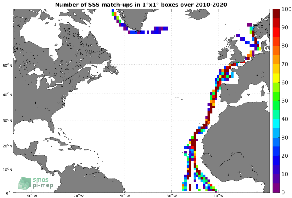
Figure 4: Number of SSS match-ups between TSG (Polarstern) SSS and the SMOS SSS L2Q v331 - No FLAG (CMEMS-CATDS-CPDC) SSS product for the North Atlantic Ocean Pi-MEP region over 1^\circ \times 1^\circ boxes and for the full satellite product period.
