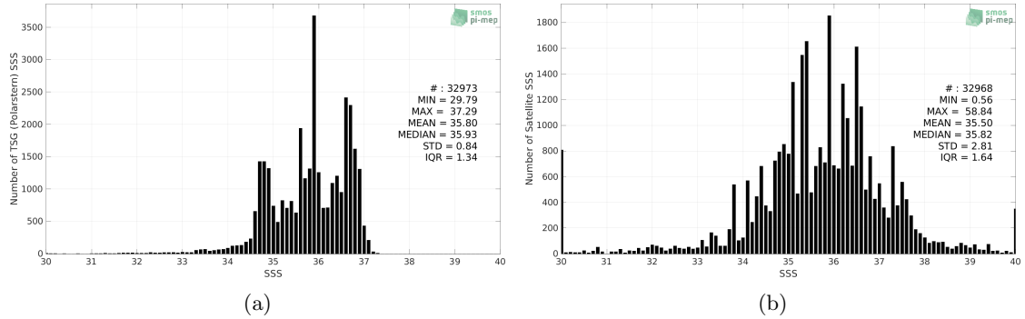
Figure 2: Histograms of SSS from TSG (Polarstern) (a) and SMOS SSS L2Q v331 - No FLAG (CMEMS-CATDS-CPDC) (b) considering all match-up pairs per bins of 0.1 over the North Atlantic Ocean Pi-MEP region and for the full satellite product period.
