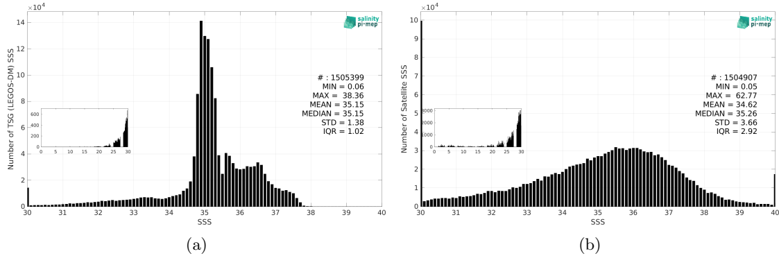
Figure 3: Histograms of SSS from TSG (LEGOS-DM) (a) and SMOS SSS L2Q v331 - No FLAG (CMEMS-CATDS-CPDC) (b) considering all match-up pairs per bins of 0.1 over the North Atlantic Ocean Pi-MEP region and for the full satellite product period.
