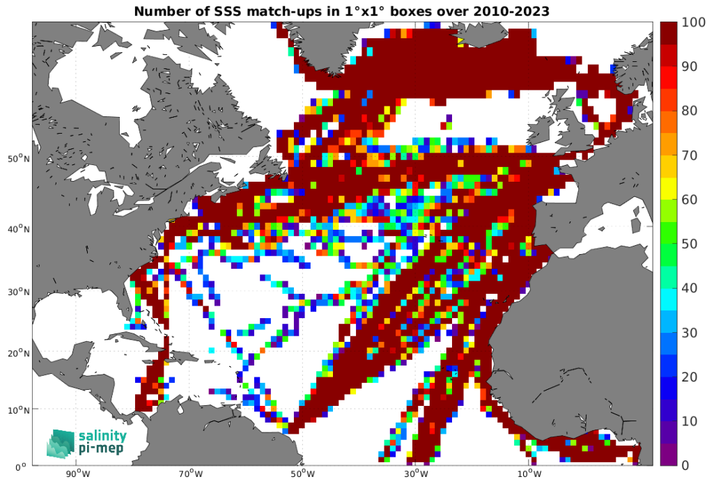
Figure 5: Number of SSS match-ups between TSG (LEGOS-DM) SSS and the SMOS SSS L2Q v331 - No FLAG (CMEMS-CATDS-CPDC) SSS product for the North Atlantic Ocean Pi-MEP region over 1^\circ \times 1^\circ boxes and for the full satellite product period.
