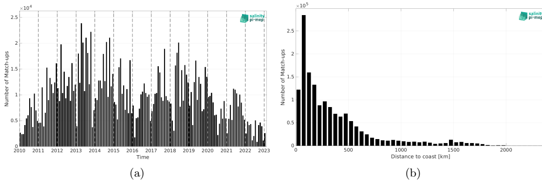
Figure 2: Number of match-ups between TSG (LEGOS-DM) and SMOS SSS L2Q v331 - No FLAG (CMEMS-CATDS-CPDC) SSS as a function of time (a) and as function of the distance to coast (b) over the North Atlantic Ocean Pi-MEP region and for the full satellite product period.
