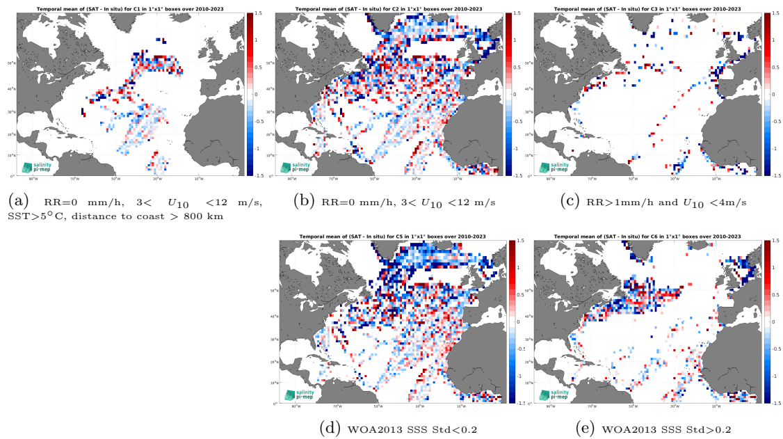
Figure 14: Temporal mean gridded over spatial boxes of size 1^\circ \times 1^\circ of \Delta\text{SSS} (SMOS SSS L2Q v331 - No FLAG (CMEMS-CATDS-CPDC) - TSG (LEGOS-DM)) for 5 different subdatasets corresponding to:RR=0 mm/h, 3 < U_{10} < 12 m/s, SST >5^\circ\text{C} , distance to coast > 800 km (a), RR=0 mm/h, 3 < U_{10} < 12 m/s (b), RR >1 mm/h and U_{10} < 4 m/s (c), WOA2013 SSS Std <0.2 (d), WOA2013 SSS Std >0.2 (e).
