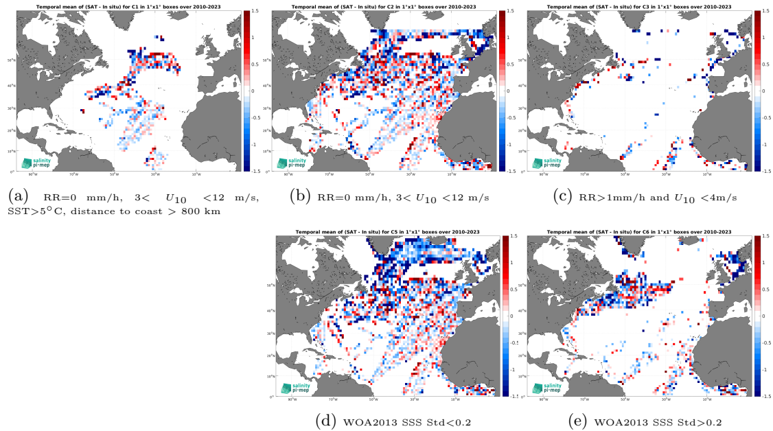
Figure 12: Temporal mean gridded over spatial boxes of size 1^\circ \times 1^\circ of \Delta\text{SSS} (SMOS SSS L2Q v331 - No FLAG (CMEMS-CATDS-CPDC) - TSG (LEGOS-DM)) for 5 different subdatasets corresponding to:RR=0 mm/h, 3 < U_{10} < 12 m/s, SST >5^\circ\text{C} , distance to coast > 800 km (a), RR=0 mm/h, 3 < U_{10} < 12 m/s (b), RR >1 mm/h and U_{10} < 4 m/s (c), WOA2013 SSS Std <0.2 (d), WOA2013 SSS Std >0.2 (e).
