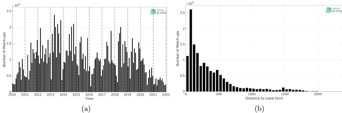
Figure 1: Number of match-ups between TSG (LEGOS-DM) and SMOS SSS L2Q v331 - No FLAG (CMEMS-CATDS-CPDC) SSS as a function of time (a) and as function of the distance to coast (b) over the North Atlantic Ocean Pi-MEP region and for the full satellite product period.
