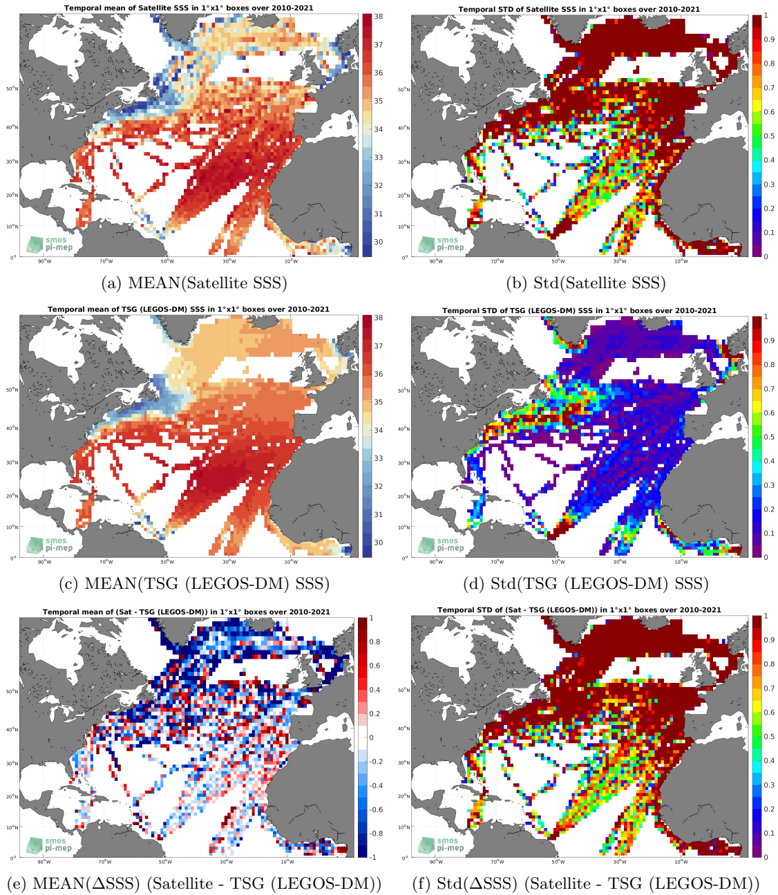
Figure 6: Temporal mean (left) and Std (right) of SSS from SMOS SSS L2Q v331 - No FLAG (CMEMS-CATDS-CPDC) (top), TSG (LEGOS-DM) (middle), and of \Delta SSS (Satellite - TSG (LEGOS-DM)). Only match-up pairs are used to generate these maps.
