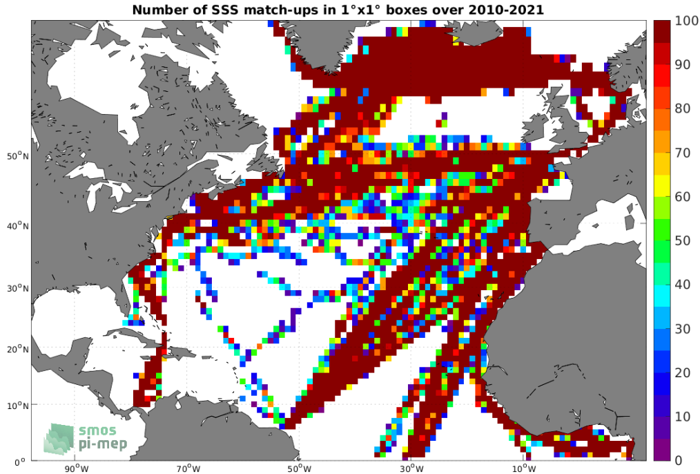
Figure 4: Number of SSS match-ups between TSG (LEGOS-DM) SSS and the SMOS SSS L2Q v331 - No FLAG (CMEMS-CATDS-CPDC) SSS product for the North Atlantic Ocean Pi-MEP region over 1^\circ \times 1^\circ boxes and for the full satellite product period.
