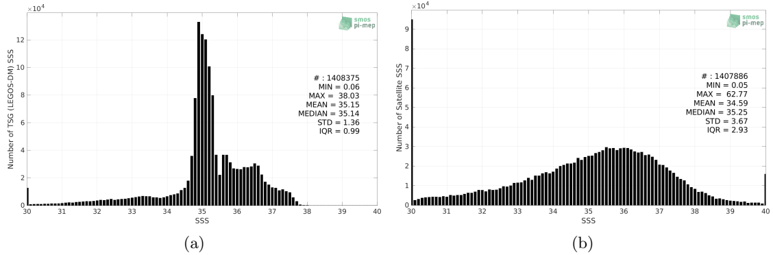
Figure 2: Histograms of SSS from TSG (LEGOS-DM) (a) and SMOS SSS L2Q v331 - No FLAG (CMEMS-CATDS-CPDC) (b) considering all match-up pairs per bins of 0.1 over the North Atlantic Ocean Pi-MEP region and for the full satellite product period.
