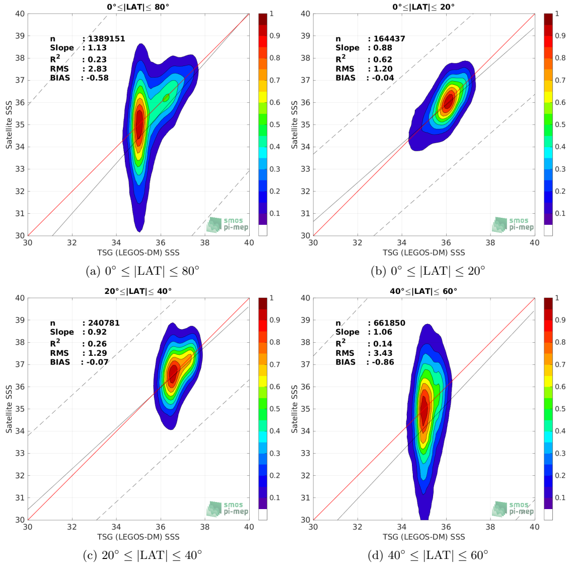
Figure 9: Contour maps of the concentration of SMOS SSS L2Q v331 - No FLAG (CMEMS-CATDS-CPDC) SSS ( y -axis) versus TSG (LEGOS-DM) SSS ( x -axis) at match-up pairs for different latitude bands. For each plot, the red line shows x=y . The black thin and dashed lines indicate a linear fit through the data cloud and the \pm 95\% confidence levels, respectively. The number match-up pairs n , the slope and R^2 coefficient of the linear fit, the root mean square (RMS) and the mean bias between satellite and in situ data are indicated for each latitude band in each plots.
