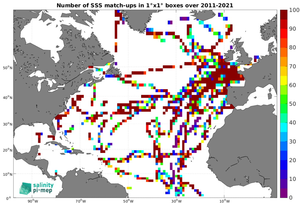
Figure 5: Number of SSS match-ups between TSG (GOSUD-Sailing-ship) SSS and the SMOS SSS L2Q v331 - No FLAG (CMEMS-CATDS-CPDC) SSS product for the North Atlantic Ocean Pi-MEP region over 1^\circ \times 1^\circ boxes and for the full satellite product period.
