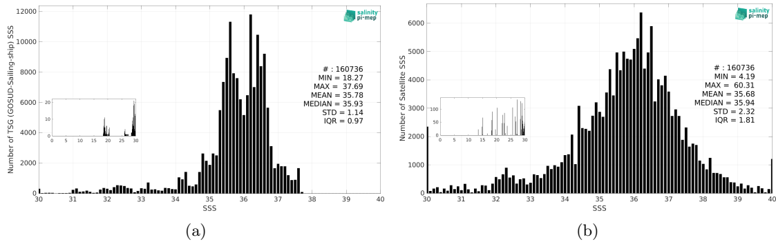
Figure 3: Histograms of SSS from TSG (GOSUD-Sailing-ship) (a) and SMOS SSS L2Q v331 - No FLAG (CMEMS-CATDS-CPDC) (b) considering all match-up pairs per bins of 0.1 over the North Atlantic Ocean Pi-MEP region and for the full satellite product period.
