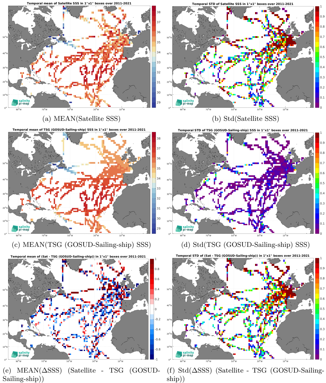
Figure 7: Temporal mean (left) and Std (right) of SSS from SMOS SSS L2Q v331 - No FLAG (CMEMS-CATDS-CPDC) (top), TSG (GOSUD-Sailing-ship) (middle), and of \Delta SSS (Satellite - TSG (GOSUD-Sailing-ship)). Only match-up pairs are used to generate these maps.
