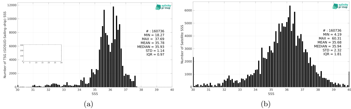
Figure 2: Histograms of SSS from TSG (GOSUD-Sailing-ship) (a) and SMOS SSS L2Q v331 - No FLAG (CMEMS-CATDS-CPDC) (b) considering all match-up pairs per bins of 0.1 over the North Atlantic Ocean Pi-MEP region and for the full satellite product period.
