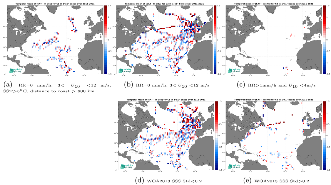
Figure 12: Temporal mean gridded over spatial boxes of size 1^\circ \times 1^\circ of \Delta\text{SSS} (SMOS SSS L2Q v331 - No FLAG (CMEMS-CATDS-CPDC) - TSG (GOSUD-Sailing-ship)) for 5 different sub-datasets corresponding to:RR=0 mm/h, 3 < U_{10} < 12 m/s, SST >5^\circ\text{C} , distance to coast > 800 km (a), RR=0 mm/h, 3 < U_{10} < 12 m/s (b), RR >1 mm/h and U_{10} < 4 m/s (c), WOA2013 SSS Std <0.2 (d), WOA2013 SSS Std >0.2 (e).
