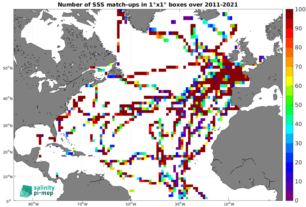
Figure 4: Number of SSS match-ups between TSG (GOSUD-Sailing-ship) SSS and the SMOS SSS L2Q v331 - No FLAG (CMEMS-CATDS-CPDC) SSS product for the North Atlantic Ocean Pi-MEP region over 1^\circ \times 1^\circ boxes and for the full satellite product period.
