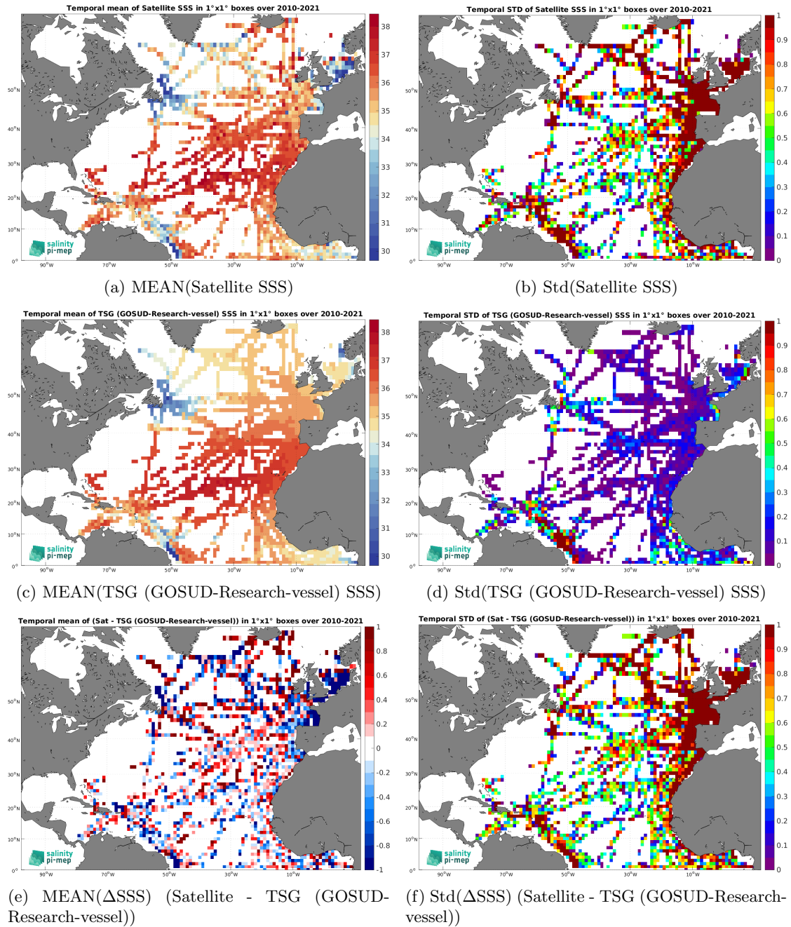
Figure 7: Temporal mean (left) and Std (right) of SSS from SMOS SSS L2Q v331 - No FLAG (CMEMS-CATDS-CPDC) (top), TSG (GOSUD-Research-vessel) (middle), and of \Delta SSS (Satellite - TSG (GOSUD-Research-vessel)). Only match-up pairs are used to generate these maps.
