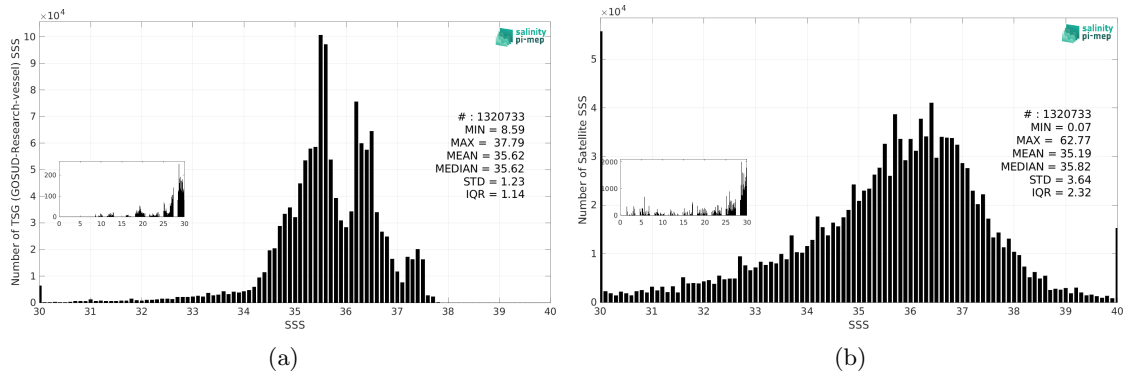
Figure 3: Histograms of SSS from TSG (GOSUD-Research-vessel) (a) and SMOS SSS L2Q v331 - No FLAG (CMEMS-CATDS-CPDC) (b) considering all match-up pairs per bins of 0.1 over the North Atlantic Ocean Pi-MEP region and for the full satellite product period.
