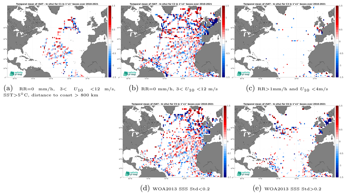
Figure 14: Temporal mean gridded over spatial boxes of size 1^\circ \times 1^\circ of \Delta\text{SSS} (SMOS SSS L2Q v331 - No FLAG (CMEMS-CATDS-CPDC) - TSG (GOSUD-Research-vessel)) for 5 different subdatasets corresponding to:RR=0 mm/h, 3 < U_{10} < 12 m/s, SST >5^\circ\text{C} , distance to coast > 800 km (a), RR=0 mm/h, 3 < U_{10} < 12 m/s (b), RR >1 mm/h and U_{10} < 4 m/s (c), WOA2013 SSS Std <0.2 (d), WOA2013 SSS Std >0.2 (e).
