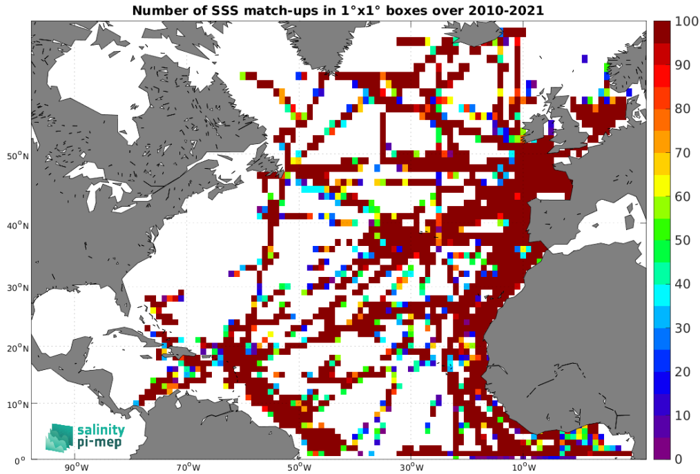
Figure 4: Number of SSS match-ups between TSG (GOSUD-Research-vessel) SSS and the SMOS SSS L2Q v331 - No FLAG (CMEMS-CATDS-CPDC) SSS product for the North Atlantic Ocean Pi-MEP region over 1^\circ \times 1^\circ boxes and for the full satellite product period.
