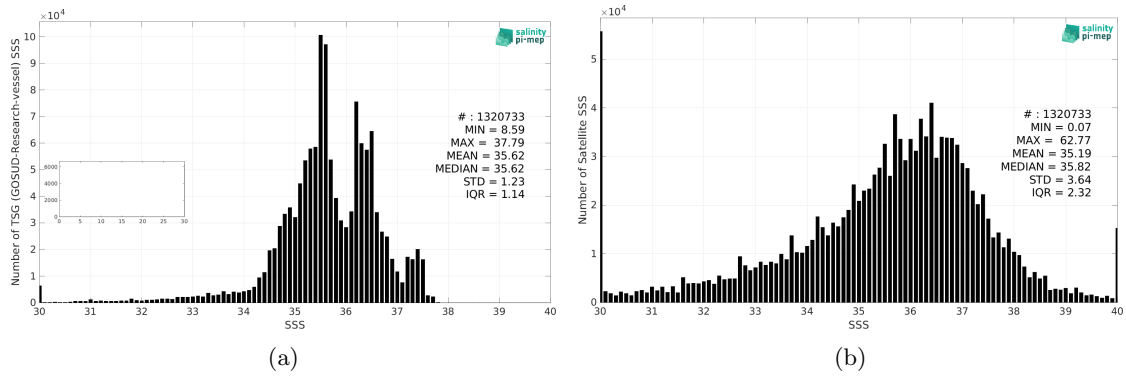
Figure 2: Histograms of SSS from TSG (GOSUD-Research-vessel) (a) and SMOS SSS L2Q v331 - No FLAG (CMEMS-CATDS-CPDC) (b) considering all match-up pairs per bins of 0.1 over the North Atlantic Ocean Pi-MEP region and for the full satellite product period.
