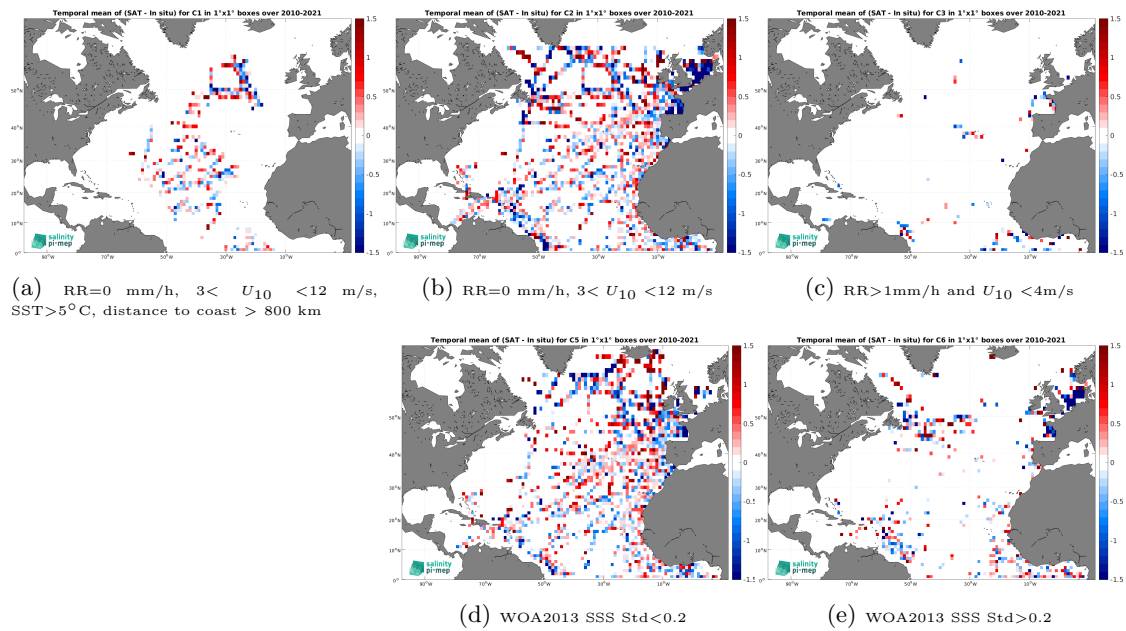
Figure 12: Temporal mean gridded over spatial boxes of size 1^\circ \times 1^\circ of \Delta\text{SSS} (SMOS SSS L2Q v331 - No FLAG (CMEMS-CATDS-CPDC) - TSG (GOSUD-Research-vessel)) for 5 different subdatasets corresponding to:RR=0 mm/h, 3 < U_{10} < 12 m/s, SST >5^\circ\text{C} , distance to coast > 800 km (a), RR=0 mm/h, 3 < U_{10} < 12 m/s (b), RR >1 mm/h and U_{10} < 4 m/s (c), WOA2013 SSS Std <0.2 (d), WOA2013 SSS Std >0.2 (e).
