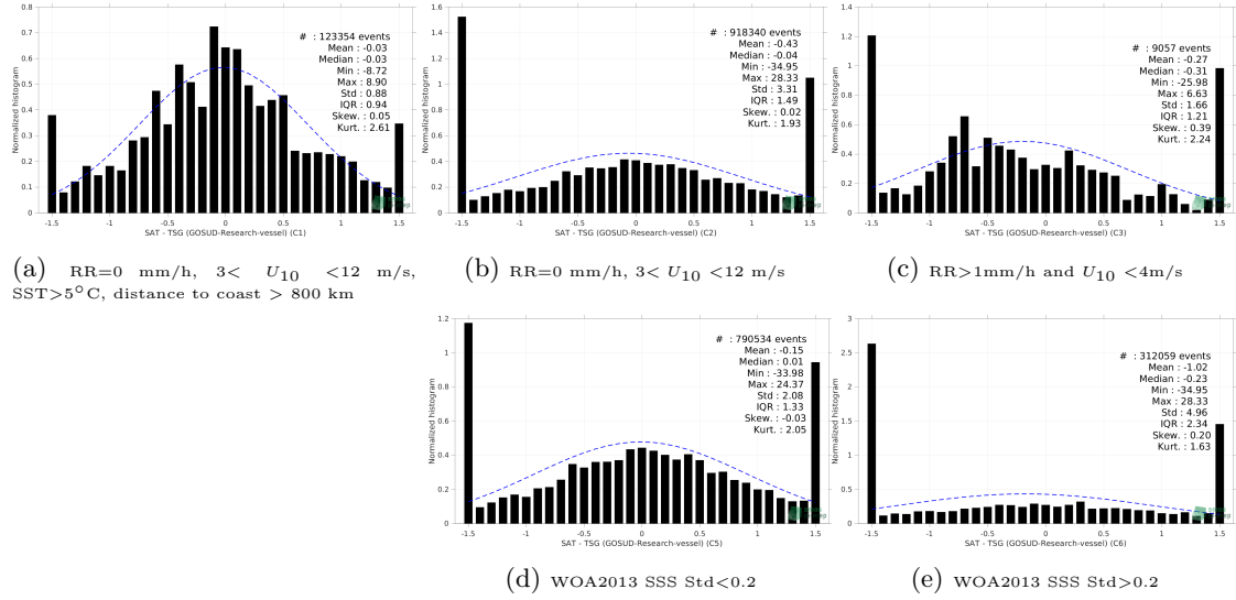
Figure 13: Normalized histogram of \Delta\text{SSS} (SMOS SSS L2Q v331 - No FLAG (CMEMS-CATDS-CPDC) - TSG (GOSUD-Research-vessel)) for 5 different subdatasets corresponding to: RR=0 mm/h, 3 < U_{10} < 12 m/s, SST > 5^\circ\text{C} , distance to coast > 800 km (a), RR=0 mm/h, 3 < U_{10} < 12 m/s (b), RR > 1 mm/h and U_{10} < 4 m/s (c), WOA2013 SSS Std < 0.2 (d), WOA2013 SSS Std > 0.2 (e).
