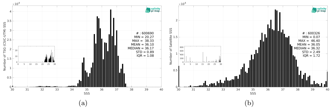
Figure 3: Histograms of SSS from TSG (CSIC-UTM) (a) and SMOS SSS L2Q v331 - No FLAG (CMEMS-CATDS-CPDC) (b) considering all match-up pairs per bins of 0.1 over the North Atlantic Ocean Pi-MEP region and for the full satellite product period.
