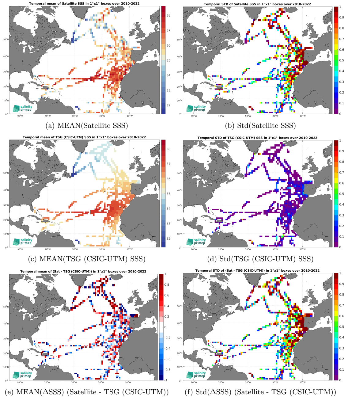
Figure 7: Temporal mean (left) and Std (right) of SSS from SMOS SSS L2Q v331 - No FLAG (CMEMS-CATDS-CPDC) (top), TSG (CSIC-UTM) (middle), and of \Delta SSS (Satellite - TSG (CSIC-UTM)). Only match-up pairs are used to generate these maps.
