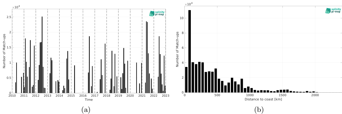
Figure 2: Number of match-ups between TSG (CSIC-UTM) and SMOS SSS L2Q v331 - No FLAG (CMEMS-CATDS-CPDC) SSS as a function of time (a) and as function of the distance to coast (b) over the North Atlantic Ocean Pi-MEP region and for the full satellite product period.
