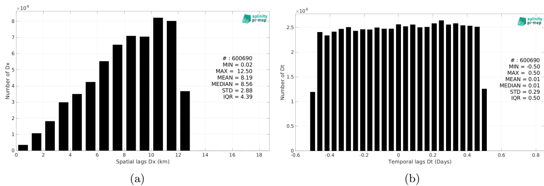
Figure 6: Histograms of the spatial (a) and temporal (b) lags between the location/time of the TSG (CSIC-UTM) measurement and the date of the corresponding SMOS SSS L2Q v331 - No FLAG (CMEMS-CATDS-CPDC) SSS pixel.
