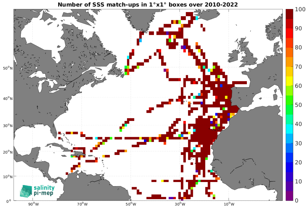
Figure 4: Number of SSS match-ups between TSG (CSIC-UTM) SSS and the SMOS SSS L2Q v331 - No FLAG (CMEMS-CATDS-CPDC) SSS product for the North Atlantic Ocean Pi-MEP region over 1^\circ \times 1^\circ boxes and for the full satellite product period.
