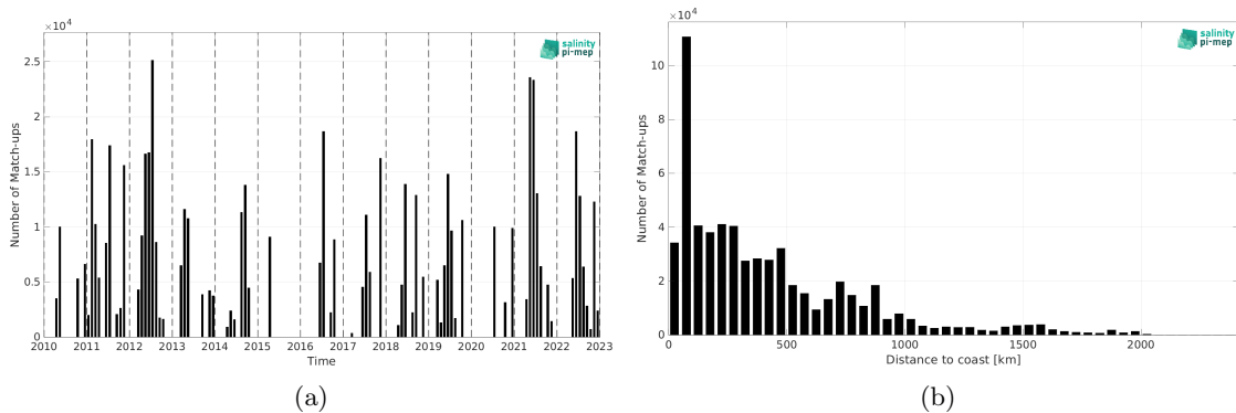
Figure 1: Number of match-ups between TSG (CSIC-UTM) and SMOS SSS L2Q v331 - No FLAG (CMEMS-CATDS-CPDC) SSS as a function of time (a) and as function of the distance to coast (b) over the North Atlantic Ocean Pi-MEP region and for the full satellite product period.
