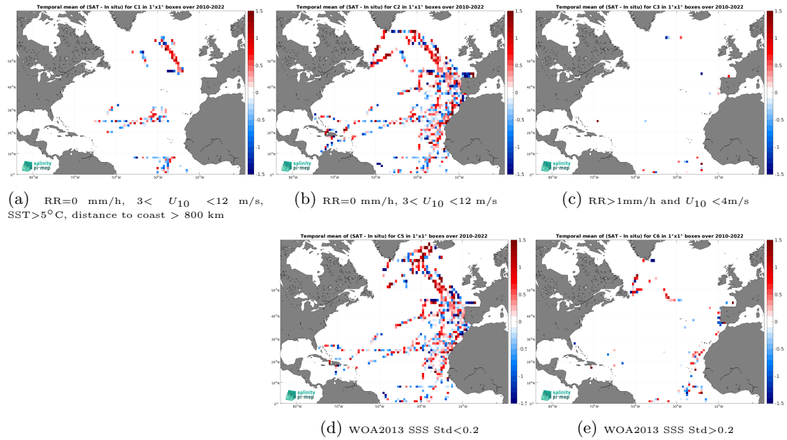
Figure 12: Temporal mean gridded over spatial boxes of size 1^\circ \times 1^\circ of \Delta SSS (SMOS SSS L2Q v331 - No FLAG (CMEMS-CATDS-CPDC) - TSG (CSIC-UTM)) for 5 different subdatasets corresponding to:RR=0 mm/h, 3 < U_{10} < 12 m/s, SST >5^\circ\text{C} , distance to coast > 800 km (a), RR=0 mm/h, 3 < U_{10} < 12 m/s (b), RR >1 mm/h and U_{10} < 4 m/s (c), WOA2013 SSS Std <0.2 (d), WOA2013 SSS Std >0.2 (e).
