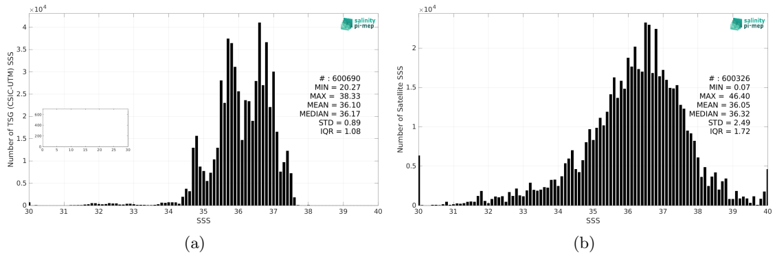
Figure 2: Histograms of SSS from TSG (CSIC-UTM) (a) and SMOS SSS L2Q v331 - No FLAG (CMEMS-CATDS-CPDC) (b) considering all match-up pairs per bins of 0.1 over the North Atlantic Ocean Pi-MEP region and for the full satellite product period.
