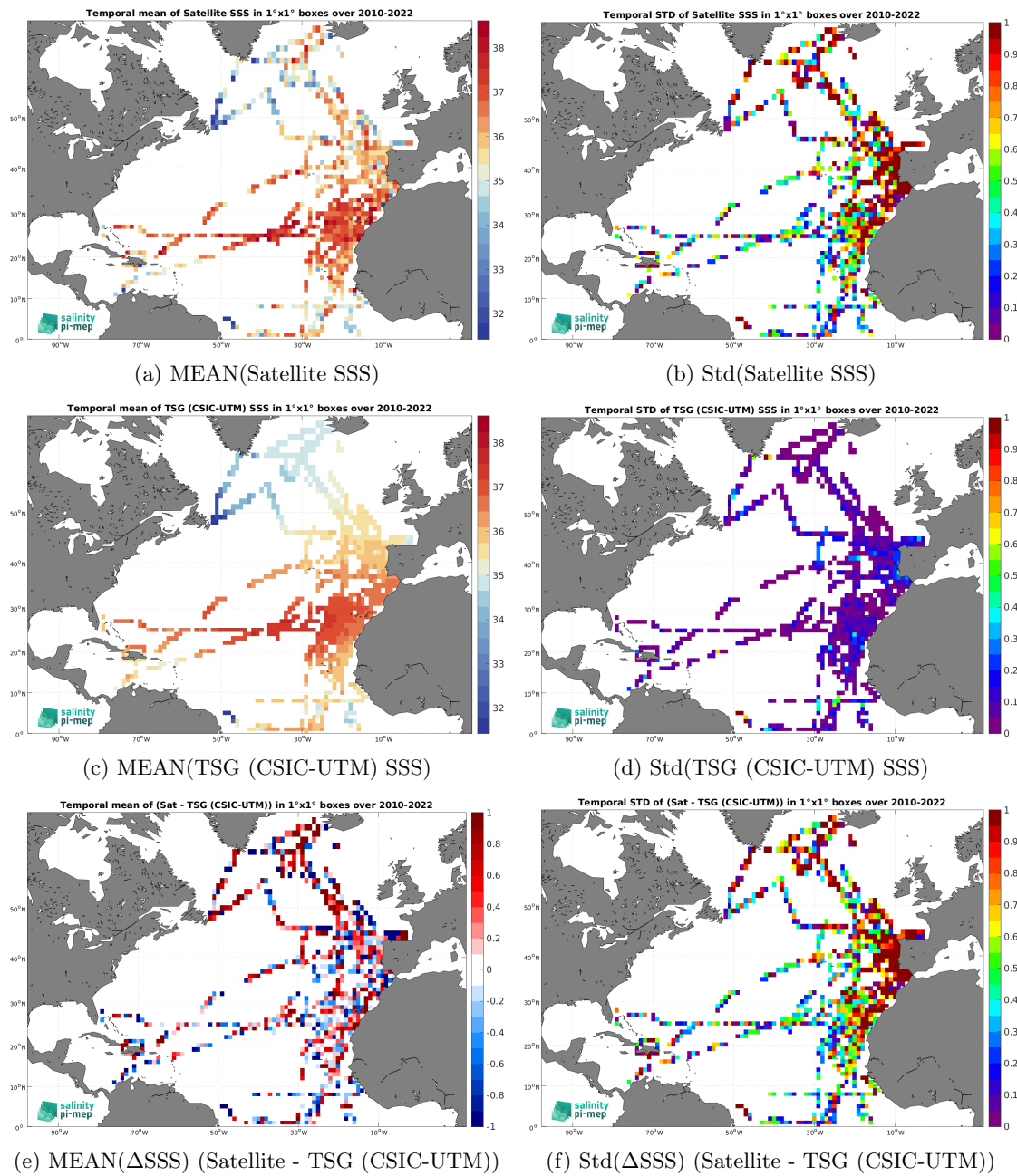
Figure 6: Temporal mean (left) and Std (right) of SSS from SMOS SSS L2Q v331 - No FLAG (CMEMS-CATDS-CPDC) (top), TSG (CSIC-UTM) (middle), and of \Delta SSS (Satellite - TSG (CSIC-UTM)). Only match-up pairs are used to generate these maps.
