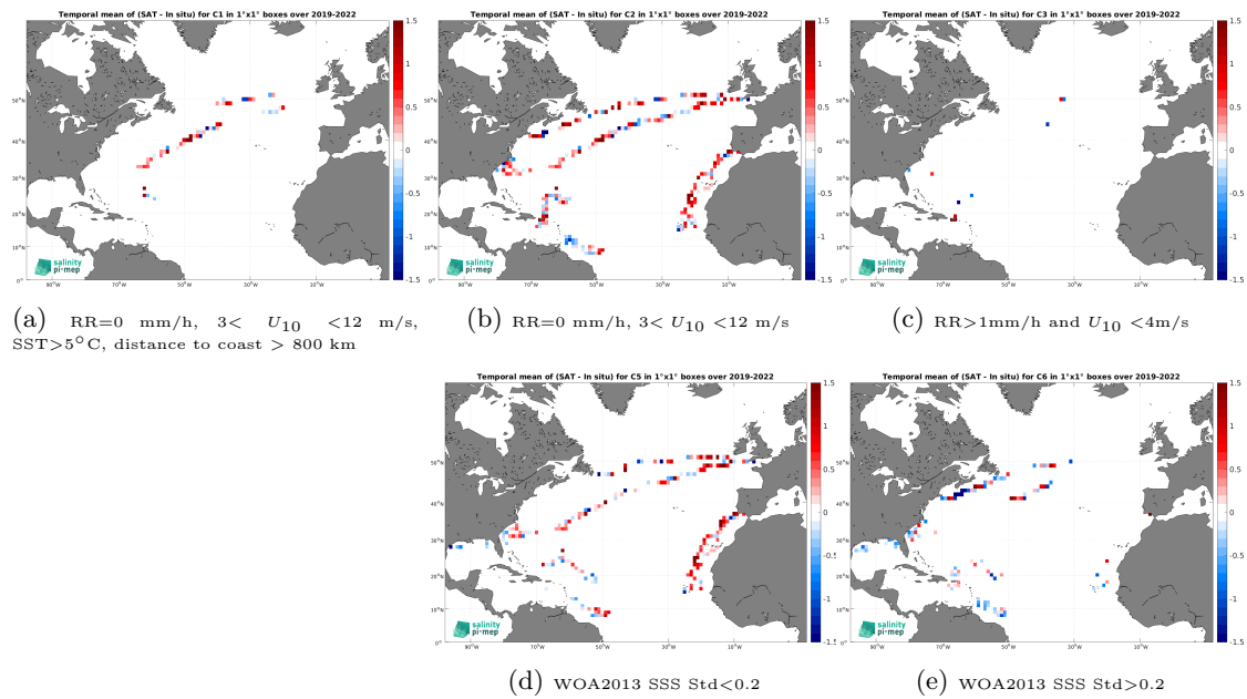
Figure 14: Temporal mean gridded over spatial boxes of size 1^\circ \times 1^\circ of \Delta\text{SSS} (SMOS SSS L2Q v331 - No FLAG (CMEMS-CATDS-CPDC) - Saildrone) for 5 different subdatasets corresponding to:RR=0 mm/h, 3 < U_{10} < 12 m/s, SST>5°C, distance to coast > 800 km (a), RR=0 mm/h, 3 < U_{10} < 12 m/s (b), RR>1mm/h and U_{10} < 4 m/s (c), WOA2013 SSS Std<0.2 (d), WOA2013 SSS Std>0.2 (e).
