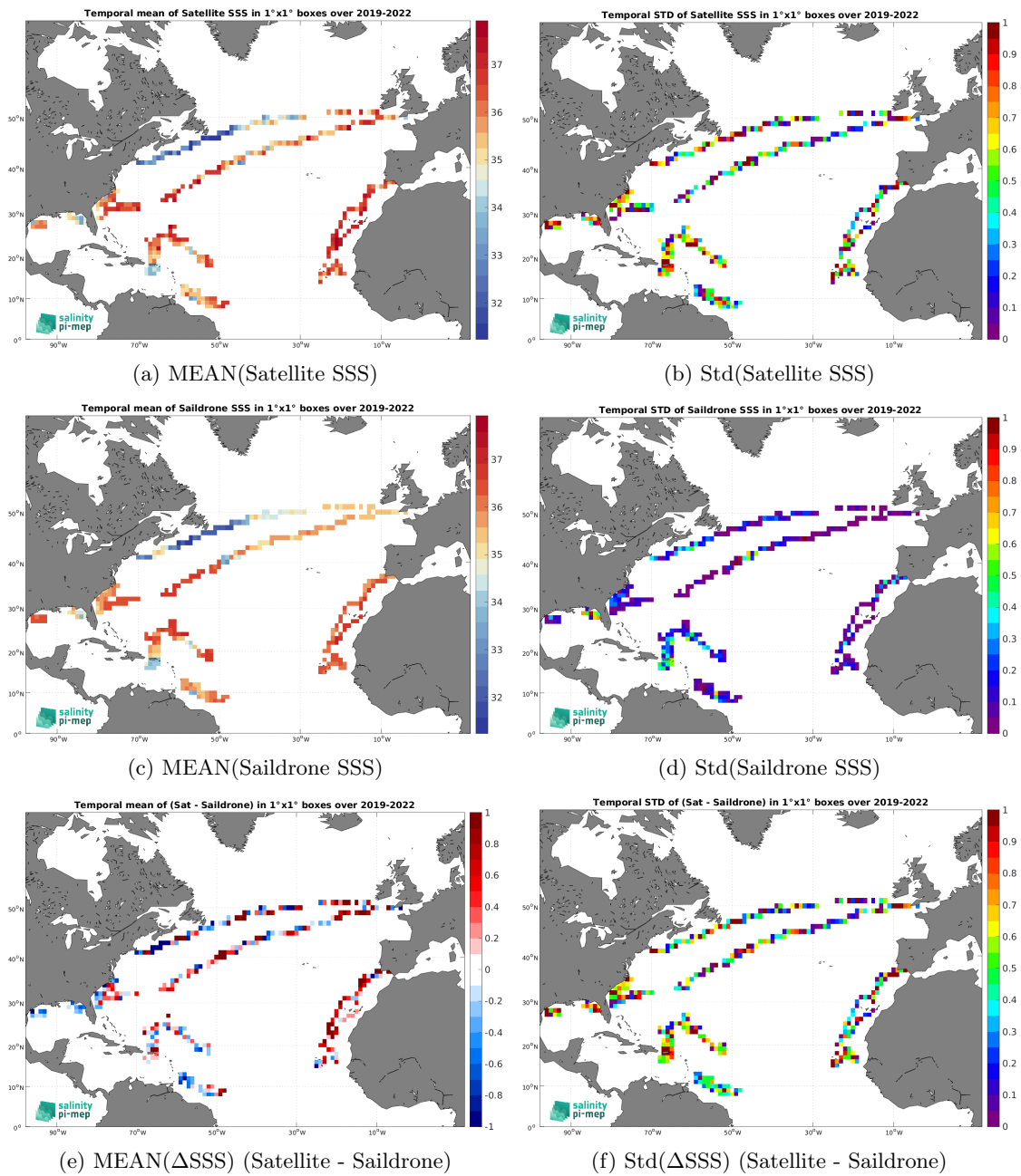
Figure 7: Temporal mean (left) and Std (right) of SSS from SMOS SSS L2Q v331 - No FLAG (CMEMS-CATDS-CPDC) (top), Saildrone (middle), and of \Delta SSS (Satellite - Saildrone). Only match-up pairs are used to generate these maps.
