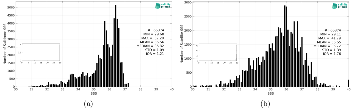
Figure 3: Histograms of SSS from Saildrone (a) and SMOS SSS L2Q v331 - No FLAG (CMEMS-CATDS-CPDC) (b) considering all match-up pairs per bins of 0.1 over the North Atlantic Ocean Pi-MEP region and for the full satellite product period.
