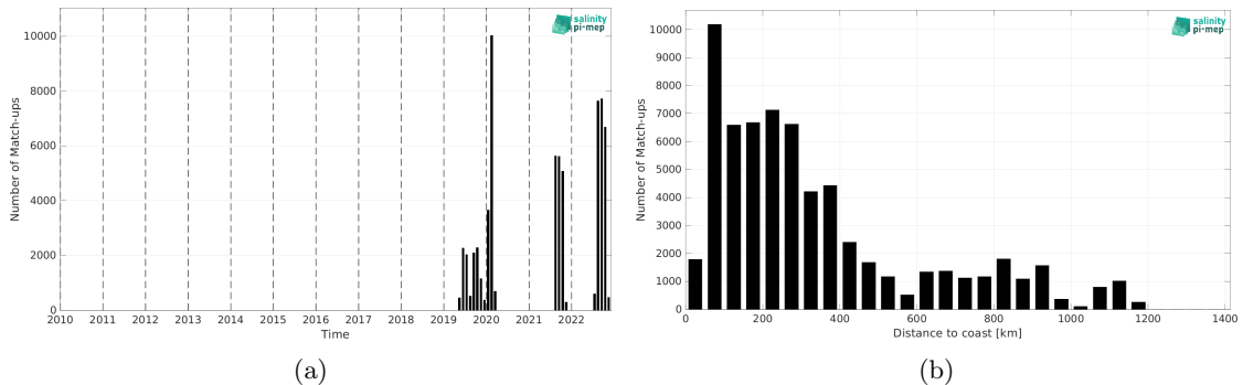
Figure 2: Number of match-ups between Saildrone and SMOS SSS L2Q v331 - No FLAG (CMEMS-CATDS-CPDC) SSS as a function of time (a) and as function of the distance to coast (b) over the North Atlantic Ocean Pi-MEP region and for the full satellite product period.
