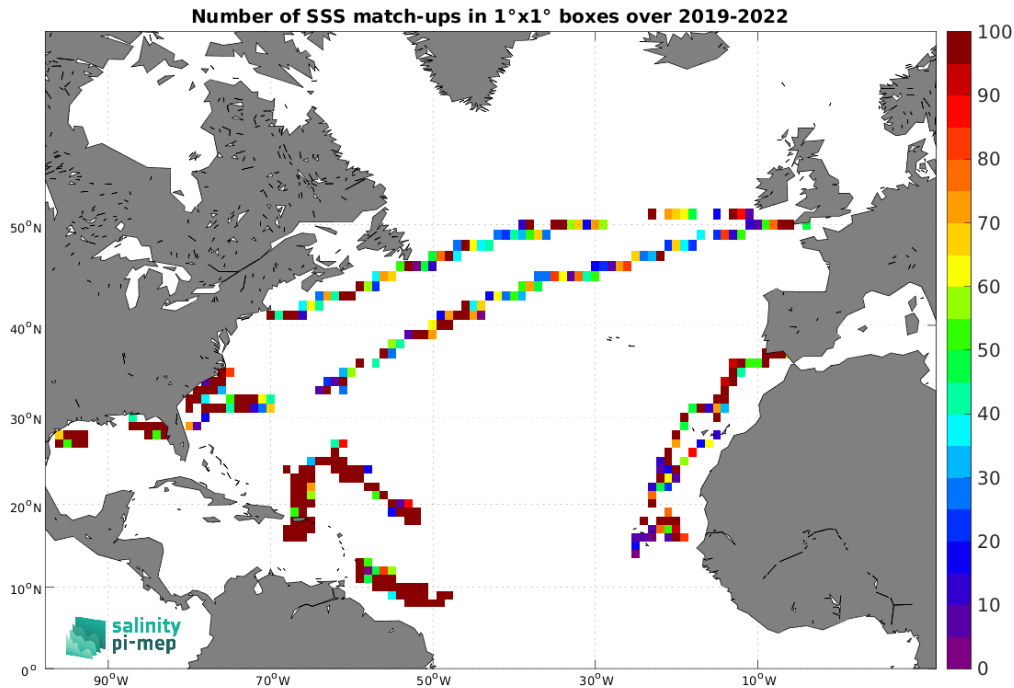
Figure 4: Number of SSS match-ups between Saildrone SSS and the SMOS SSS L2Q v331 - No FLAG (CMEMS-CATDS-CPDC) SSS product for the North Atlantic Ocean Pi-MEP region over 1^\circ \times 1^\circ boxes and for the full satellite product period.
