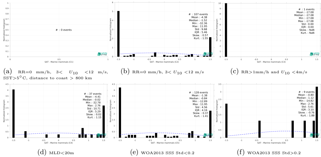
Figure 15: Normalized histogram of \Delta\text{SSS} (SMOS SSS L2Q v331 - No FLAG (CMEMS-CATDS-CPDC) - Marine mammals) for 6 different subdatasets corresponding to: RR=0 mm/h, 3 < U_{10} < 12 m/s, SST > 5^{\circ}\text{C} , distance to coast > 800 km (a), RR=0 mm/h, 3 < U_{10} < 12 m/s (b), RR > 1\text{mm/h} and U_{10} < 4\text{m/s} (c), MLD < 20\text{m} (d), WOA2013 SSS Std < 0.2 (e), WOA2013 SSS Std > 0.2 (f).
