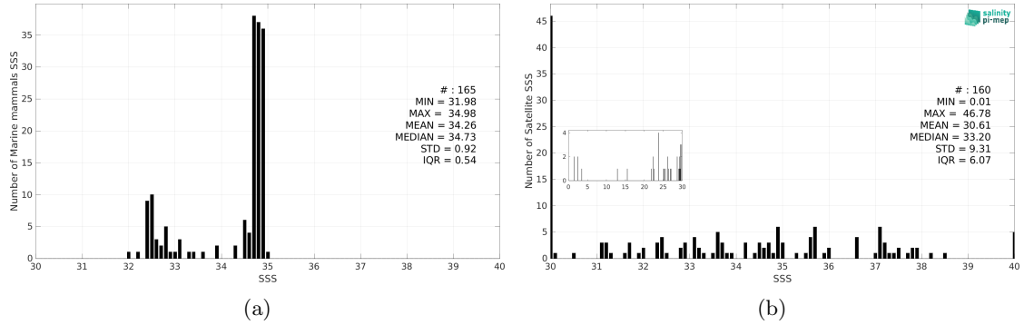
Figure 3: Histograms of SSS from Marine mammals (a) and SMOS SSS L2Q v331 - No FLAG (CMEMS-CATDS-CPDC) (b) considering all match-up pairs per bins of 0.1 over the North Atlantic Ocean Pi-MEP region and for the full satellite product period.
