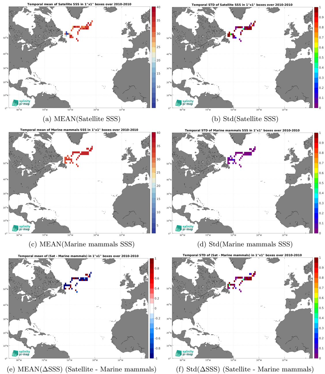
Figure 7: Temporal mean (left) and Std (right) of SSS from SMOS SSS L2Q v331 - No FLAG (CMEMS-CATDS-CPDC) (top), Marine mammals (middle), and of \Delta SSS (Satellite - Marine mammals). Only match-up pairs are used to generate these maps.
