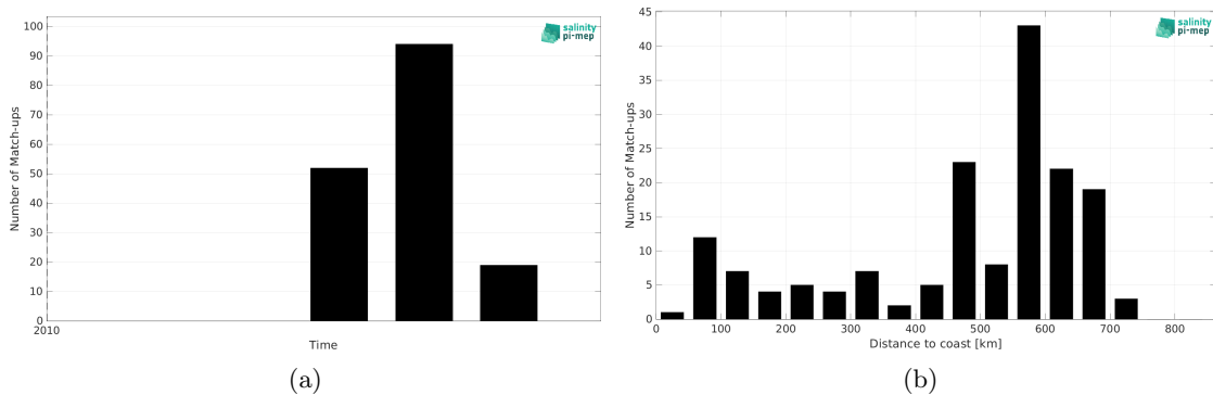
Figure 2: Number of match-ups between Marine mammals and SMOS SSS L2Q v331 - No FLAG (CMEMS-CATDS-CPDC) SSS as a function of time (a) and as function of the distance to coast (b) over the North Atlantic Ocean Pi-MEP region and for the full satellite product period.
