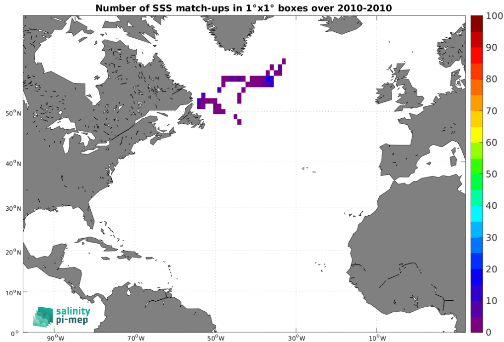
Figure 5: Number of SSS match-ups between Marine mammals SSS and the SMOS SSS L2Q v331 - No FLAG (CMEMS-CATDS-CPDC) SSS product for the North Atlantic Ocean Pi-MEP region over 1^\circ \times 1^\circ boxes and for the full satellite product period.
