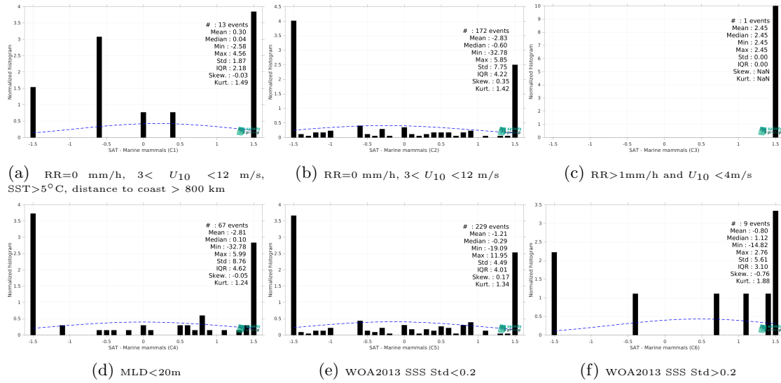
Figure 13: Normalized histogram of \Delta SSS (SMOS SSS L2Q v331 - No FLAG (CMEMS-CATDS-CPDC) - Marine mammals) for 6 different subdatasets corresponding to: RR=0 mm/h, 3 < U_{10} < 12 m/s, SST > 5°C, distance to coast > 800 km (a), RR=0 mm/h, 3 < U_{10} < 12 m/s (b), RR > 1mm/h and U_{10} < 4 m/s (c), MLD < 20m (d), WOA2013 SSS Std < 0.2 (e), WOA2013 SSS Std > 0.2 (f).
