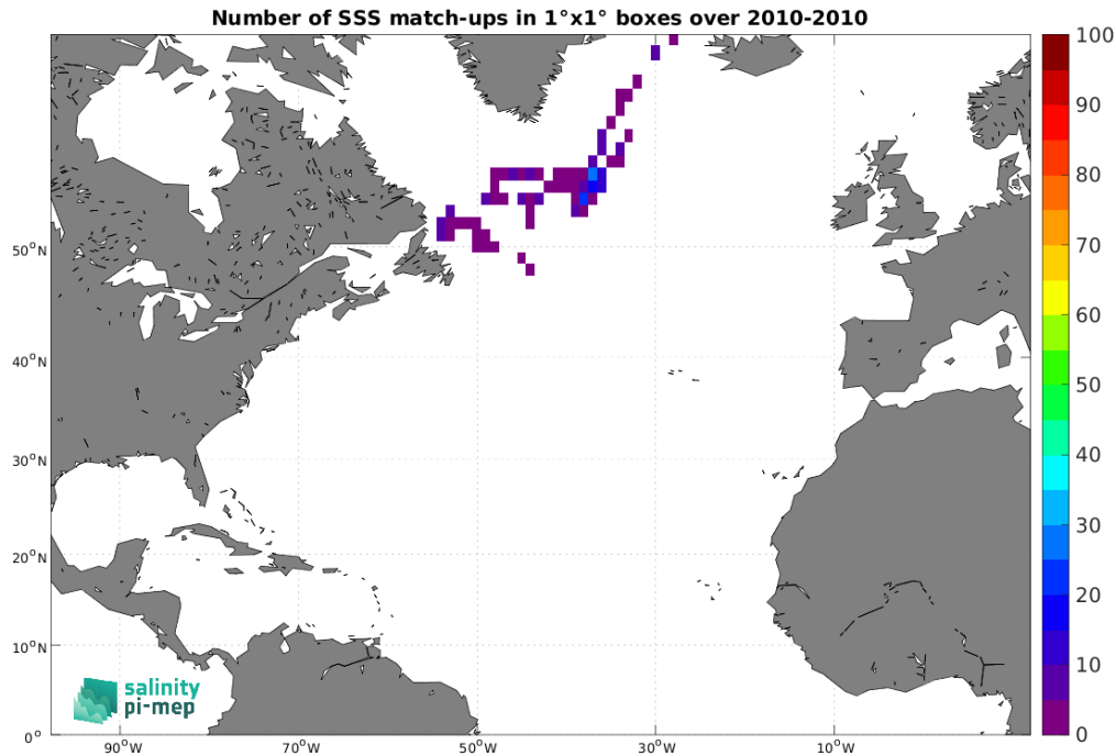
Figure 4: Number of SSS match-ups between Marine mammals SSS and the SMOS SSS L2Q v331 - No FLAG (CMEMS-CATDS-CPDC) SSS product for the North Atlantic Ocean Pi-MEP region over 1^\circ \times 1^\circ boxes and for the full satellite product period.
