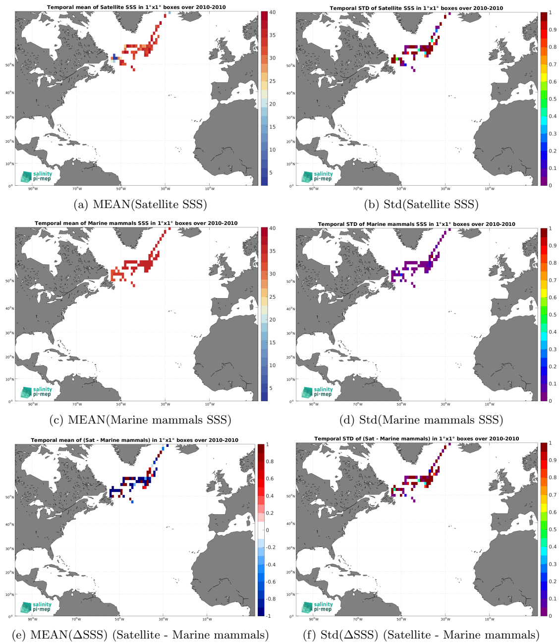
Figure 6: Temporal mean (left) and Std (right) of SSS from SMOS SSS L2Q v331 - No FLAG (CMEMS-CATDS-CPDC) (top), Marine mammals (middle), and of \Delta SSS (Satellite - Marine mammals). Only match-up pairs are used to generate these maps.
