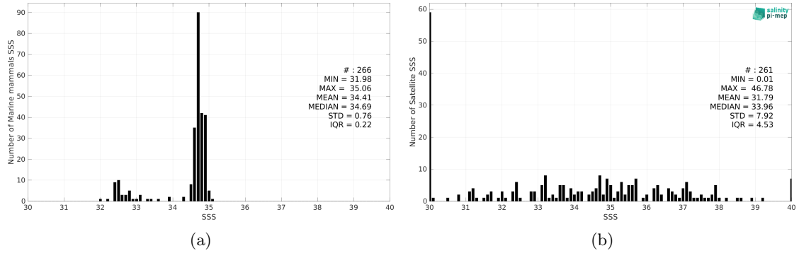
Figure 2: Histograms of SSS from Marine mammals (a) and SMOS SSS L2Q v331 - No FLAG (CMEMS-CATDS-CPDC) (b) considering all match-up pairs per bins of 0.1 over the North Atlantic Ocean Pi-MEP region and for the full satellite product period.
