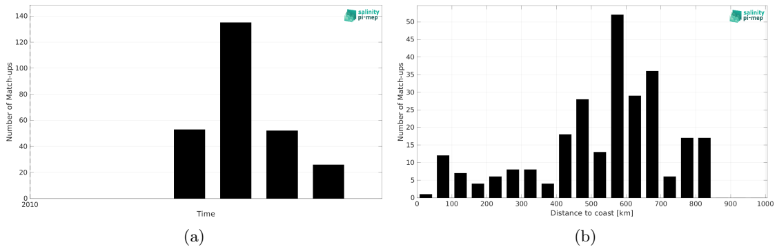
Figure 1: Number of match-ups between Marine mammals and SMOS SSS L2Q v331 - No FLAG (CMEMS-CATDS-CPDC) SSS as a function of time (a) and as function of the distance to coast (b) over the North Atlantic Ocean Pi-MEP region and for the full satellite product period.
