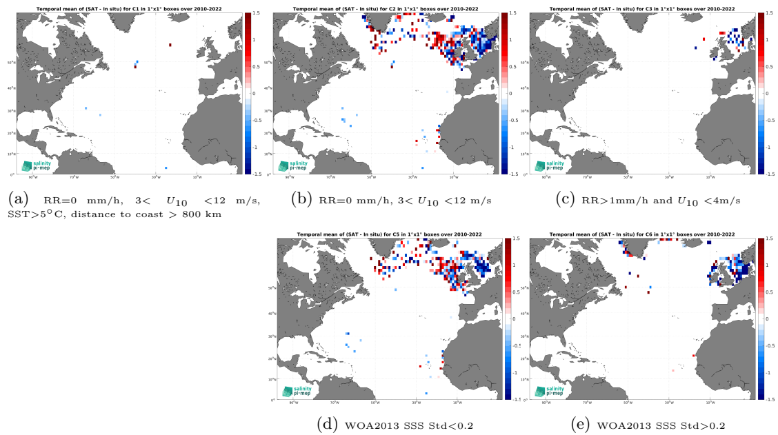
Figure 14: Temporal mean gridded over spatial boxes of size 1^\circ \times 1^\circ of \Delta\text{SSS} (SMOS SSS L2Q v331 - No FLAG (CMEMS-CATDS-CPDC) - ICES) for 5 different subdatasets corresponding to:RR=0 mm/h, 3 < U_{10} < 12 m/s, SST >5^\circ\text{C} , distance to coast > 800 km (a), RR=0 mm/h, 3 < U_{10} < 12 m/s (b), RR >1 mm/h and U_{10} < 4 m/s (c), WOA2013 SSS Std <0.2 (d), WOA2013 SSS Std >0.2 (e).
