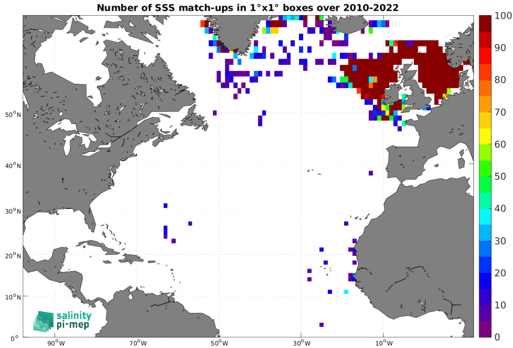
Figure 5: Number of SSS match-ups between ICES SSS and the SMOS SSS L2Q v331 - No FLAG (CMEMS-CATDS-CPDC) SSS product for the North Atlantic Ocean Pi-MEP region over 1^\circ \times 1^\circ boxes and for the full satellite product period.
