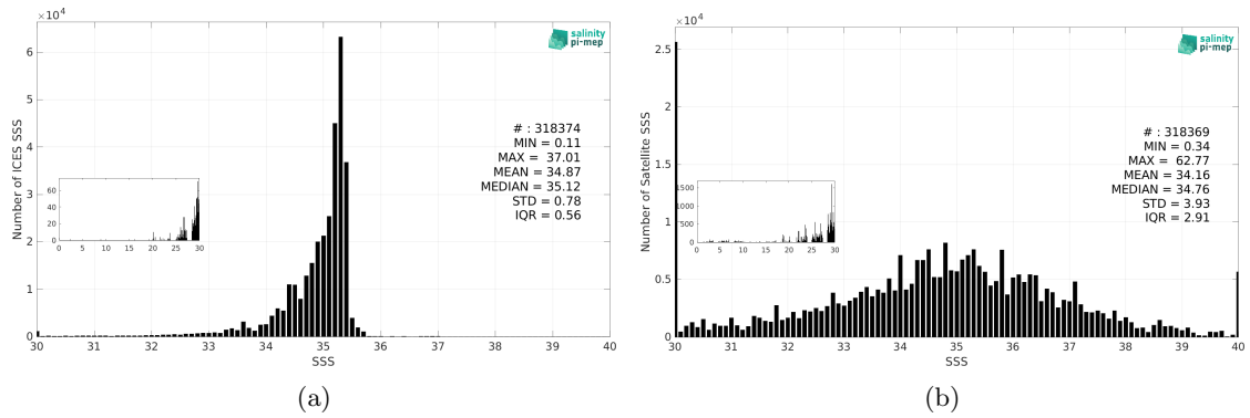
Figure 3: Histograms of SSS from ICES (a) and SMOS SSS L2Q v331 - No FLAG (CMEMS-CATDS-CPDC) (b) considering all match-up pairs per bins of 0.1 over the North Atlantic Ocean Pi-MEP region and for the full satellite product period.
