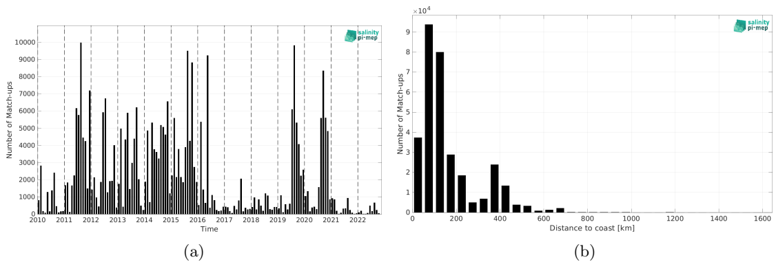
Figure 2: Number of match-ups between ICES and SMOS SSS L2Q v331 - No FLAG (CMEMS-CATDS-CPDC) SSS as a function of time (a) and as function of the distance to coast (b) over the North Atlantic Ocean Pi-MEP region and for the full satellite product period.
