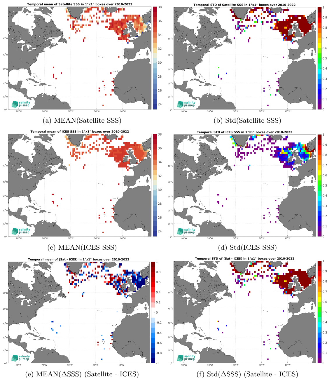
Figure 7: Temporal mean (left) and Std (right) of SSS from SMOS SSS L2Q v331 - No FLAG (CMEMS-CATDS-CPDC) (top), ICES (middle), and of \Delta SSS (Satellite - ICES). Only match-up pairs are used to generate these maps.
