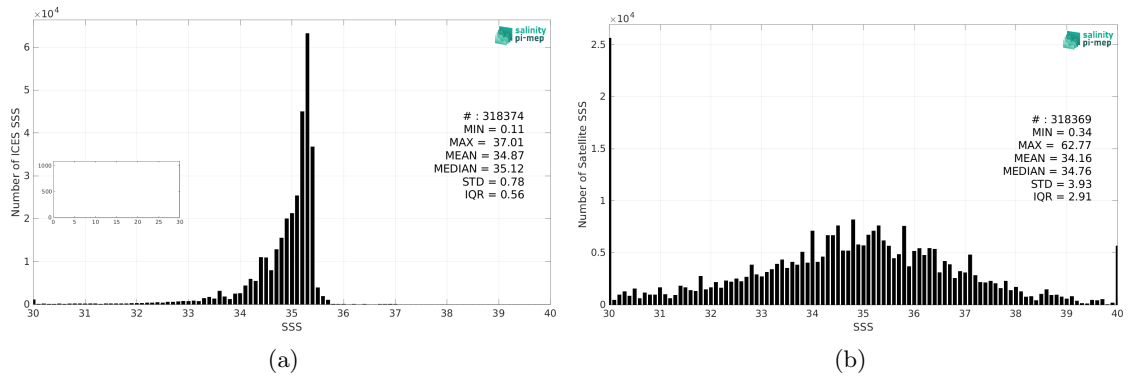
Figure 2: Histograms of SSS from ICES (a) and SMOS SSS L2Q v331 - No FLAG (CMEMS-CATDS-CPDC) (b) considering all match-up pairs per bins of 0.1 over the North Atlantic Ocean Pi-MEP region and for the full satellite product period.
