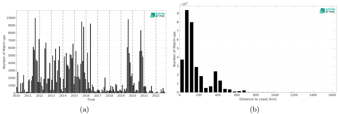
Figure 1: Number of match-ups between ICES and SMOS SSS L2Q v331 - No FLAG (CMEMS-CATDS-CPDC) SSS as a function of time (a) and as function of the distance to coast (b) over the North Atlantic Ocean Pi-MEP region and for the full satellite product period.
