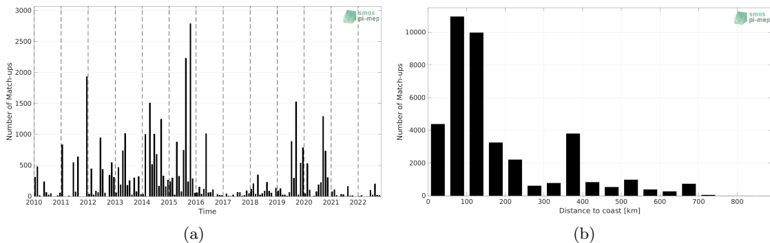
Figure 1: Number of match-ups between ICES and SMOS SSS L2Q v331 - No FLAG (CMEMS-CATDS-CPDC) SSS as a function of time (a) and as function of the distance to coast (b) over the North Atlantic Ocean Pi-MEP region and for the full satellite product period.
