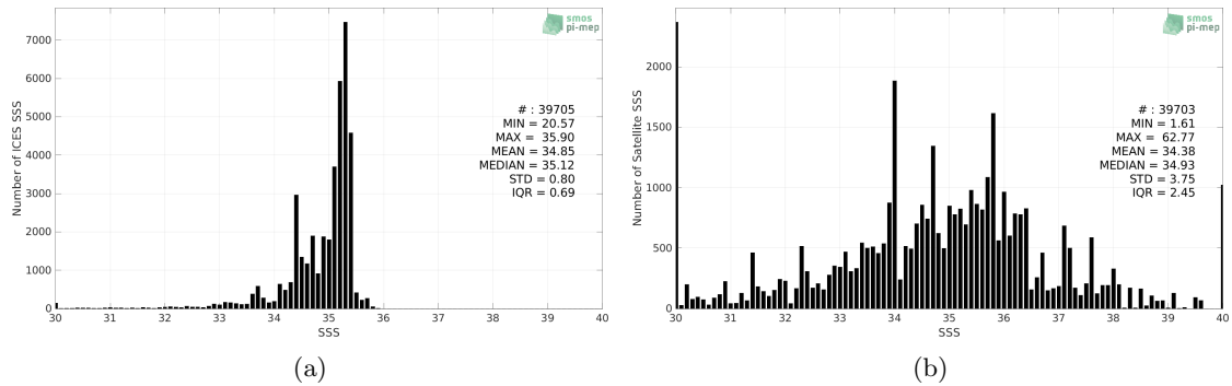
Figure 2: Histograms of SSS from ICES (a) and SMOS SSS L2Q v331 - No FLAG (CMEMS-CATDS-CPDC) (b) considering all match-up pairs per bins of 0.1 over the North Atlantic Ocean Pi-MEP region and for the full satellite product period.
