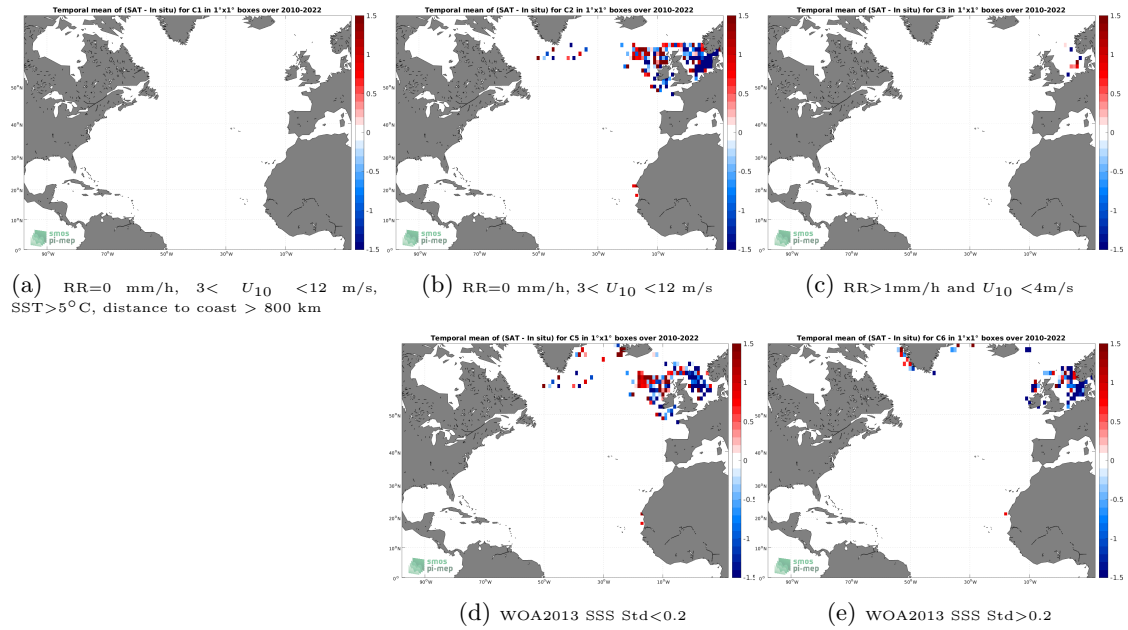
Figure 12: Temporal mean gridded over spatial boxes of size 1^\circ \times 1^\circ of \Delta\text{SSS} (SMOS SSS L2Q v331 - No FLAG (CMEMS-CATDS-CPDC) - ICES) for 5 different subdatasets corresponding to:RR=0 mm/h, 3 < U_{10} < 12 m/s, SST >5^\circ\text{C} , distance to coast > 800 km (a), RR=0 mm/h, 3 < U_{10} < 12 m/s (b), RR >1 mm/h and U_{10} < 4 m/s (c), WOA2013 SSS Std <0.2 (d), WOA2013 SSS Std >0.2 (e).
