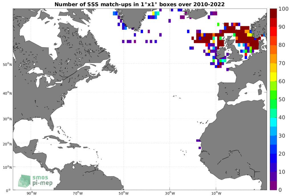
Figure 4: Number of SSS match-ups between ICES SSS and the SMOS SSS L2Q v331 - No FLAG (CMEMS-CATDS-CPDC) SSS product for the North Atlantic Ocean Pi-MEP region over 1^\circ \times 1^\circ boxes and for the full satellite product period.
