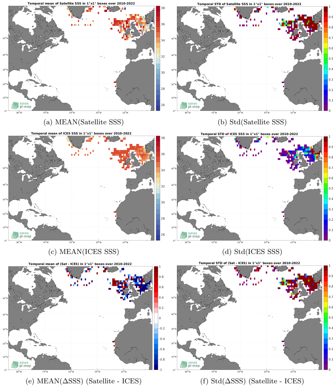
Figure 6: Temporal mean (left) and Std (right) of SSS from SMOS SSS L2Q v331 - No FLAG (CMEMS-CATDS-CPDC) (top), ICES (middle), and of \Delta SSS (Satellite - ICES). Only match-up pairs are used to generate these maps.
