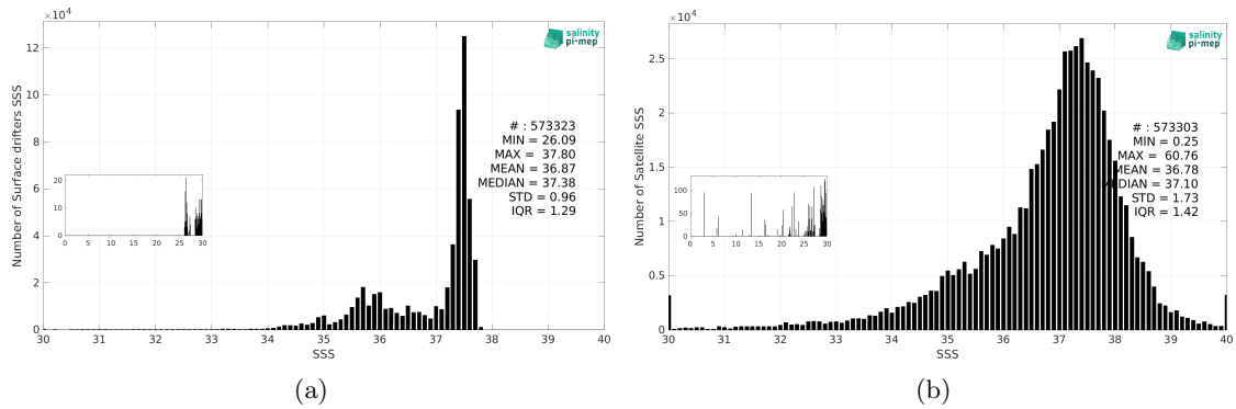
Figure 3: Histograms of SSS from Surface drifters (a) and SMOS SSS L2Q v331 - No FLAG (CMEMS-CATDS-CPDC) (b) considering all match-up pairs per bins of 0.1 over the North Atlantic Ocean Pi-MEP region and for the full satellite product period.
