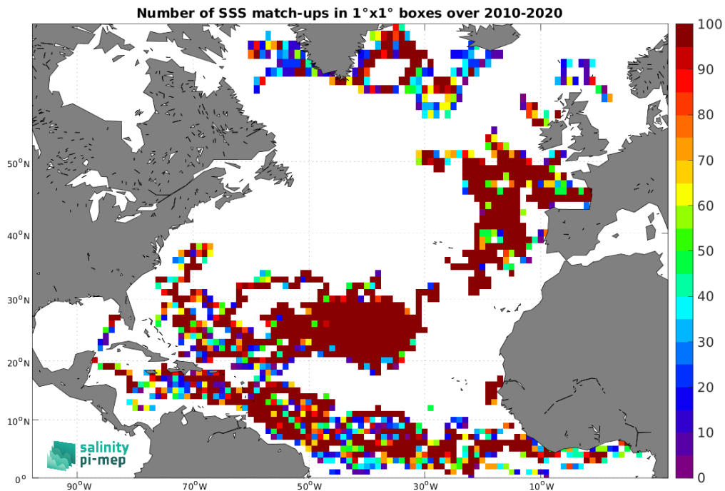
Figure 4: Number of SSS match-ups between Surface drifters SSS and the SMOS SSS L2Q v331 - No FLAG (CMEMS-CATDS-CPDC) SSS product for the North Atlantic Ocean Pi-MEP region over 1^\circ \times 1^\circ boxes and for the full satellite product period.
