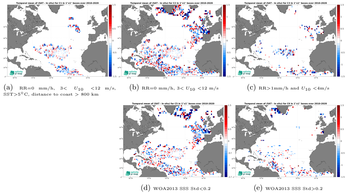
Figure 13: Temporal mean gridded over spatial boxes of size 1^\circ \times 1^\circ of \Delta\text{SSS} (SMOS SSS L2Q v331 - No FLAG (CMEMS-CATDS-CPDC) - Surface drifters) for 5 different subdatasets corresponding to:RR=0 mm/h, 3 < U_{10} < 12 m/s, SST >5^\circ\text{C} , distance to coast > 800 km (a), RR=0 mm/h, 3 < U_{10} < 12 m/s (b), RR >1 mm/h and U_{10} < 4 m/s (c), WOA2013 SSS Std <0.2 (d), WOA2013 SSS Std >0.2 (e).
