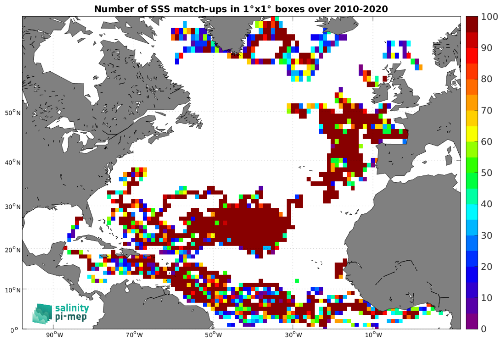
Figure 3: Number of SSS match-ups between Surface drifters SSS and the SMOS SSS L2Q v331 - No FLAG (CMEMS-CATDS-CPDC) SSS product for the North Atlantic Ocean Pi-MEP region over 1^\circ \times 1^\circ boxes and for the full satellite product period.
