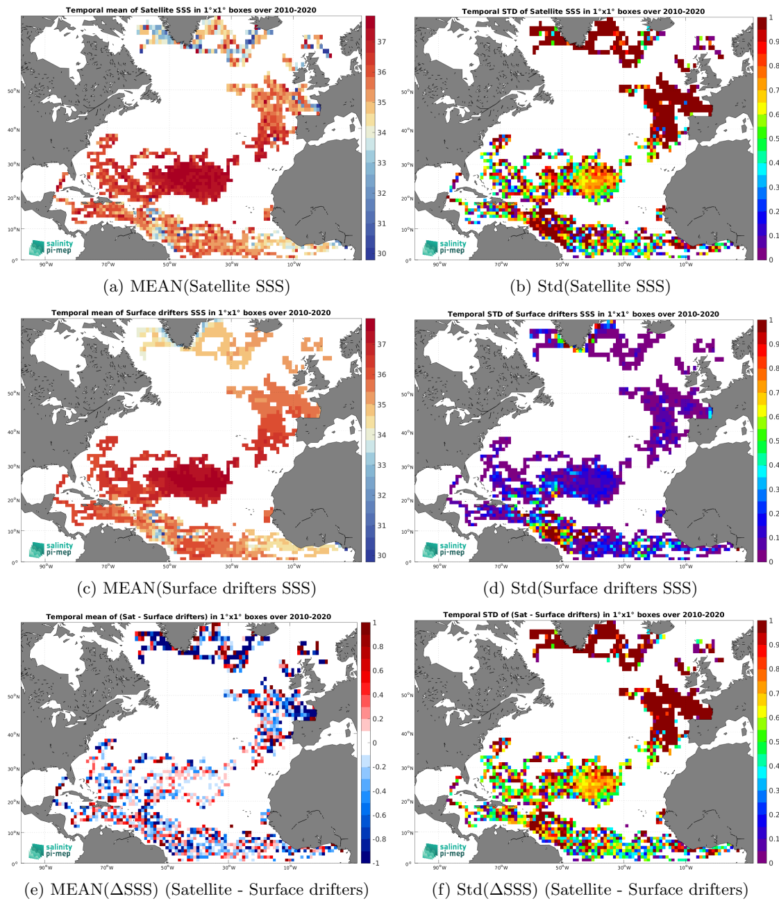
Figure 5: Temporal mean (left) and Std (right) of SSS from SMOS SSS L2Q v331 - No FLAG (CMEMS-CATDS-CPDC) (top), Surface drifters (middle), and of \Delta SSS (Satellite - Surface drifters). Only match-up pairs are used to generate these maps.
