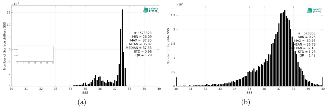
Figure 2: Histograms of SSS from Surface drifters (a) and SMOS SSS L2Q v331 - No FLAG (CMEMS-CATDS-CPDC) (b) considering all match-up pairs per bins of 0.1 over the North Atlantic Ocean Pi-MEP region and for the full satellite product period.
