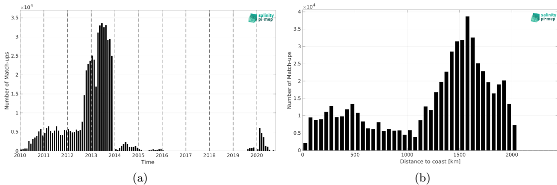
Figure 1: Number of match-ups between Surface drifters and SMOS SSS L2Q v331 - No FLAG (CMEMS-CATDS-CPDC) SSS as a function of time (a) and as function of the distance to coast (b) over the North Atlantic Ocean Pi-MEP region and for the full satellite product period.
