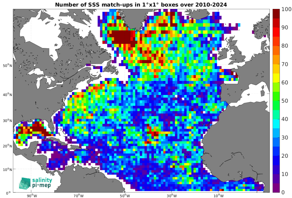
Figure 5: Number of SSS match-ups between Argo SSS and the SMOS SSS L2Q v331 - No FLAG (CMEMS-CATDS-CPDC) SSS product for the North Atlantic Ocean Pi-MEP region over 1^\circ \times 1^\circ boxes and for the full satellite product period.
