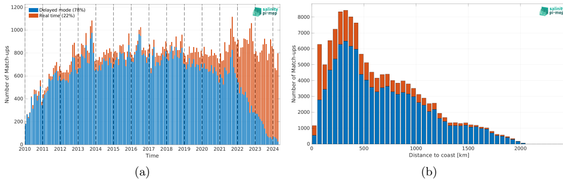
Figure 2: Number of match-ups between Argo and SMOS SSS L2Q v331 - No FLAG (CMEMS-CATDS-CPDC) SSS as a function of time (a) and as function of the distance to coast (b) over the North Atlantic Ocean Pi-MEP region and for the full satellite product period.
