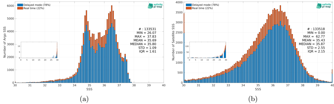
Figure 3: Histograms of SSS from Argo (a) and SMOS SSS L2Q v331 - No FLAG (CMEMS-CATDS-CPDC) (b) considering all match-up pairs per bins of 0.1 over the North Atlantic Ocean Pi-MEP region and for the full satellite product period.
