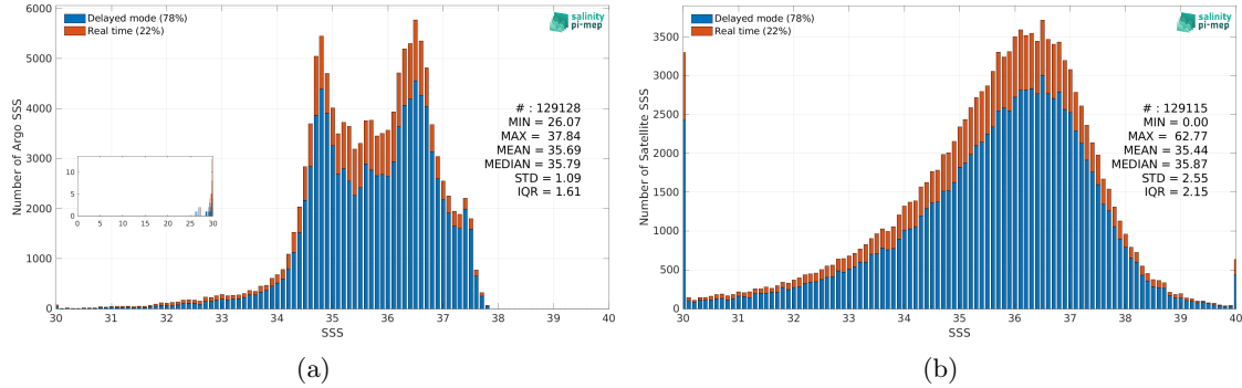
Figure 2: Histograms of SSS from Argo (a) and SMOS SSS L2Q v331 - No FLAG (CMEMS-CATDS-CPDC) (b) considering all match-up pairs per bins of 0.1 over the North Atlantic Ocean Pi-MEP region and for the full satellite product period.
