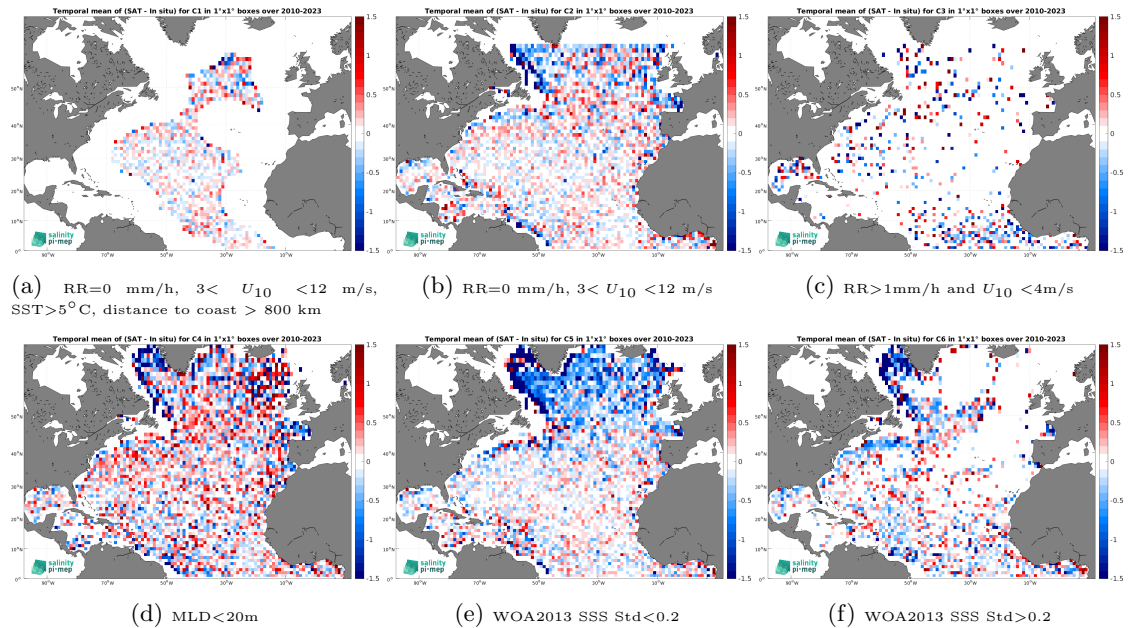
Figure 12: Temporal mean gridded over spatial boxes of size 1^\circ \times 1^\circ of \Delta SSS (SMOS SSS L2Q v331 - No FLAG (CMEMS-CATDS-CPDC) - Argo) for 6 different subdatasets corresponding to: RR=0 mm/h, 3 < U_{10} < 12 m/s, SST > 5^\circ\text{C} , distance to coast > 800 km (a), RR=0 mm/h, 3 < U_{10} < 12 m/s (b), RR > 1 mm/h and U_{10} < 4 m/s (c),MLD < 20 m (d),WOA2013 SSS Std < 0.2 (e),WOA2013 SSS Std > 0.2 (f).
