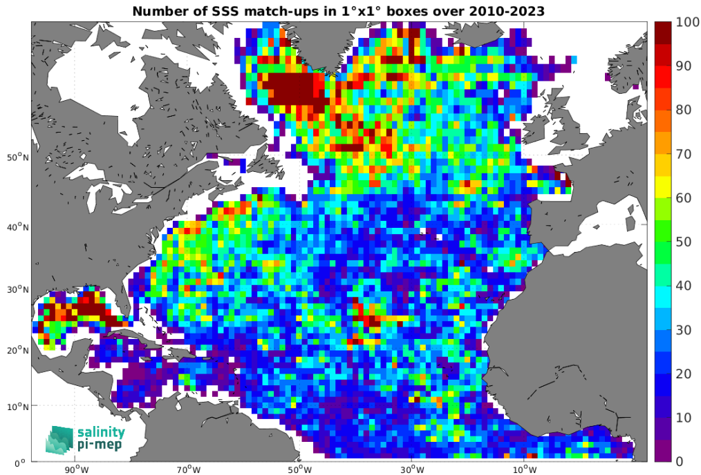
Figure 4: Number of SSS match-ups between Argo SSS and the SMOS SSS L2Q v331 - No FLAG (CMEMS-CATDS-CPDC) SSS product for the North Atlantic Ocean Pi-MEP region over 1^\circ \times 1^\circ boxes and for the full satellite product period.
