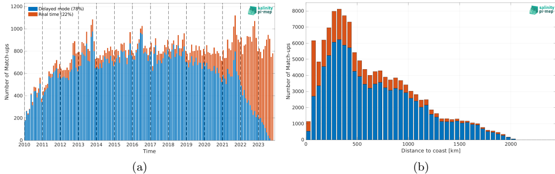
Figure 1: Number of match-ups between Argo and SMOS SSS L2Q v331 - No FLAG (CMEMS-CATDS-CPDC) SSS as a function of time (a) and as function of the distance to coast (b) over the North Atlantic Ocean Pi-MEP region and for the full satellite product period.
