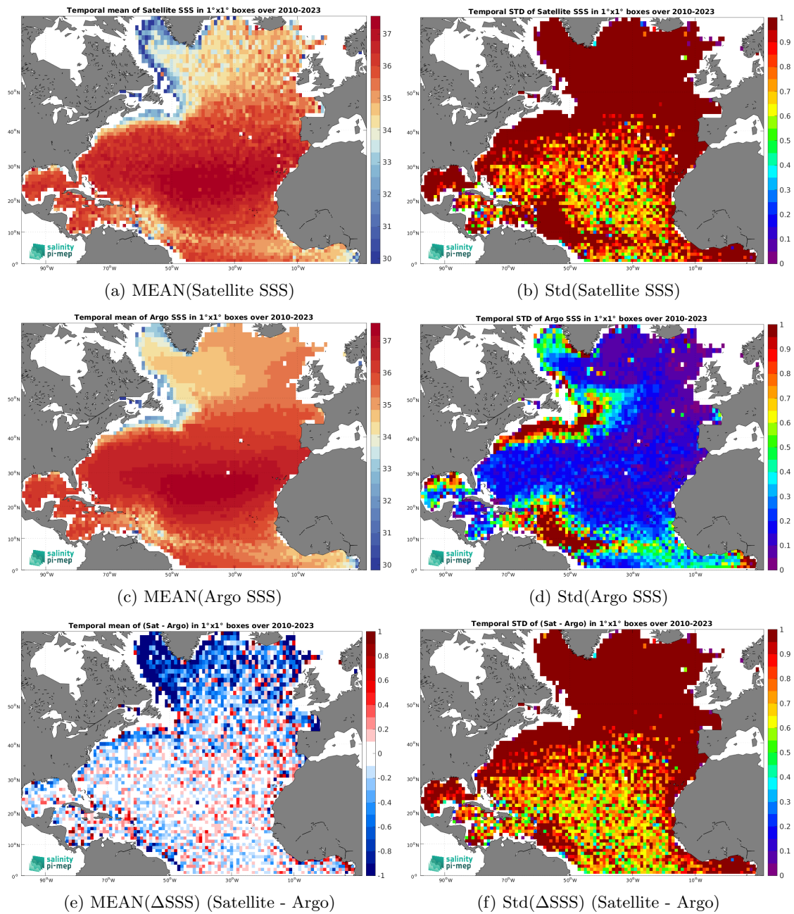
Figure 6: Temporal mean (left) and Std (right) of SSS from SMOS SSS L2Q v331 - No FLAG (CMEMS-CATDS-CPDC) (top), Argo (middle), and of \Delta SSS (Satellite - Argo). Only match-up pairs are used to generate these maps.
