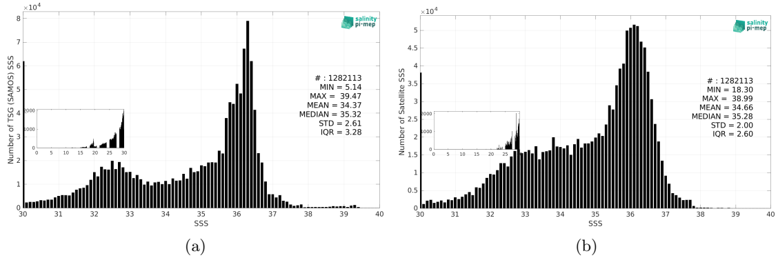
Figure 3: Histograms of SSS from TSG (SAMOS) (a) and SMOS SSS L3 v9 - 9 Days (CATDS-CEC-LOCEAN) (b) considering all match-up pairs per bins of 0.1 over the North Atlantic Ocean Pi-MEP region and for the full satellite product period.
