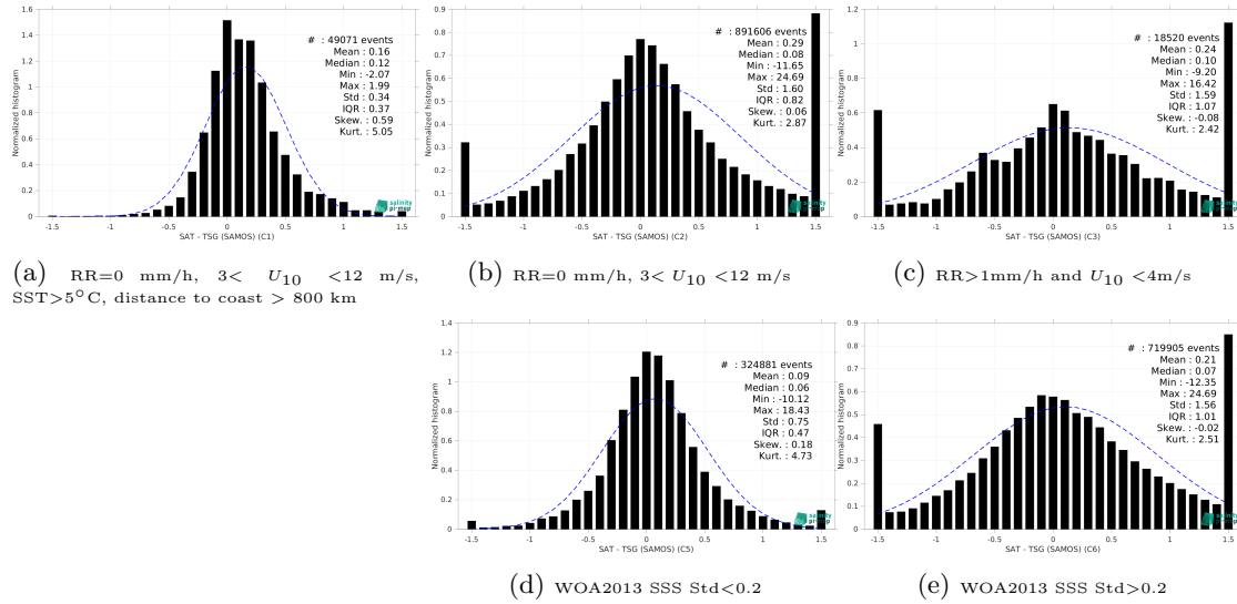
Figure 13: Normalized histogram of \Delta SSS (SMOS SSS L3 v9 - 9 Days (CATDS-CEC-LOCEAN) - TSG (SAMOS)) for 5 different subdatasets corresponding to: RR=0 mm/h, 3 < U_{10} < 12 m/s, SST > 5°C, distance to coast > 800 km (a), RR=0 mm/h, 3 < U_{10} < 12 m/s (b), RR > 1mm/h and U_{10} < 4 m/s (c), WOA2013 SSS Std < 0.2 (d), WOA2013 SSS Std > 0.2 (e).
