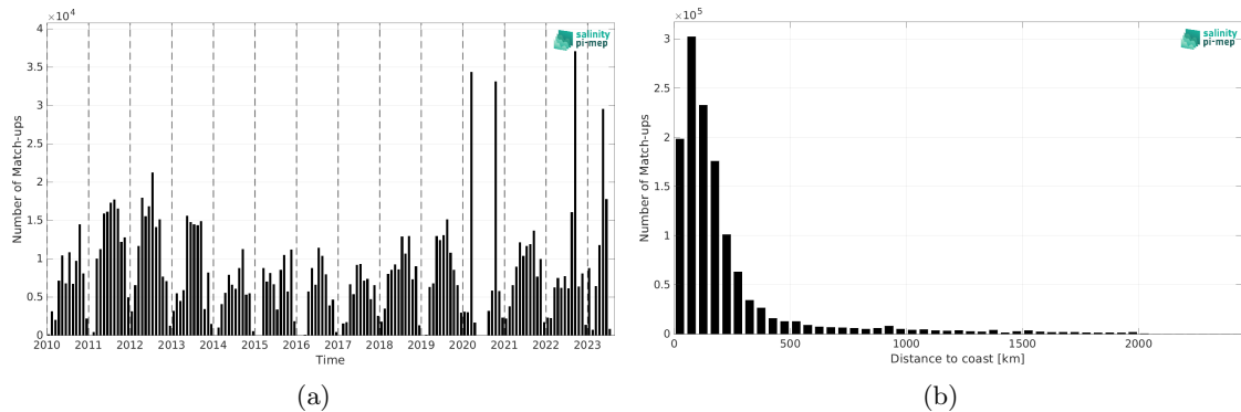
Figure 1: Number of match-ups between TSG (SAMOS) and SMOS SSS L3 v9 - 9 Days (CATDS-CEC-LOCEAN) SSS as a function of time (a) and as function of the distance to coast (b) over the North Atlantic Ocean Pi-MEP region and for the full satellite product period.
