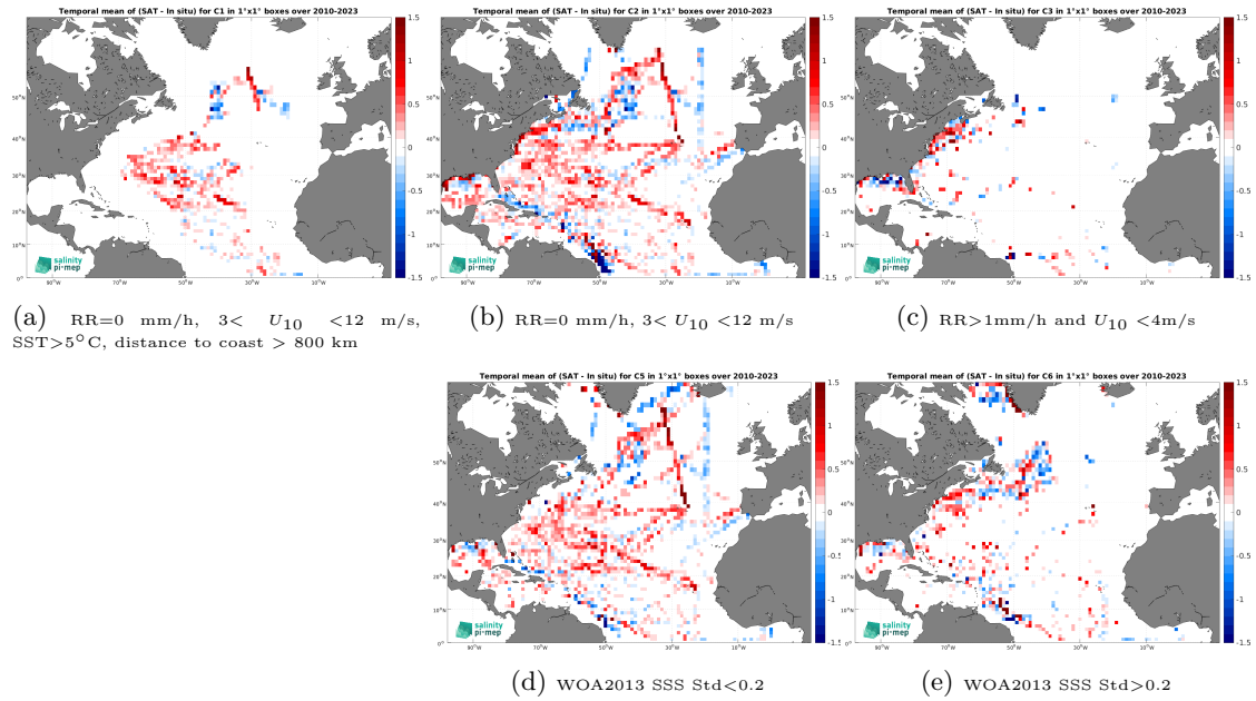
Figure 12: Temporal mean gridded over spatial boxes of size 1^\circ \times 1^\circ of \Delta SSS (SMOS SSS L3 v9 - 9 Days (CATDS-CEC-LOCEAN) - TSG (SAMOS)) for 5 different subdatasets corresponding to:RR=0 mm/h, 3 < U_{10} < 12 m/s, SST >5^\circ\text{C} , distance to coast > 800 km (a), RR=0 mm/h, 3 < U_{10} < 12 m/s (b), RR >1 mm/h and U_{10} < 4 m/s (c), WOA2013 SSS Std <0.2 (d), WOA2013 SSS Std >0.2 (e).
