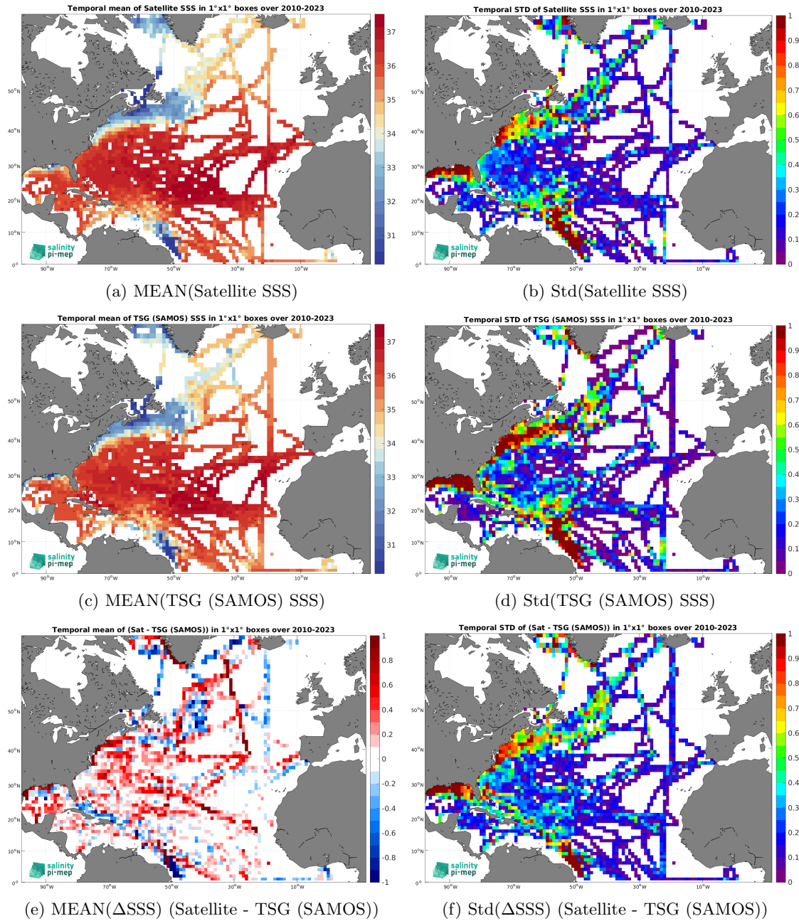
Figure 6: Temporal mean (left) and Std (right) of SSS from SMOS SSS L3 v9 - 9 Days (CATDS-CEC-LOCEAN) (top), TSG (SAMOS) (middle), and of \Delta SSS (Satellite - TSG (SAMOS)). Only match-up pairs are used to generate these maps.
