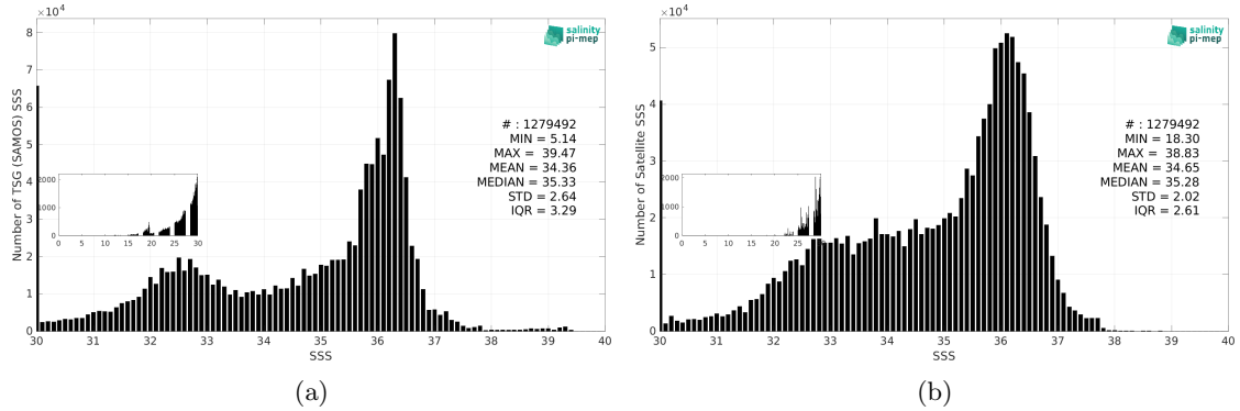
Figure 2: Histograms of SSS from TSG (SAMOS) (a) and SMOS SSS L3 v9 - 9 Days (CATDS-CEC-LOCEAN) (b) considering all match-up pairs per bins of 0.1 over the North Atlantic Ocean Pi-MEP region and for the full satellite product period.
