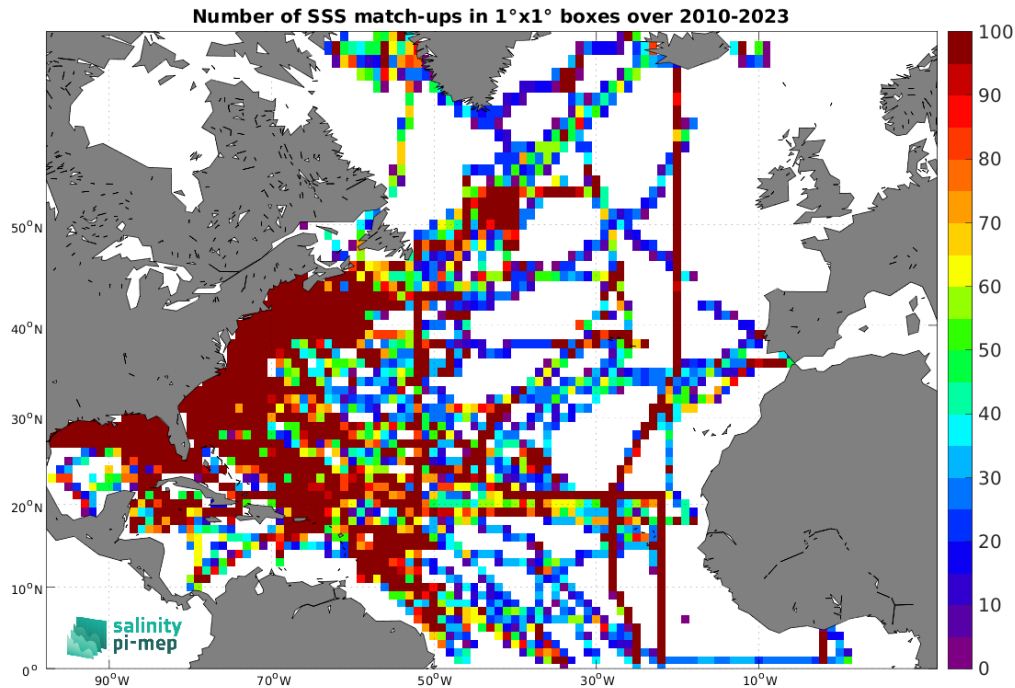
Figure 4: Number of SSS match-ups between TSG (SAMOS) SSS and the SMOS SSS L3 v9 - 9 Days (CATDS-CEC-LOCEAN) SSS product for the North Atlantic Ocean Pi-MEP region over 1^\circ \times 1^\circ boxes and for the full satellite product period.
