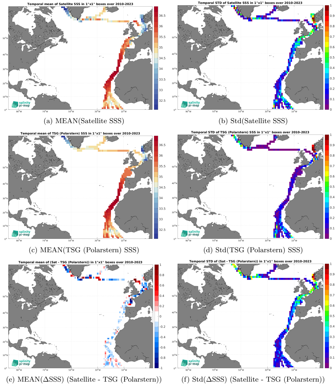
Figure 7: Temporal mean (left) and Std (right) of SSS from SMOS SSS L3 v9 - 9 Days (CATDS-CEC-LOCEAN) (top), TSG (Polarstern) (middle), and of \Delta SSS (Satellite - TSG (Polarstern)). Only match-up pairs are used to generate these maps.
