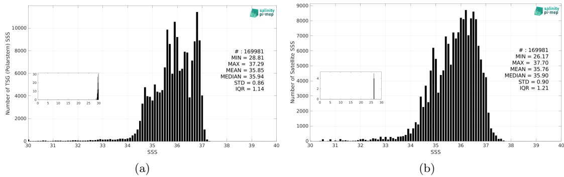
Figure 3: Histograms of SSS from TSG (Polarstern) (a) and SMOS SSS L3 v9 - 9 Days (CATDS-CEC-LOCEAN) (b) considering all match-up pairs per bins of 0.1 over the North Atlantic Ocean Pi-MEP region and for the full satellite product period.
