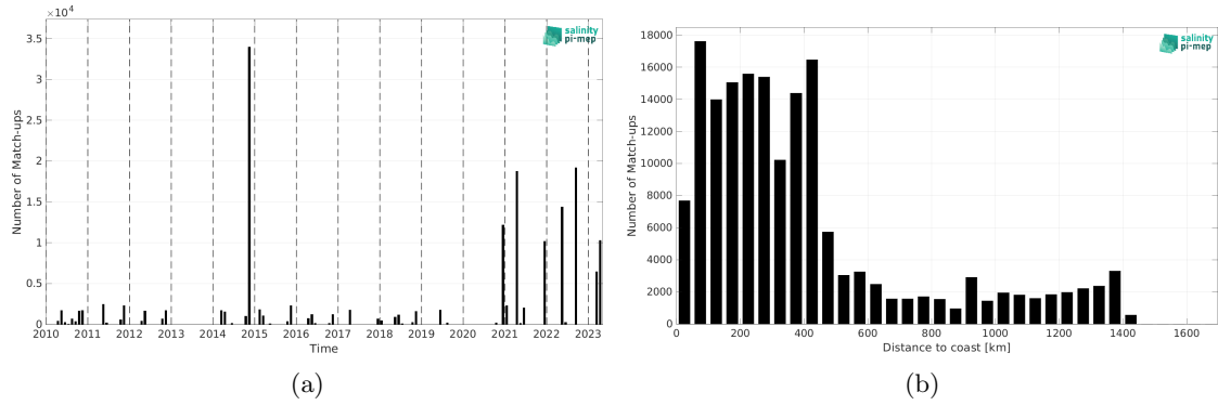
Figure 2: Number of match-ups between TSG (Polarstern) and SMOS SSS L3 v9 - 9 Days (CATDS-CEC-LOCEAN) SSS as a function of time (a) and as function of the distance to coast (b) over the North Atlantic Ocean Pi-MEP region and for the full satellite product period.
