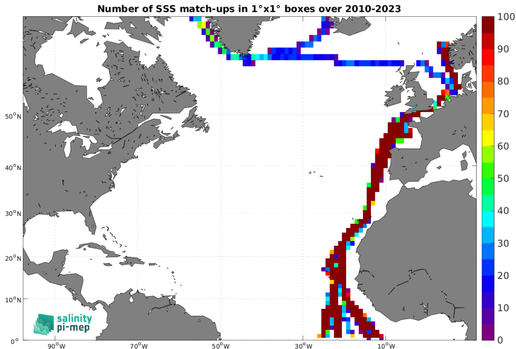
Figure 5: Number of SSS match-ups between TSG (Polarstern) SSS and the SMOS SSS L3 v9 - 9 Days (CATDS-CEC-LOCEAN) SSS product for the North Atlantic Ocean Pi-MEP region over 1^\circ \times 1^\circ boxes and for the full satellite product period.
