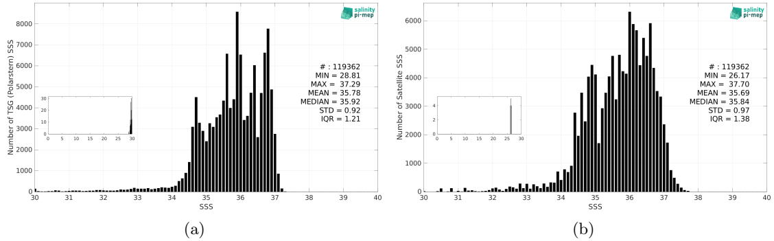
Figure 2: Histograms of SSS from TSG (Polarstern) (a) and SMOS SSS L3 v9 - 9 Days (CATDS-CEC-LOCEAN) (b) considering all match-up pairs per bins of 0.1 over the North Atlantic Ocean Pi-MEP region and for the full satellite product period.
