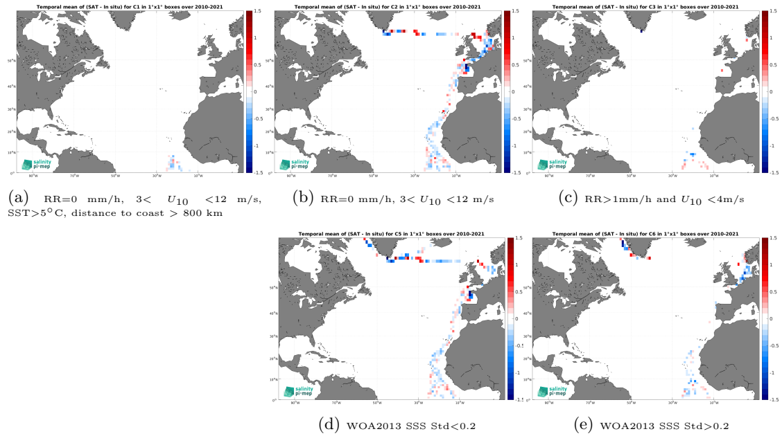
Figure 12: Temporal mean gridded over spatial boxes of size 1^\circ \times 1^\circ of \Delta\text{SSS} (SMOS SSS L3 v9 - 9 Days (CATDS-CEC-LOCEAN) - TSG (Polarstern)) for 5 different subdatasets corresponding to:RR=0 mm/h, 3 < U_{10} < 12 m/s, SST >5^\circ\text{C} , distance to coast > 800 km (a), RR=0 mm/h, 3 < U_{10} < 12 m/s (b), RR >1 mm/h and U_{10} < 4 m/s (c), WOA2013 SSS Std <0.2 (d), WOA2013 SSS Std >0.2 (e).
