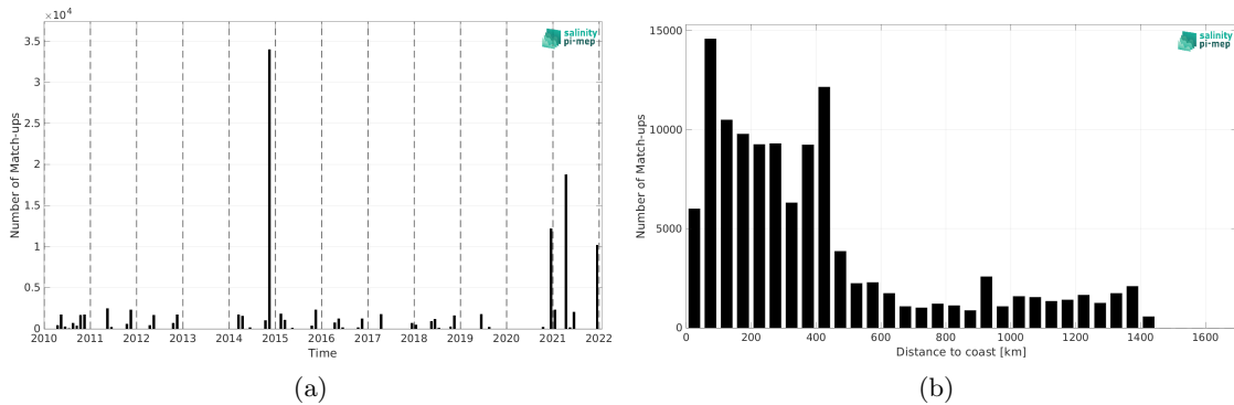
Figure 1: Number of match-ups between TSG (Polarstern) and SMOS SSS L3 v9 - 9 Days (CATDS-CEC-LOCEAN) SSS as a function of time (a) and as function of the distance to coast (b) over the North Atlantic Ocean Pi-MEP region and for the full satellite product period.
