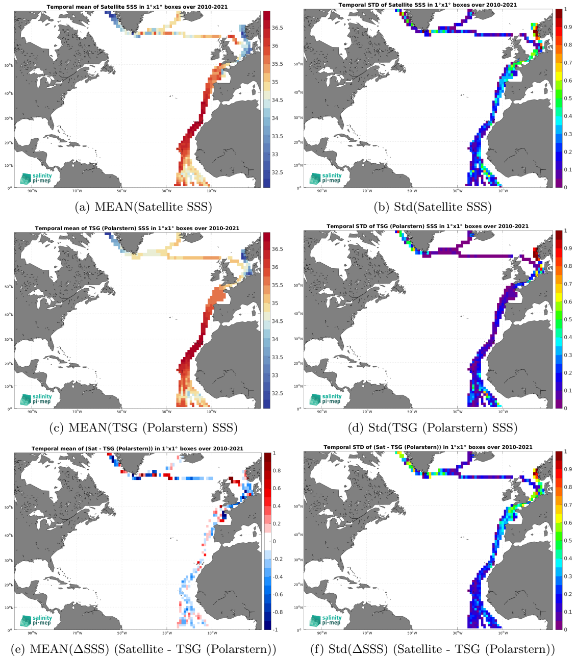
Figure 6: Temporal mean (left) and Std (right) of SSS from SMOS SSS L3 v9 - 9 Days (CATDS-CEC-LOCEAN) (top), TSG (Polarstern) (middle), and of \Delta SSS (Satellite - TSG (Polarstern)). Only match-up pairs are used to generate these maps.
