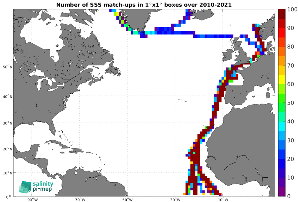
Figure 4: Number of SSS match-ups between TSG (Polarstern) SSS and the SMOS SSS L3 v9 - 9 Days (CATDS-CEC-LOCEAN) SSS product for the North Atlantic Ocean Pi-MEP region over 1^\circ \times 1^\circ boxes and for the full satellite product period.
