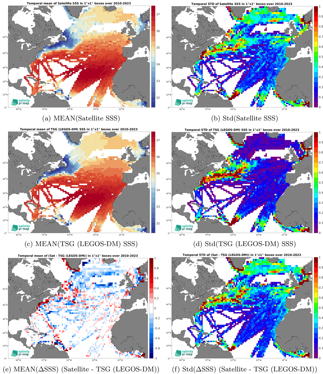
Figure 7: Temporal mean (left) and Std (right) of SSS from SMOS SSS L3 v9 - 9 Days (CATDS-CEC-LOCEAN) (top), TSG (LEGOS-DM) (middle), and of \Delta SSS (Satellite - TSG (LEGOS-DM)). Only match-up pairs are used to generate these maps.
