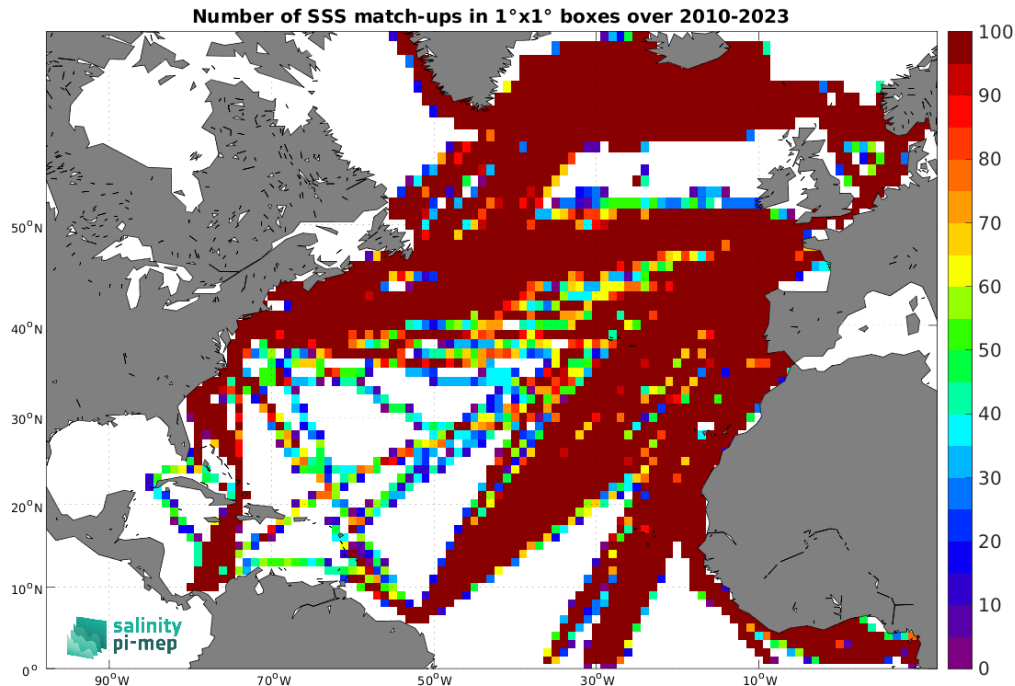
Figure 5: Number of SSS match-ups between TSG (LEGOS-DM) SSS and the SMOS SSS L3 v9 - 9 Days (CATDS-CEC-LOCEAN) SSS product for the North Atlantic Ocean Pi-MEP region over 1^\circ \times 1^\circ boxes and for the full satellite product period.
