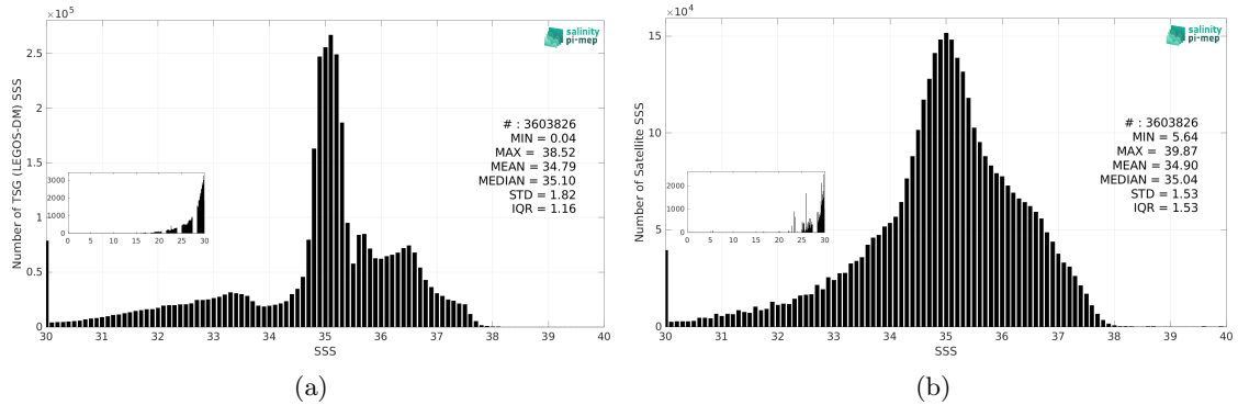
Figure 3: Histograms of SSS from TSG (LEGOS-DM) (a) and SMOS SSS L3 v9 - 9 Days (CATDS-CEC-LOCEAN) (b) considering all match-up pairs per bins of 0.1 over the North Atlantic Ocean Pi-MEP region and for the full satellite product period.
