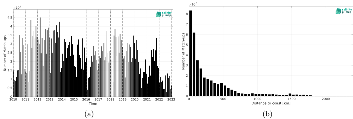
Figure 2: Number of match-ups between TSG (LEGOS-DM) and SMOS SSS L3 v9 - 9 Days (CATDS-CEC-LOCEAN) SSS as a function of time (a) and as function of the distance to coast (b) over the North Atlantic Ocean Pi-MEP region and for the full satellite product period.
