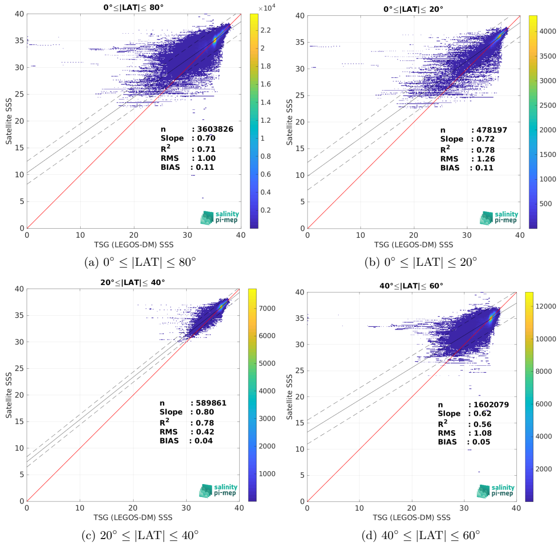
Figure 10: Contour maps of the concentration of SMOS SSS L3 v9 - 9 Days (CATDS-CEC-LOCEAN) SSS (y-axis) versus TSG (LEGOS-DM) SSS (x-axis) at match-up pairs for different latitude bands. For each plot, the red line shows x=y . The black thin and dashed lines indicate a linear fit through the data cloud and the \pm 95\% confidence levels, respectively. The number of match-up pairs n , the slope and R^2 coefficient of the linear fit, the root mean square (RMS) and the mean bias between satellite and in situ data are indicated for each latitude band in each plot.
