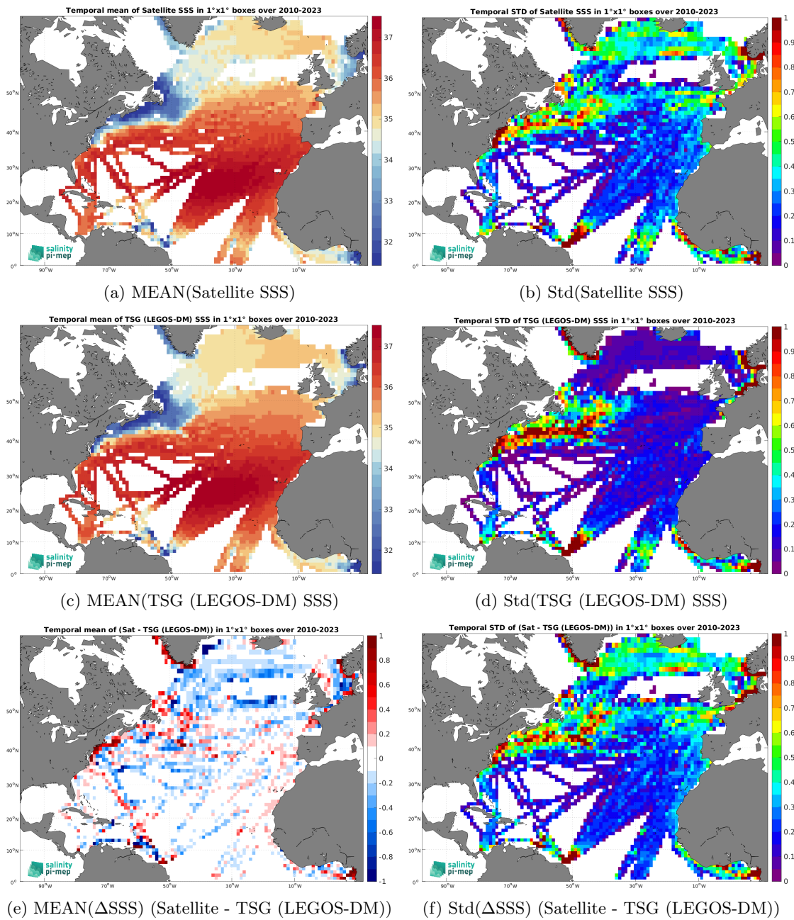
Figure 6: Temporal mean (left) and Std (right) of SSS from SMOS SSS L3 v9 - 9 Days (CATDS-CEC-LOCEAN) (top), TSG (LEGOS-DM) (middle), and of \Delta SSS (Satellite - TSG (LEGOS-DM)). Only match-up pairs are used to generate these maps.
