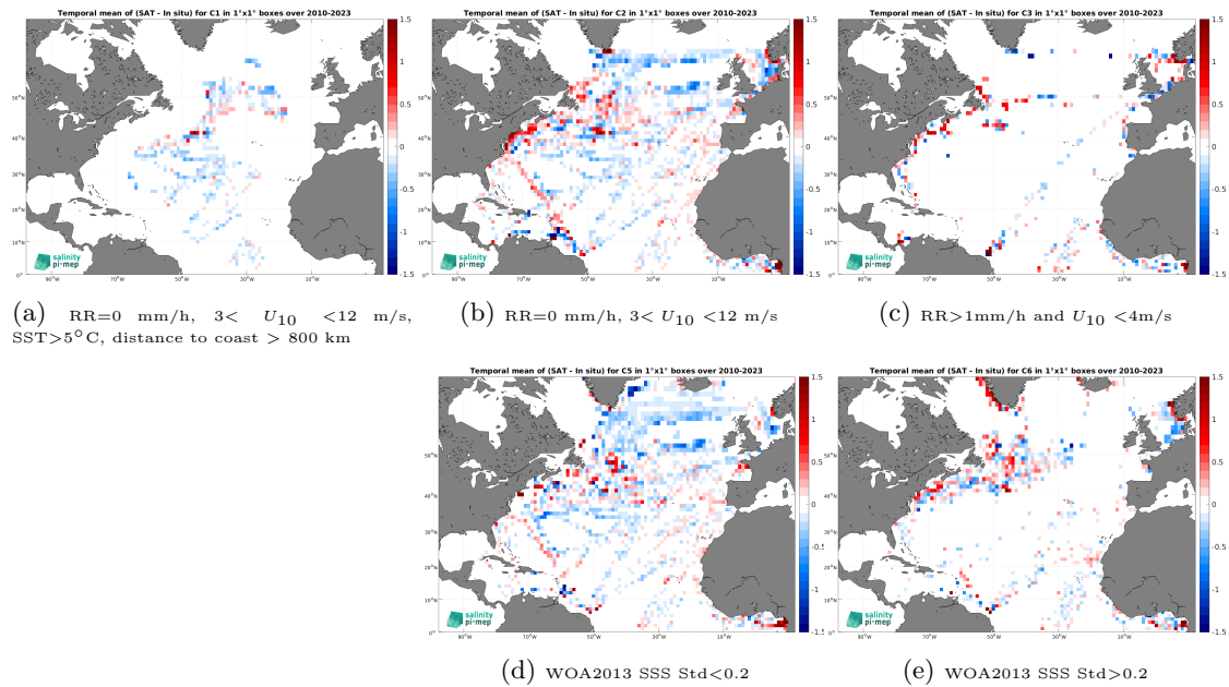
Figure 12: Temporal mean gridded over spatial boxes of size 1^\circ \times 1^\circ of \Delta\text{SSS} (SMOS SSS L3 v9 - 9 Days (CATDS-CEC-LOCEAN) - TSG (LEGOS-DM)) for 5 different subdatasets corresponding to:RR=0 mm/h, 3 < U_{10} < 12 m/s, SST >5^\circ\text{C} , distance to coast > 800 km (a), RR=0 mm/h, 3 < U_{10} < 12 m/s (b), RR >1 mm/h and U_{10} < 4 m/s (c), WOA2013 SSS Std <0.2 (d), WOA2013 SSS Std >0.2 (e).
