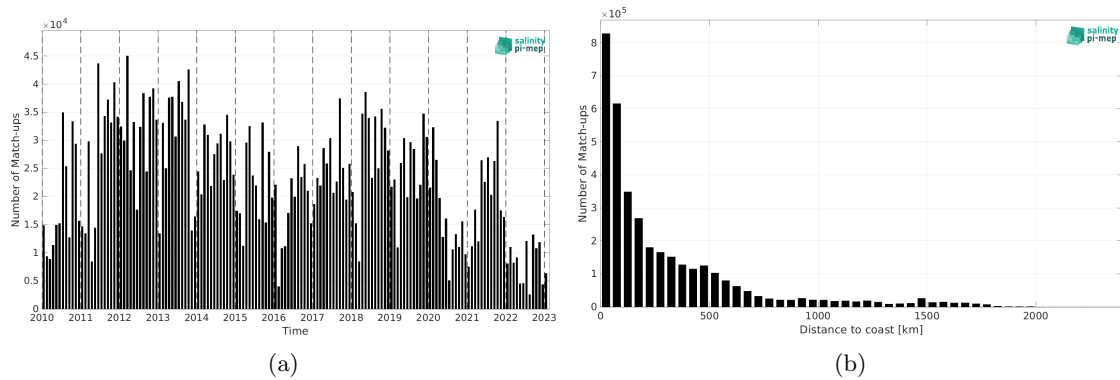
Figure 1: Number of match-ups between TSG (LEGOS-DM) and SMOS SSS L3 v9 - 9 Days (CATDS-CEC-LOCEAN) SSS as a function of time (a) and as function of the distance to coast (b) over the North Atlantic Ocean Pi-MEP region and for the full satellite product period.
