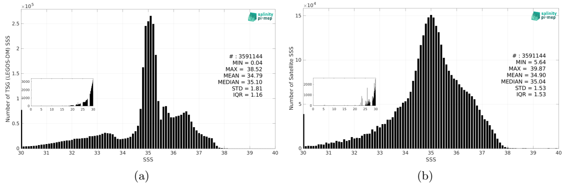
Figure 2: Histograms of SSS from TSG (LEGOS-DM) (a) and SMOS SSS L3 v9 - 9 Days (CATDS-CEC-LOCEAN) (b) considering all match-up pairs per bins of 0.1 over the North Atlantic Ocean Pi-MEP region and for the full satellite product period.
