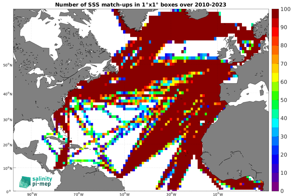
Figure 4: Number of SSS match-ups between TSG (LEGOS-DM) SSS and the SMOS SSS L3 v9 - 9 Days (CATDS-CEC-LOCEAN) SSS product for the North Atlantic Ocean Pi-MEP region over 1^\circ \times 1^\circ boxes and for the full satellite product period.
