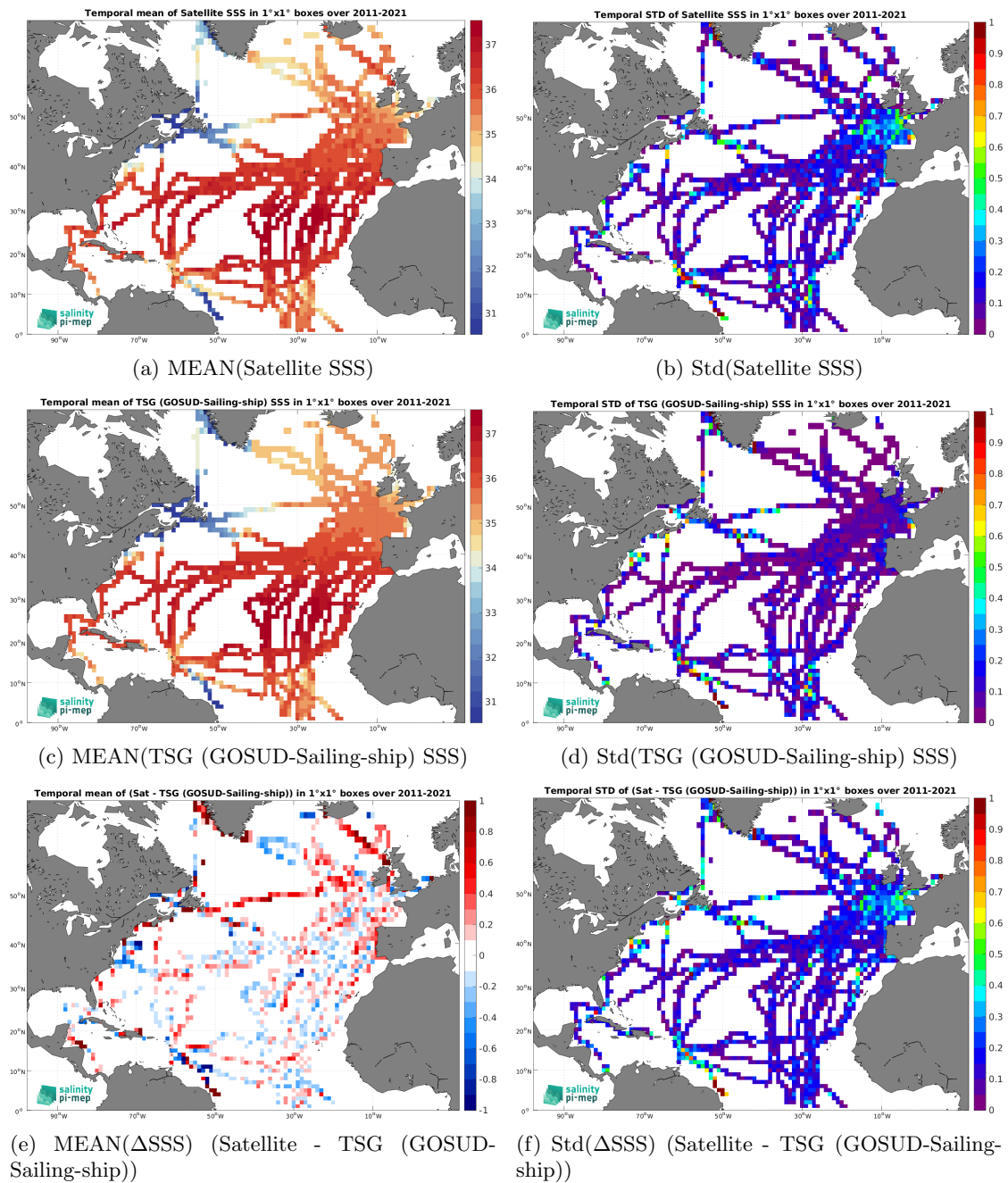
Figure 7: Temporal mean (left) and Std (right) of SSS from SMOS SSS L3 v9 - 9 Days (CATDS-CEC-LOCEAN) (top), TSG (GOSUD-Sailing-ship) (middle), and of \Delta SSS (Satellite - TSG (GOSUD-Sailing-ship)). Only match-up pairs are used to generate these maps.
