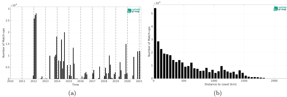
Figure 2: Number of match-ups between TSG (GOSUD-Sailing-ship) and SMOS SSS L3 v9 - 9 Days (CATDS-CEC-LOCEAN) SSS as a function of time (a) and as function of the distance to coast (b) over the North Atlantic Ocean Pi-MEP region and for the full satellite product period.
