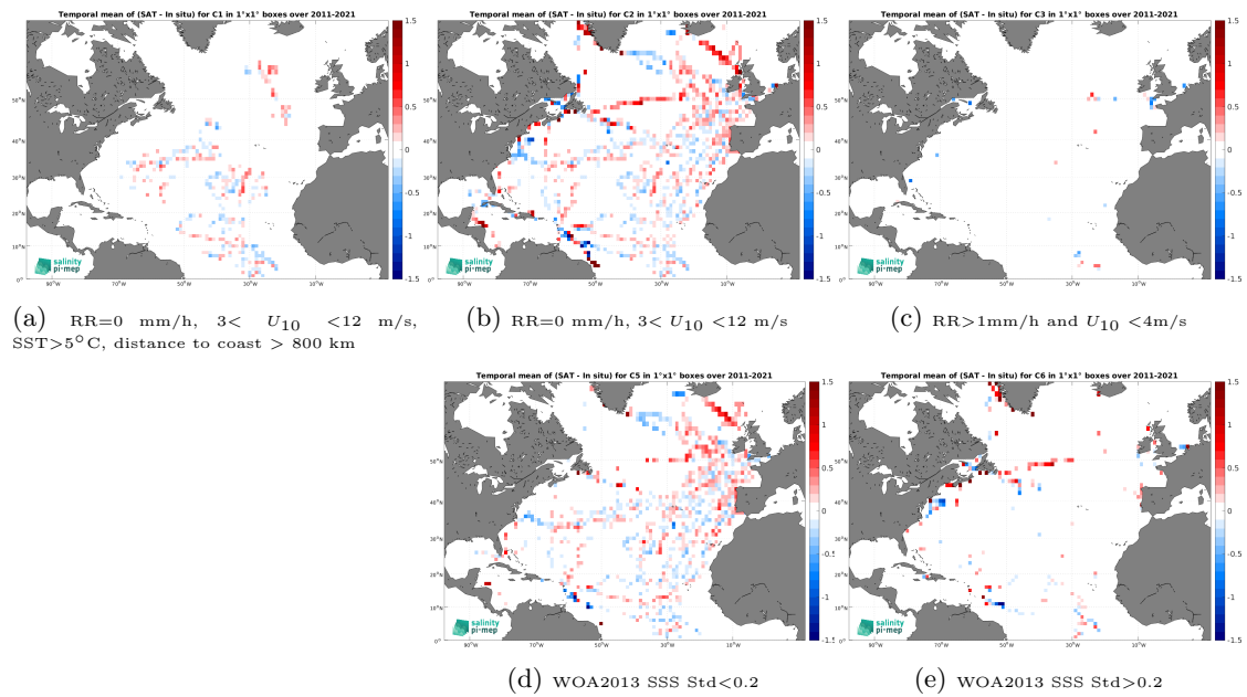
Figure 14: Temporal mean gridded over spatial boxes of size 1^\circ \times 1^\circ of \Delta\text{SSS} (SMOS SSS L3 v9 - 9 Days (CATDS-CEC-LOCEAN) - TSG (GOSUD-Sailing-ship)) for 5 different subdatasets corresponding to:RR=0 mm/h, 3 < U_{10} < 12 m/s, SST >5^\circ\text{C} , distance to coast > 800 km (a), RR=0 mm/h, 3 < U_{10} < 12 m/s (b), RR >1 mm/h and U_{10} < 4 m/s (c), WOA2013 SSS Std <0.2 (d), WOA2013 SSS Std >0.2 (e).
