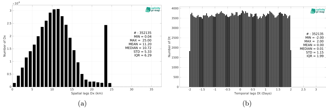
Figure 6: Histograms of the spatial (a) and temporal (b) lags between the location/time of the TSG (GOSUD-Sailing-ship) measurement and the date of the corresponding SMOS SSS L3 v9 - 9 Days (CATDS-CEC-LOCEAN) SSS pixel.
