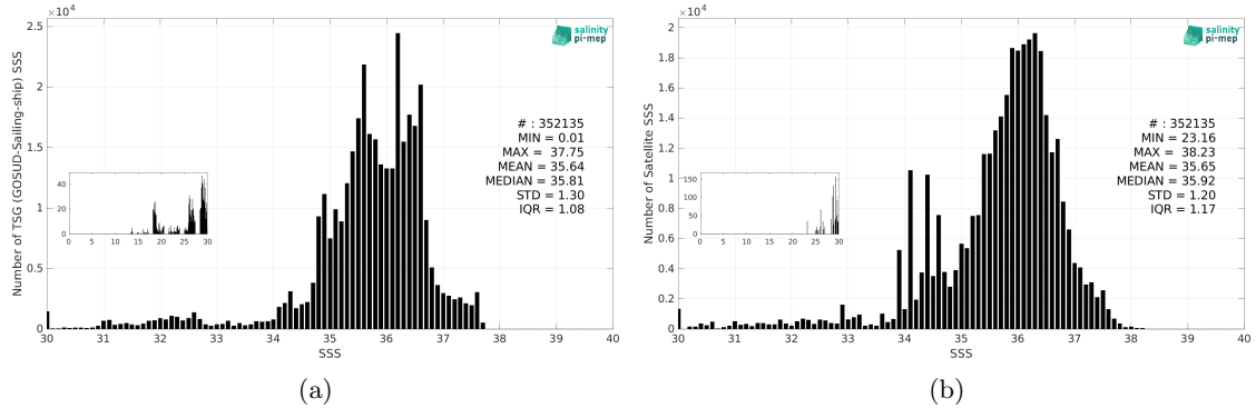
Figure 2: Histograms of SSS from TSG (GOSUD-Sailing-ship) (a) and SMOS SSS L3 v9 - 9 Days (CATDS-CEC-LOCEAN) (b) considering all match-up pairs per bins of 0.1 over the North Atlantic Ocean Pi-MEP region and for the full satellite product period.
