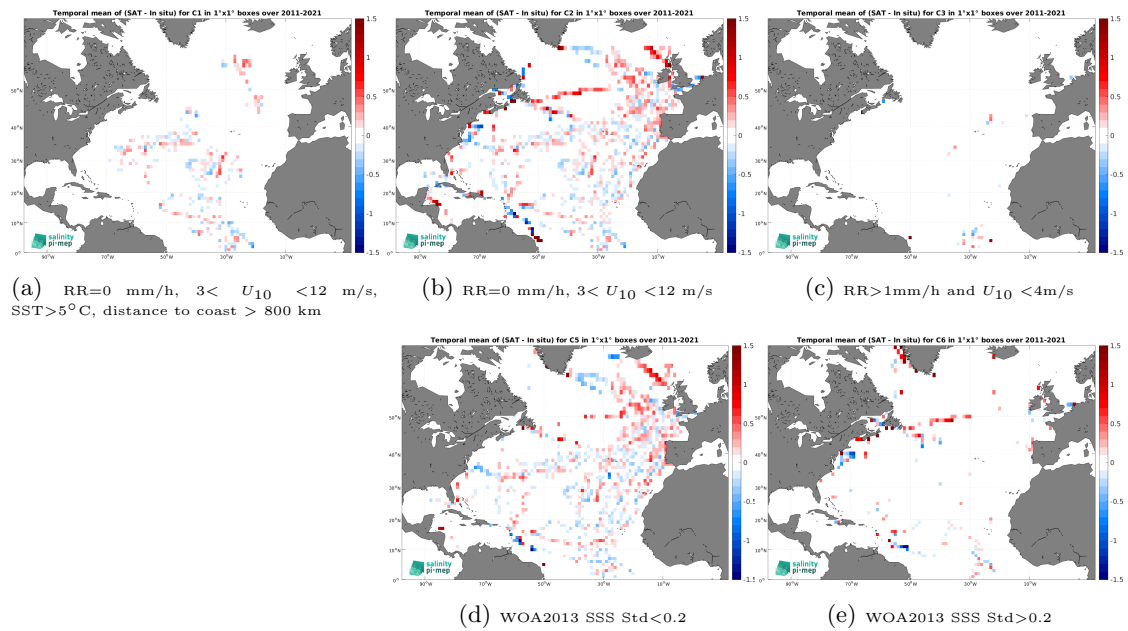
Figure 12: Temporal mean gridded over spatial boxes of size 1^\circ \times 1^\circ of \Delta\text{SSS} (SMOS SSS L3 v9 - 9 Days (CATDS-CEC-LOCEAN) - TSG (GOSUD-Sailing-ship)) for 5 different subdatasets corresponding to:RR=0 mm/h, 3 < U_{10} < 12 m/s, SST>5°C, distance to coast > 800 km (a), RR=0 mm/h, 3 < U_{10} < 12 m/s (b), RR>1mm/h and U_{10} < 4 m/s (c), WOA2013 SSS Std<0.2 (d), WOA2013 SSS Std>0.2 (e).
