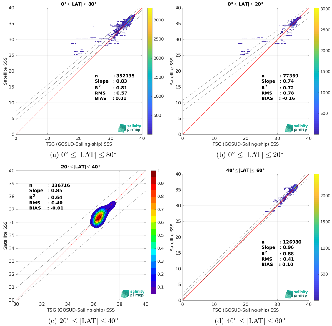
Figure 9: Contour maps of the concentration of SMOS SSS L3 v9 - 9 Days (CATDS-CEC-LOCEAN) SSS (y-axis) versus TSG (GOSUD-Sailing-ship) SSS (x-axis) at match-up pairs for different latitude bands. For each plot, the red line shows x=y . The black thin and dashed lines indicate a linear fit through the data cloud and the \pm 95\% confidence levels, respectively. The number match-up pairs n , the slope and R^2 coefficient of the linear fit, the root mean square (RMS) and the mean bias between satellite and in situ data are indicated for each latitude band in each plots.
