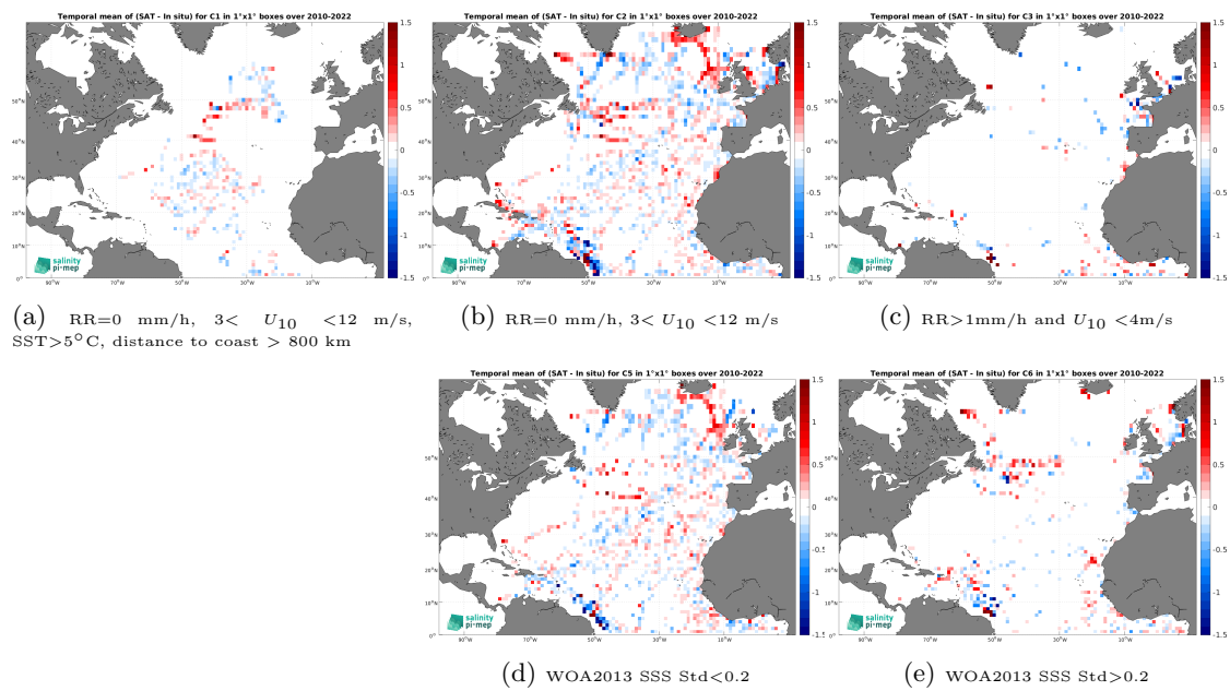
Figure 14: Temporal mean gridded over spatial boxes of size 1^\circ \times 1^\circ of \Delta\text{SSS} (SMOS SSS L3 v9 - 9 Days (CATDS-CEC-LOCEAN) - TSG (GOSUD-Research-vessel)) for 5 different subdatasets corresponding to:RR=0 mm/h, 3 < U_{10} < 12 m/s, SST >5^\circ\text{C} , distance to coast > 800 km (a), RR=0 mm/h, 3 < U_{10} < 12 m/s (b), RR >1 mm/h and U_{10} < 4 m/s (c), WOA2013 SSS Std <0.2 (d), WOA2013 SSS Std >0.2 (e).
