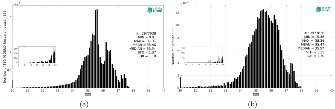
Figure 2: Histograms of SSS from TSG (GOSUD-Research-vessel) (a) and SMOS SSS L3 v9 - 9 Days (CATDS-CEC-LOCEAN) (b) considering all match-up pairs per bins of 0.1 over the North Atlantic Ocean Pi-MEP region and for the full satellite product period.
