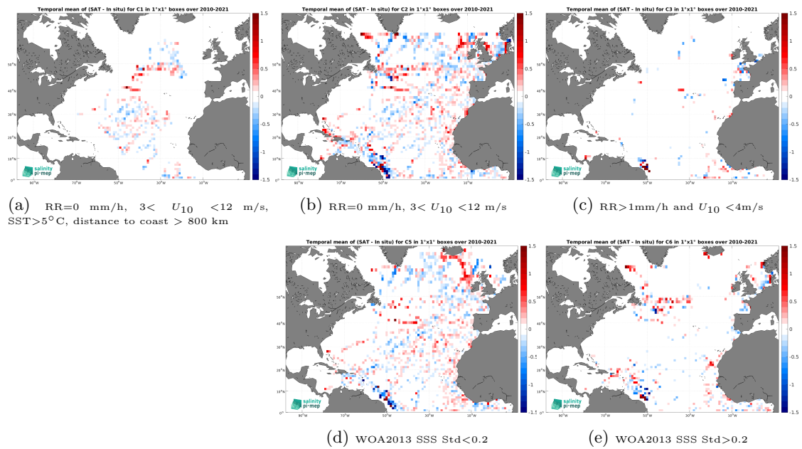
Figure 12: Temporal mean gridded over spatial boxes of size 1^\circ \times 1^\circ of \Delta\text{SSS} (SMOS SSS L3 v9 - 9 Days (CATDS-CEC-LOCEAN) - TSG (GOSUD-Research-vessel)) for 5 different subdatasets corresponding to:RR=0 mm/h, 3 < U_{10} < 12 m/s, SST>5°C, distance to coast > 800 km (a), RR=0 mm/h, 3 < U_{10} < 12 m/s (b), RR>1mm/h and U_{10} < 4 m/s (c), WOA2013 SSS Std<0.2 (d), WOA2013 SSS Std>0.2 (e).
