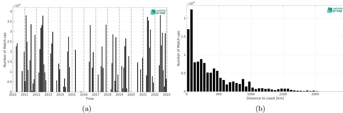
Figure 2: Number of match-ups between TSG (CSIC-UTM) and SMOS SSS L3 v9 - 9 Days (CATDS-CEC-LOCEAN) SSS as a function of time (a) and as function of the distance to coast (b) over the North Atlantic Ocean Pi-MEP region and for the full satellite product period.
