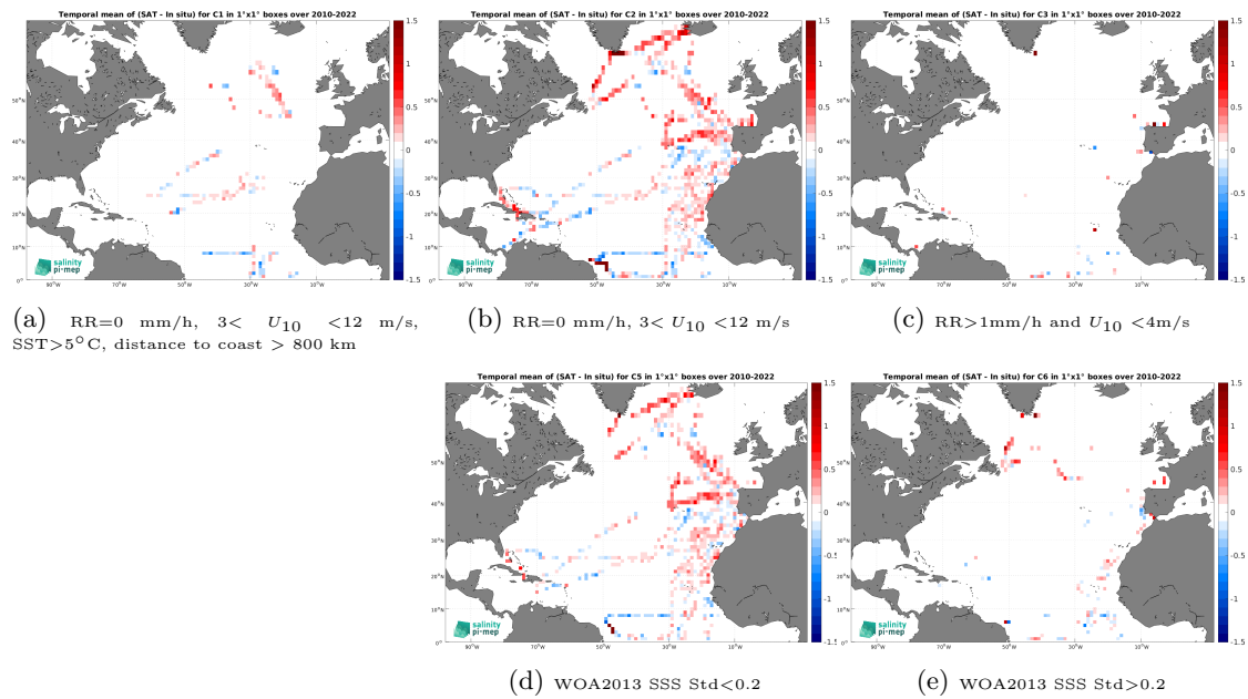
Figure 14: Temporal mean gridded over spatial boxes of size 1^\circ \times 1^\circ of \Delta\text{SSS} (SMOS SSS L3 v9 - 9 Days (CATDS-CEC-LOCEAN) - TSG (CSIC-UTM)) for 5 different subdatasets corresponding to:RR=0 mm/h, 3 < U_{10} < 12 m/s, SST >5^\circ\text{C} , distance to coast > 800 km (a), RR=0 mm/h, 3 < U_{10} < 12 m/s (b), RR >1 mm/h and U_{10} < 4 m/s (c), WOA2013 SSS Std <0.2 (d), WOA2013 SSS Std >0.2 (e).
