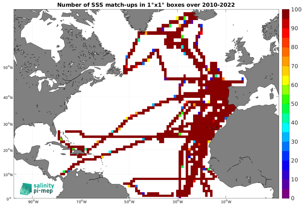
Figure 5: Number of SSS match-ups between TSG (CSIC-UTM) SSS and the SMOS SSS L3 v9 - 9 Days (CATDS-CEC-LOCEAN) SSS product for the North Atlantic Ocean Pi-MEP region over 1^\circ \times 1^\circ boxes and for the full satellite product period.
