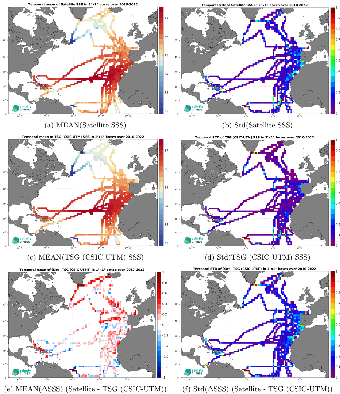
Figure 7: Temporal mean (left) and Std (right) of SSS from SMOS SSS L3 v9 - 9 Days (CATDS-CEC-LOCEAN) (top), TSG (CSIC-UTM) (middle), and of \Delta SSS (Satellite - TSG (CSIC-UTM)). Only match-up pairs are used to generate these maps.
