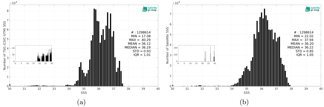
Figure 3: Histograms of SSS from TSG (CSIC-UTM) (a) and SMOS SSS L3 v9 - 9 Days (CATDS-CEC-LOCEAN) (b) considering all match-up pairs per bins of 0.1 over the North Atlantic Ocean Pi-MEP region and for the full satellite product period.
