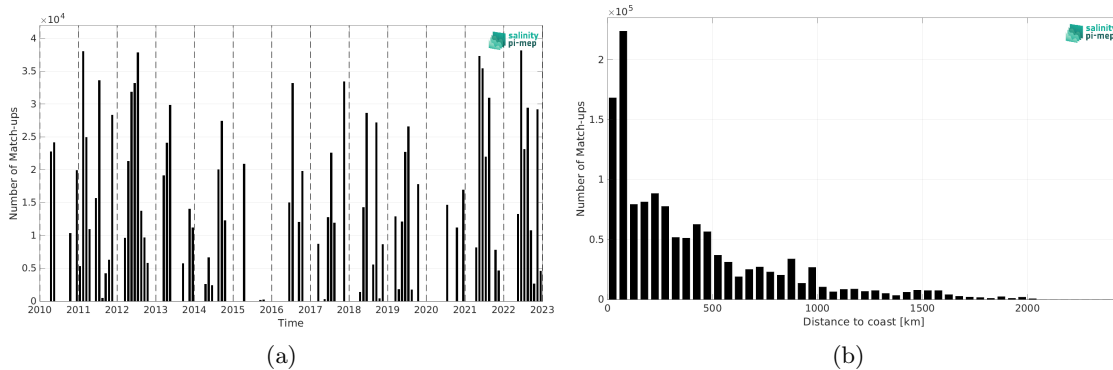
Figure 1: Number of match-ups between TSG (CSIC-UTM) and SMOS SSS L3 v9 - 9 Days (CATDS-CEC-LOCEAN) SSS as a function of time (a) and as function of the distance to coast (b) over the North Atlantic Ocean Pi-MEP region and for the full satellite product period.
