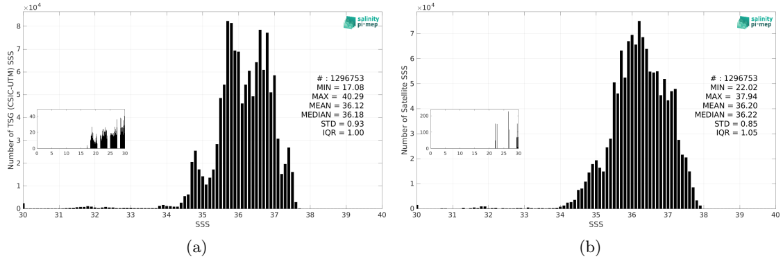
Figure 2: Histograms of SSS from TSG (CSIC-UTM) (a) and SMOS SSS L3 v9 - 9 Days (CATDS-CEC-LOCEAN) (b) considering all match-up pairs per bins of 0.1 over the North Atlantic Ocean Pi-MEP region and for the full satellite product period.
