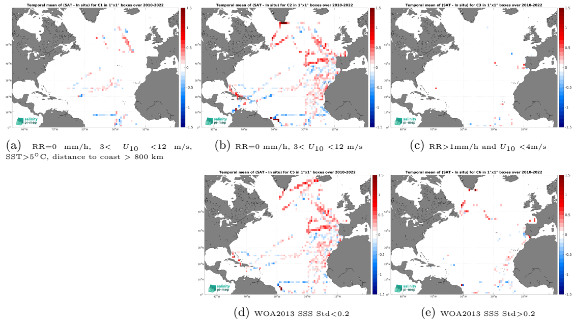
Figure 12: Temporal mean gridded over spatial boxes of size 1^\circ \times 1^\circ of \Delta\text{SSS} (SMOS SSS L3 v9 - 9 Days (CATDS-CEC-LOCEAN) - TSG (CSIC-UTM)) for 5 different subdatasets corresponding to:RR=0 mm/h, 3 < U_{10} < 12 m/s, SST >5^\circ\text{C} , distance to coast > 800 km (a), RR=0 mm/h, 3 < U_{10} < 12 m/s (b), RR >1 mm/h and U_{10} < 4 m/s (c), WOA2013 SSS Std <0.2 (d), WOA2013 SSS Std >0.2 (e).
