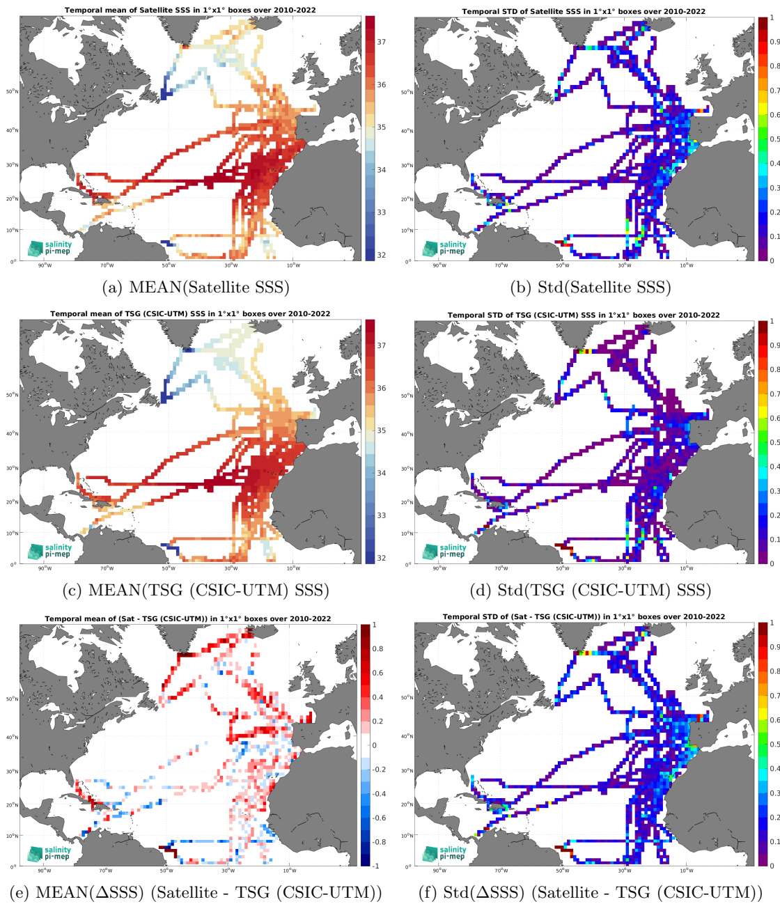
Figure 6: Temporal mean (left) and Std (right) of SSS from SMOS SSS L3 v9 - 9 Days (CATDS-CEC-LOCEAN) (top), TSG (CSIC-UTM) (middle), and of \Delta SSS (Satellite - TSG (CSIC-UTM)). Only match-up pairs are used to generate these maps.
