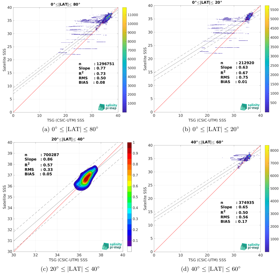
Figure 9: Contour maps of the concentration of SMOS SSS L3 v9 - 9 Days (CATDS-CEC-LOCEAN) SSS (y-axis) versus TSG (CSIC-UTM) SSS (x-axis) at match-up pairs for different latitude bands. For each plot, the red line shows x=y . The black thin and dashed lines indicate a linear fit through the data cloud and the \pm 95\% confidence levels, respectively. The number match-up pairs n , the slope and R^2 coefficient of the linear fit, the root mean square (RMS) and the mean bias between satellite and in situ data are indicated for each latitude band in each plots.
