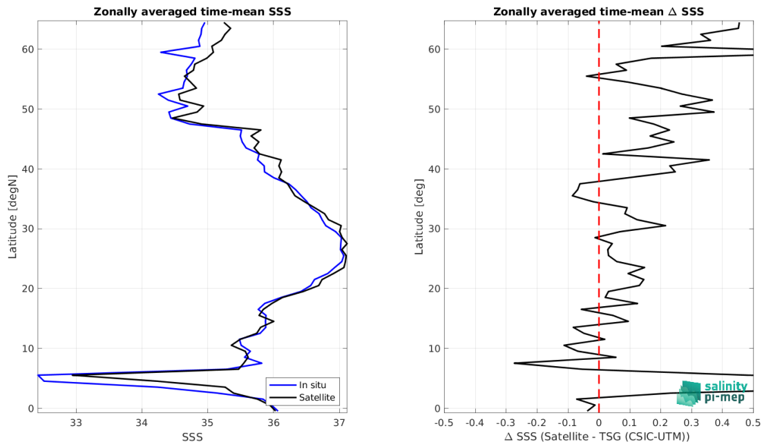
Figure 8: Left panel: Zonal mean SSS from SMOS SSS L3 v9 - 9 Days (CATDS-CEC-LOCEAN) satellite product (black) and from TSG (CSIC-UTM) (blue). Right panel: Zonal mean of \Delta SSS (Satellite - TSG (CSIC-UTM)) for all the collected Pi-MEP match-up pairs estimated over the full satellite product period.
