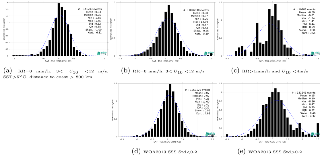
Figure 13: Normalized histogram of \Delta SSS (SMOS SSS L3 v9 - 9 Days (CATDS-CEC-LOCEAN) - TSG (CSIC-UTM)) for 5 different subdatasets corresponding to: RR=0 mm/h, 3 < U_{10} < 12 m/s, SST>5°C, distance to coast > 800 km (a), RR=0 mm/h, 3 < U_{10} < 12 m/s (b), RR>1mm/h and U_{10} < 4 m/s (c), WOA2013 SSS Std<0.2 (d), WOA2013 SSS Std>0.2 (e).
