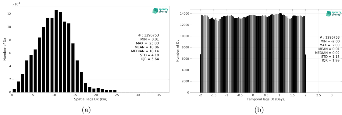
Figure 5: Histograms of the spatial (a) and temporal (b) lags between the location/time of the TSG (CSIC-UTM) measurement and the date of the corresponding SMOS SSS L3 v9 - 9 Days (CATDS-CEC-LOCEAN) SSS pixel.
