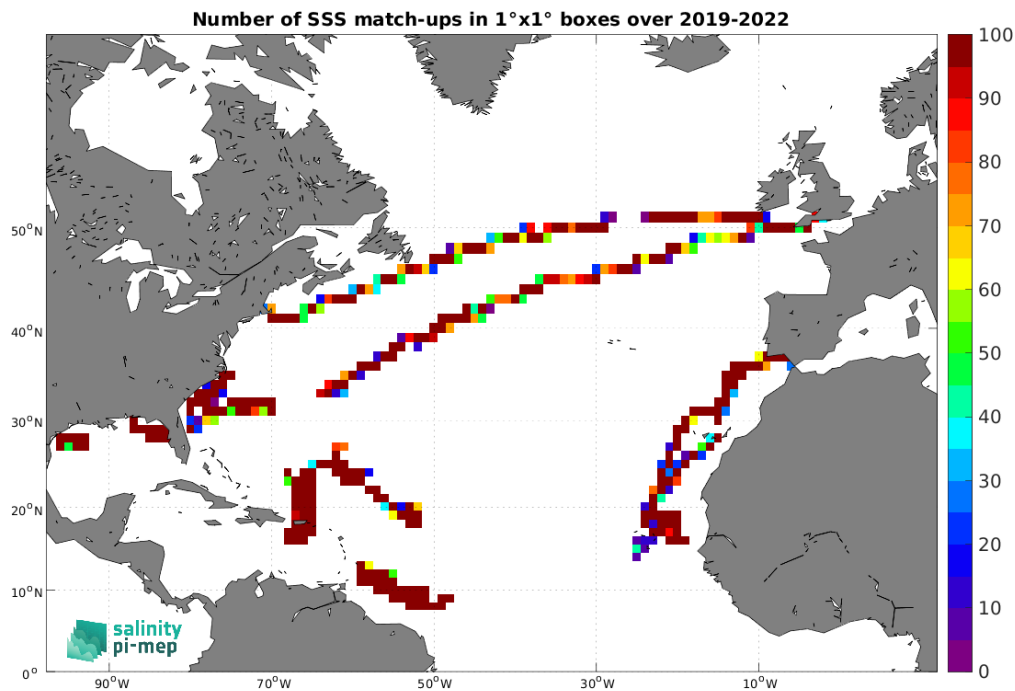
Figure 5: Number of SSS match-ups between Saildrone SSS and the SMOS SSS L3 v9 - 9 Days (CATDS-CEC-LOCEAN) SSS product for the North Atlantic Ocean Pi-MEP region over 1^\circ \times 1^\circ boxes and for the full satellite product period.
