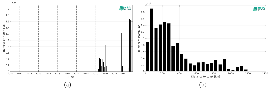
Figure 2: Number of match-ups between Saildrone and SMOS SSS L3 v9 - 9 Days (CATDS-CEC-LOCEAN) SSS as a function of time (a) and as function of the distance to coast (b) over the North Atlantic Ocean Pi-MEP region and for the full satellite product period.
