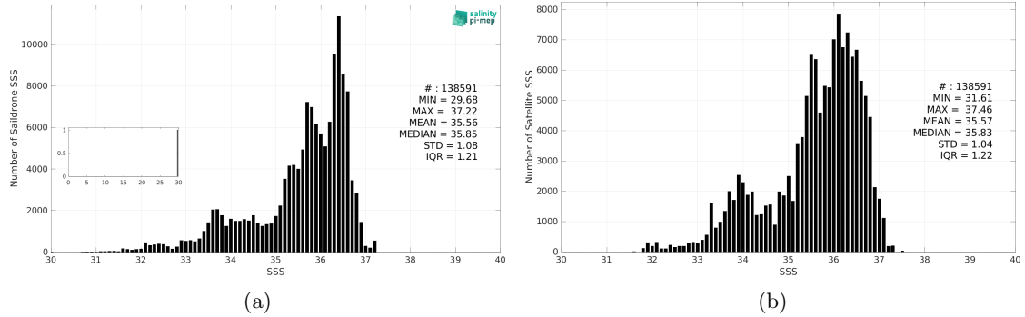
Figure 3: Histograms of SSS from Saildrone (a) and SMOS SSS L3 v9 - 9 Days (CATDS-CEC-LOCEAN) (b) considering all match-up pairs per bins of 0.1 over the North Atlantic Ocean Pi-MEP region and for the full satellite product period.
