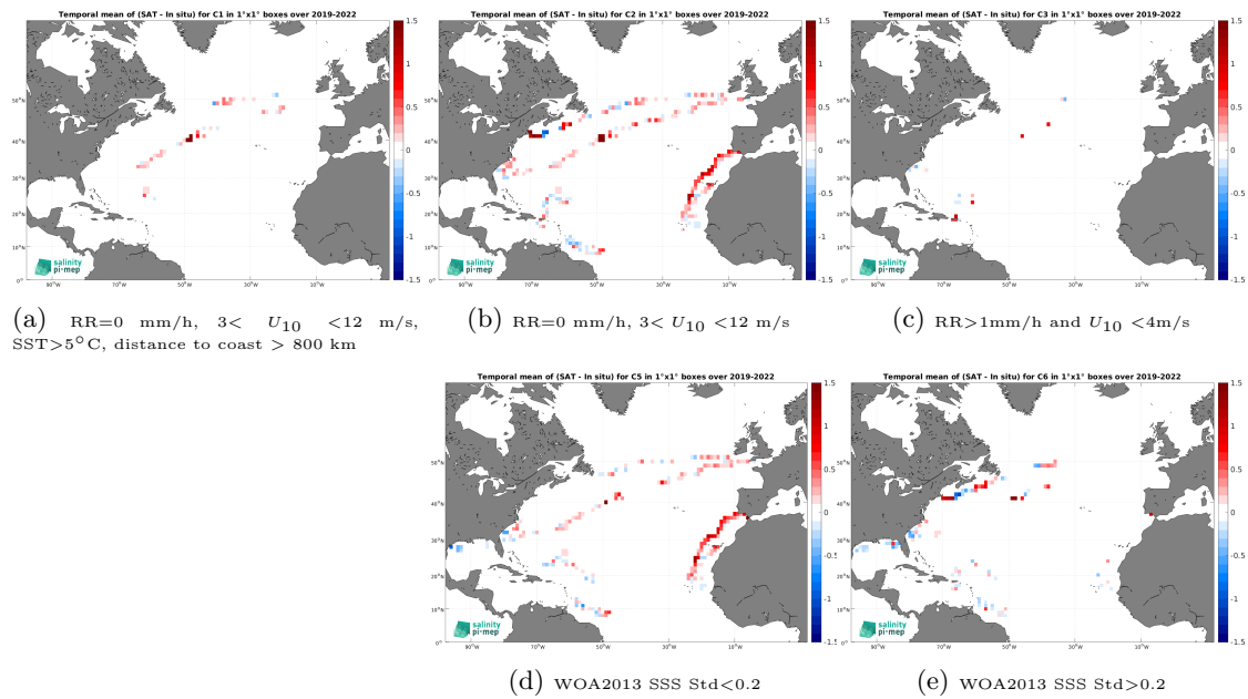
Figure 14: Temporal mean gridded over spatial boxes of size 1^\circ \times 1^\circ of \Delta\text{SSS} (SMOS SSS L3 v9 - 9 Days (CATDS-CEC-LOCEAN) - Saildrone) for 5 different subdatasets corresponding to:RR=0 mm/h, 3 < U_{10} < 12 m/s, SST >5^\circ\text{C} , distance to coast > 800 km (a), RR=0 mm/h, 3 < U_{10} < 12 m/s (b), RR >1 mm/h and U_{10} < 4 m/s (c), WOA2013 SSS Std <0.2 (d), WOA2013 SSS Std >0.2 (e).
