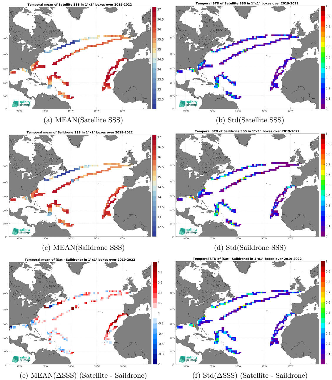
Figure 7: Temporal mean (left) and Std (right) of SSS from SMOS SSS L3 v9 - 9 Days (CATDS-CEC-LOCEAN) (top), Saildrone (middle), and of \Delta SSS (Satellite - Saildrone). Only match-up pairs are used to generate these maps.
