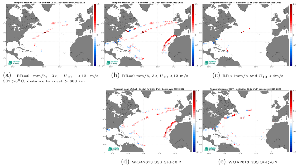
Figure 12: Temporal mean gridded over spatial boxes of size 1^\circ \times 1^\circ of \Delta\text{SSS} (SMOS SSS L3 v9 - 9 Days (CATDS-CEC-LOCEAN) - Saildrone) for 5 different subdatasets corresponding to:RR=0 mm/h, 3 < U_{10} < 12 m/s, SST > 5^\circ\text{C} , distance to coast > 800 km (a), RR=0 mm/h, 3 < U_{10} < 12 m/s (b), RR > 1 mm/h and U_{10} < 4 m/s (c), WOA2013 SSS Std < 0.2 (d), WOA2013 SSS Std > 0.2 (e).
