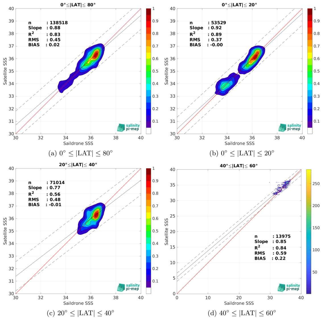
Figure 9: Contour maps of the concentration of SMOS SSS L3 v9 - 9 Days (CATDS-CEC-LOCEAN) SSS (y-axis) versus Sailability SSS (x-axis) at match-up pairs for different latitude bands. For each plot, the red line shows x=y . The black thin and dashed lines indicate a linear fit through the data cloud and the \pm 95\% confidence levels, respectively. The number match-up pairs n , the slope and R^2 coefficient of the linear fit, the root mean square (RMS) and the mean bias between satellite and in situ data are indicated for each latitude band in each plots.
