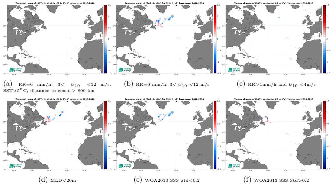
Figure 14: Temporal mean gridded over spatial boxes of size 1^\circ \times 1^\circ of \Delta\text{SSS} (SMOS SSS L3 v9 - 9 Days (CATDS-CEC-LOCEAN) - Marine mammals) for 6 different subdatasets corresponding to:RR=0 mm/h, 3 < U_{10} < 12 m/s, SST>5°C, distance to coast > 800 km (a), RR=0 mm/h, 3 < U_{10} < 12 m/s (b), RR>1mm/h and U_{10} < 4 m/s (c),MLD<20m (d),WOA2013 SSS Std<0.2 (e),WOA2013 SSS Std>0.2 (f).
