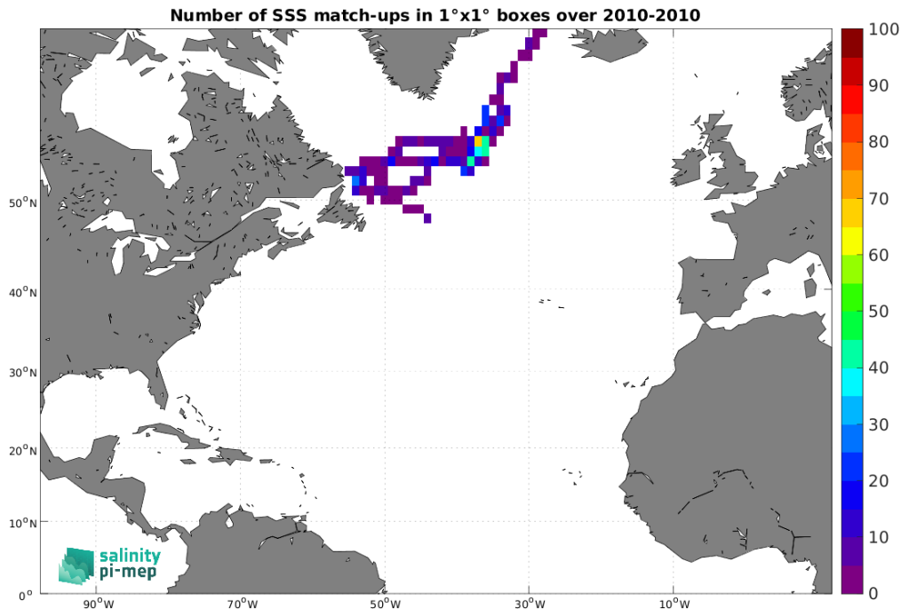
Figure 4: Number of SSS match-ups between Marine mammals SSS and the SMOS SSS L3 v9 - 9 Days (CATDS-CEC-LOCEAN) SSS product for the North Atlantic Ocean Pi-MEP region over 1^\circ \times 1^\circ boxes and for the full satellite product period.
