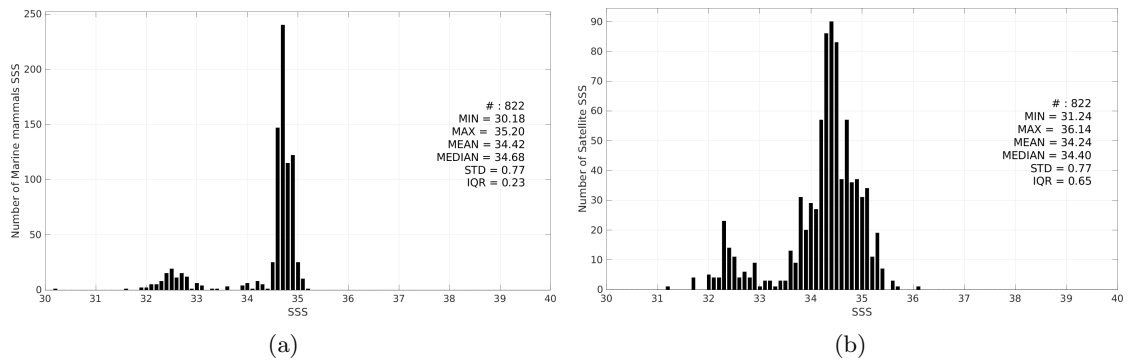
Figure 2: Histograms of SSS from Marine mammals (a) and SMOS SSS L3 v9 - 9 Days (CATDS-CEC-LOCEAN) (b) considering all match-up pairs per bins of 0.1 over the North Atlantic Ocean Pi-MEP region and for the full satellite product period.
