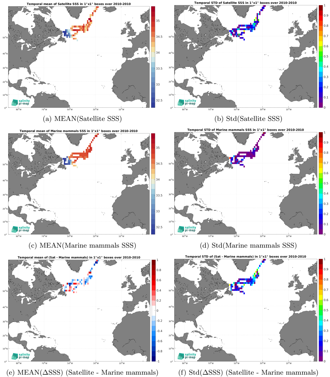
Figure 6: Temporal mean (left) and Std (right) of SSS from SMOS SSS L3 v9 - 9 Days (CATDS-CEC-LOCEAN) (top), Marine mammals (middle), and of \Delta SSS (Satellite - Marine mammals). Only match-up pairs are used to generate these maps.
