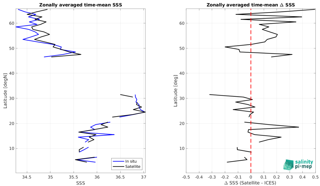
Figure 9: Left panel: Zonal mean SSS from SMOS SSS L3 v9 - 9 Days (CATDS-CEC-LOCEAN) satellite product (black) and from ICES (blue). Right panel: Zonal mean of \Delta SSS (Satellite - ICES) for all the collected Pi-MEP match-up pairs estimated over the full satellite product period.
