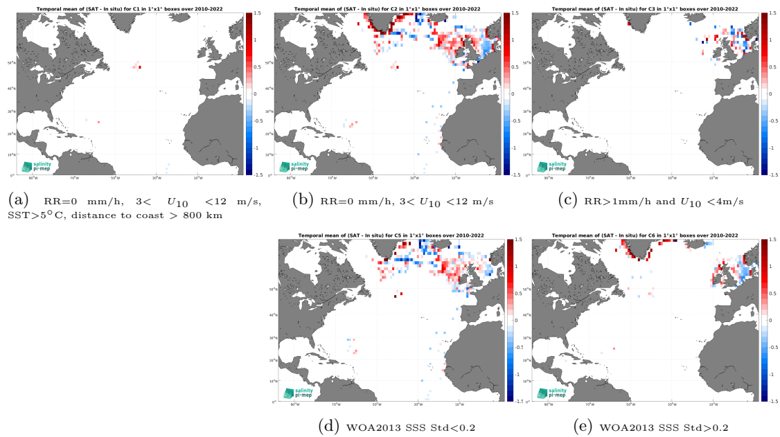
Figure 14: Temporal mean gridded over spatial boxes of size 1^\circ \times 1^\circ of \Delta\text{SSS} (SMOS SSS L3 v9 - 9 Days (CATDS-CEC-LOCEAN) - ICES) for 5 different subdatasets corresponding to:RR=0 mm/h, 3 < U_{10} < 12 m/s, SST >5^\circ\text{C} , distance to coast > 800 km (a), RR=0 mm/h, 3 < U_{10} < 12 m/s (b), RR >1 mm/h and U_{10} < 4 m/s (c), WOA2013 SSS Std <0.2 (d), WOA2013 SSS Std >0.2 (e).
