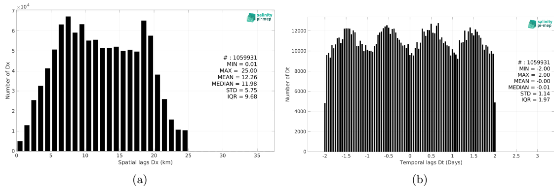
Figure 6: Histograms of the spatial (a) and temporal (b) lags between the location/time of the ICES measurement and the date of the corresponding SMOS SSS L3 v9 - 9 Days (CATDS-CEC-LOCEAN) SSS pixel.
