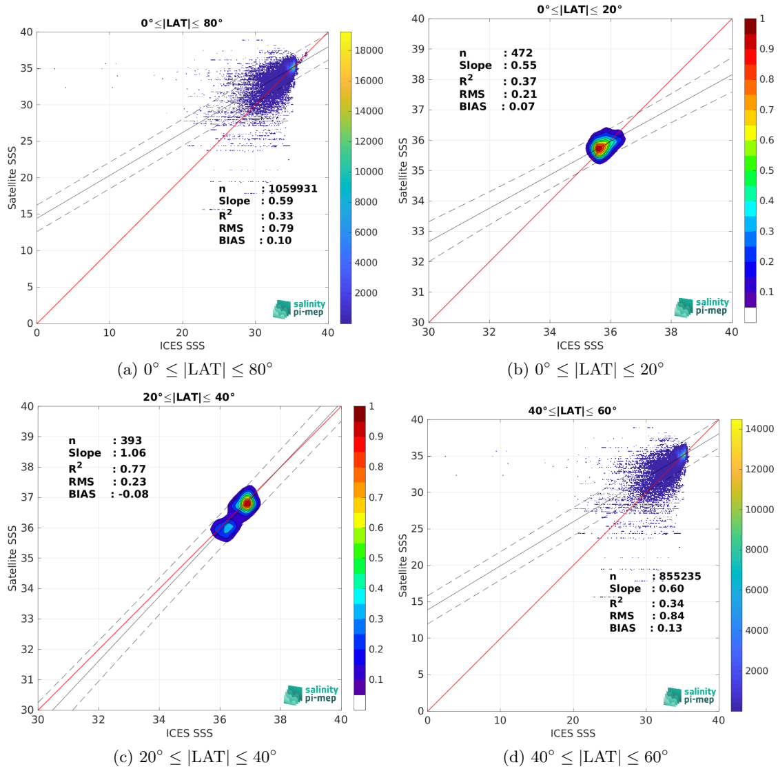
Figure 10: Contour maps of the concentration of SMOS SSS L3 v9 - 9 Days (CATDS-CEC-LOCEAN) SSS (y-axis) versus ICES SSS (x-axis) at match-up pairs for different latitude bands. For each plot, the red line shows x=y . The black thin and dashed lines indicate a linear fit through the data cloud and the \pm 95\% confidence levels, respectively. The number match-up pairs n , the slope and R^2 coefficient of the linear fit, the root mean square (RMS) and the mean bias between satellite and in situ data are indicated for each latitude band in each plots.
