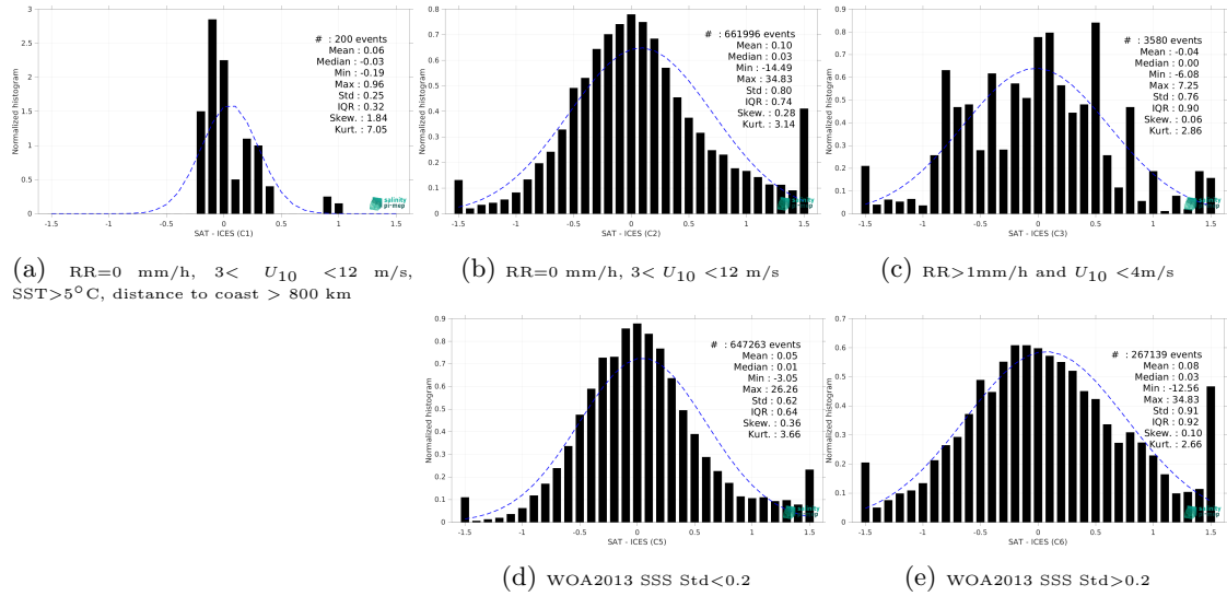
Figure 15: Normalized histogram of \Delta SSS (SMOS SSS L3 v9 - 9 Days (CATDS-CEC-LOCEAN) - ICES) for 5 different subdatasets corresponding to: RR=0 mm/h, 3 < U_{10} < 12 m/s, SST > 5°C, distance to coast > 800 km (a), RR=0 mm/h, 3 < U_{10} < 12 m/s (b), RR > 1mm/h and U_{10} < 4 m/s (c), WOA2013 SSS Std < 0.2 (d), WOA2013 SSS Std > 0.2 (e).
