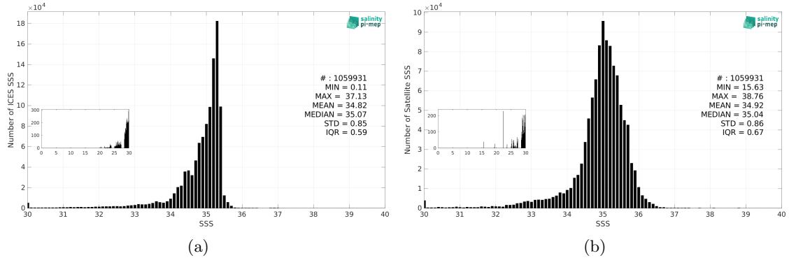
Figure 3: Histograms of SSS from ICES (a) and SMOS SSS L3 v9 - 9 Days (CATDS-CEC-LOCEAN) (b) considering all match-up pairs per bins of 0.1 over the North Atlantic Ocean Pi-MEP region and for the full satellite product period.
