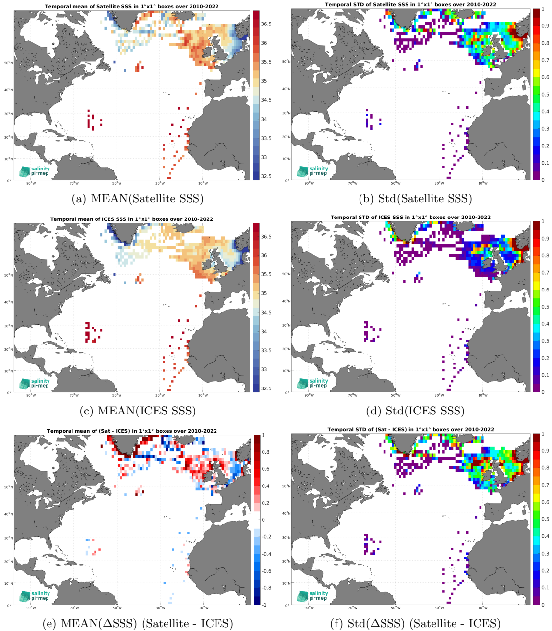
Figure 7: Temporal mean (left) and Std (right) of SSS from SMOS SSS L3 v9 - 9 Days (CATDS-CEC-LOCEAN) (top), ICES (middle), and of \Delta SSS (Satellite - ICES). Only match-up pairs are used to generate these maps.
