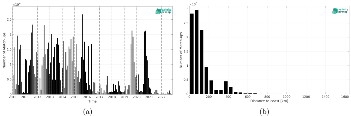
Figure 2: Number of match-ups between ICES and SMOS SSS L3 v9 - 9 Days (CATDS-CEC-LOCEAN) SSS as a function of time (a) and as function of the distance to coast (b) over the North Atlantic Ocean Pi-MEP region and for the full satellite product period.
