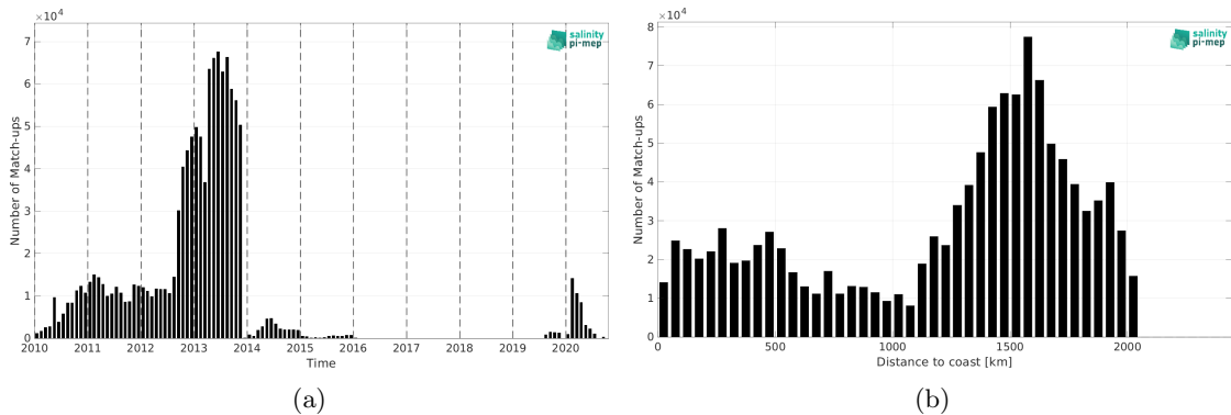
Figure 1: Number of match-ups between Surface drifters and SMOS SSS L3 v9 - 9 Days (CATDS-CEC-LOCEAN) SSS as a function of time (a) and as function of the distance to coast (b) over the North Atlantic Ocean Pi-MEP region and for the full satellite product period.
