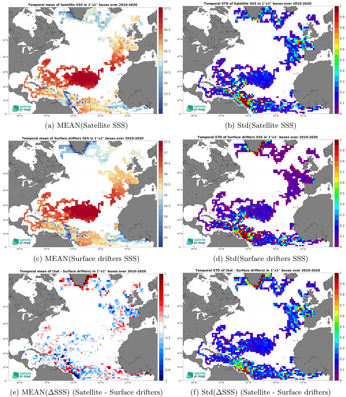
Figure 5: Temporal mean (left) and Std (right) of SSS from SMOS SSS L3 v9 - 9 Days (CATDS-CEC-LOCEAN) (top), Surface drifters (middle), and of \Delta SSS (Satellite - Surface drifters). Only match-up pairs are used to generate these maps.
