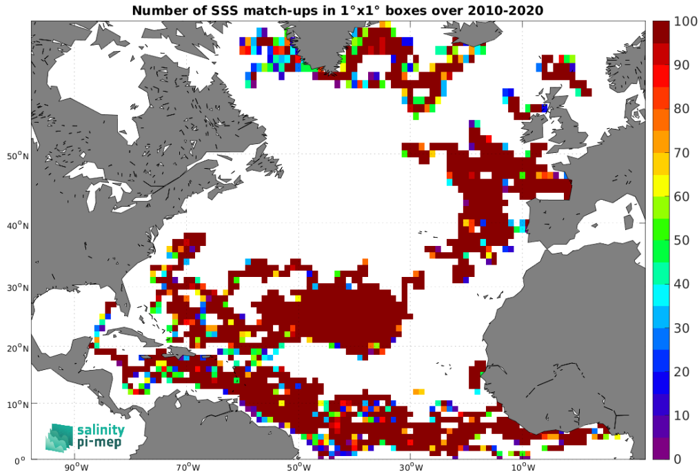
Figure 3: Number of SSS match-ups between Surface drifters SSS and the SMOS SSS L3 v9 - 9 Days (CATDS-CEC-LOCEAN) SSS product for the North Atlantic Ocean Pi-MEP region over 1^\circ \times 1^\circ boxes and for the full satellite product period.
