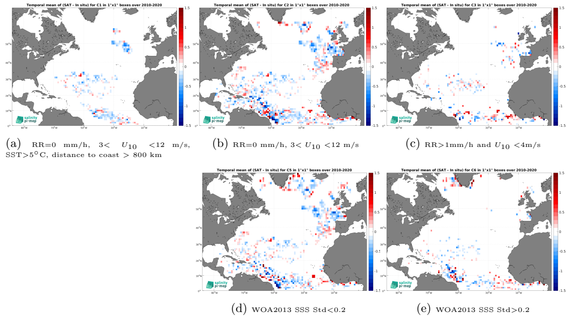
Figure 11: Temporal mean gridded over spatial boxes of size 1^\circ \times 1^\circ of \Delta\text{SSS} (SMOS SSS L3 v9 - 9 Days (CATDS-CEC-LOCEAN) - Surface drifters) for 5 different subdatasets corresponding to:RR=0 mm/h, 3 < U_{10} < 12 m/s, SST >5^\circ\text{C} , distance to coast > 800 km (a), RR=0 mm/h, 3 < U_{10} < 12 m/s (b), RR >1 mm/h and U_{10} < 4 m/s (c), WOA2013 SSS Std <0.2 (d), WOA2013 SSS Std >0.2 (e).
