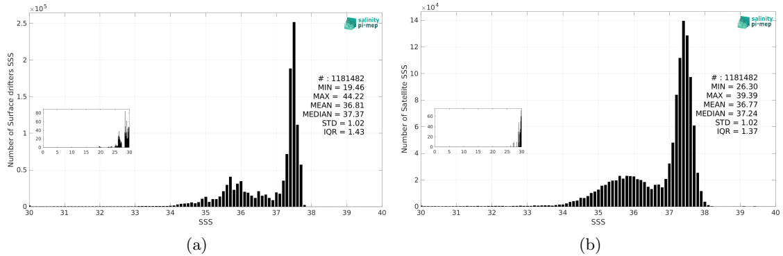
Figure 2: Histograms of SSS from Surface drifters (a) and SMOS SSS L3 v9 - 9 Days (CATDS-CEC-LOCEAN) (b) considering all match-up pairs per bins of 0.1 over the North Atlantic Ocean Pi-MEP region and for the full satellite product period.
