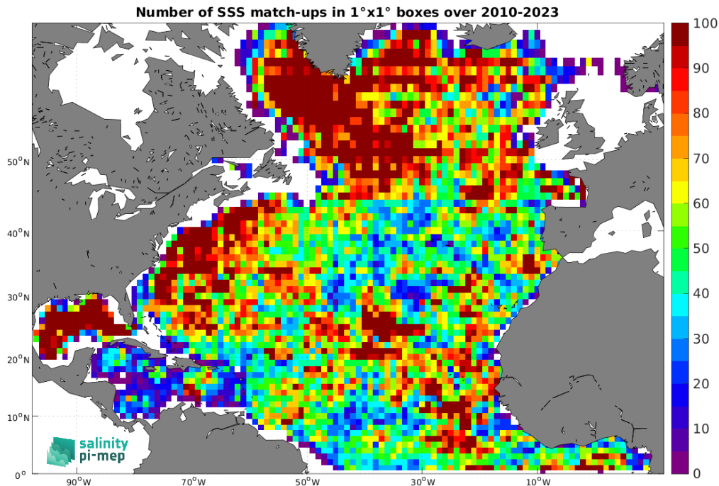
Figure 5: Number of SSS match-ups between Argo SSS and the SMOS SSS L3 v9 - 9 Days (CATDS-CEC-LOCEAN) SSS product for the North Atlantic Ocean Pi-MEP region over 1^\circ \times 1^\circ boxes and for the full satellite product period.
