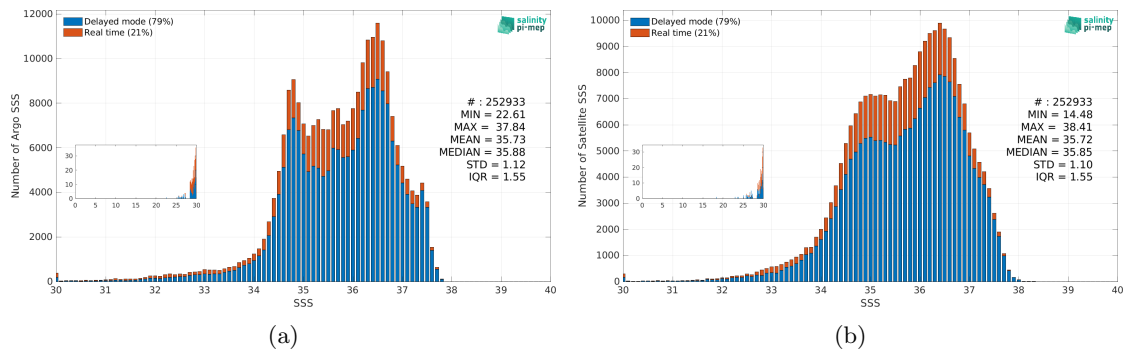
Figure 3: Histograms of SSS from Argo (a) and SMOS SSS L3 v9 - 9 Days (CATDS-CEC-LOCEAN) (b) considering all match-up pairs per bins of 0.1 over the North Atlantic Ocean Pi-MEP region and for the full satellite product period.
