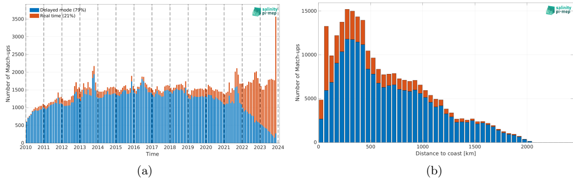
Figure 2: Number of match-ups between Argo and SMOS SSS L3 v9 - 9 Days (CATDS-CEC-LOCEAN) SSS as a function of time (a) and as function of the distance to coast (b) over the North Atlantic Ocean Pi-MEP region and for the full satellite product period.
