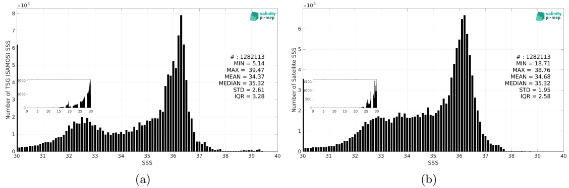
Figure 3: Histograms of SSS from TSG (SAMOS) (a) and SMOS SSS L3 v9 - 18 Days (CATDS-CEC-LOCEAN) (b) considering all match-up pairs per bins of 0.1 over the North Atlantic Ocean Pi-MEP region and for the full satellite product period.
