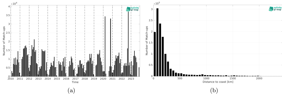
Figure 2: Number of match-ups between TSG (SAMOS) and SMOS SSS L3 v9 - 18 Days (CATDS-CEC-LOCEAN) SSS as a function of time (a) and as function of the distance to coast (b) over the North Atlantic Ocean Pi-MEP region and for the full satellite product period.
