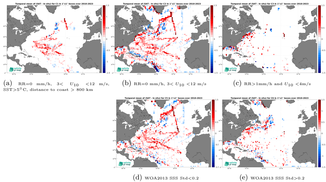
Figure 14: Temporal mean gridded over spatial boxes of size 1^\circ \times 1^\circ of \Delta\text{SSS} (SMOS SSS L3 v9 - 18 Days (CATDS-CEC-LOCEAN) - TSG (SAMOS)) for 5 different subdatasets corresponding to:RR=0 mm/h, 3 < U_{10} < 12 m/s, SST >5^\circ\text{C} , distance to coast > 800 km (a), RR=0 mm/h, 3 < U_{10} < 12 m/s (b), RR >1 mm/h and U_{10} < 4 m/s (c), WOA2013 SSS Std <0.2 (d), WOA2013 SSS Std >0.2 (e).
