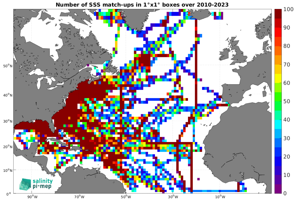
Figure 5: Number of SSS match-ups between TSG (SAMOS) SSS and the SMOS SSS L3 v9 - 18 Days (CATDS-CEC-LOCEAN) SSS product for the North Atlantic Ocean Pi-MEP region over 1^\circ \times 1^\circ boxes and for the full satellite product period.
