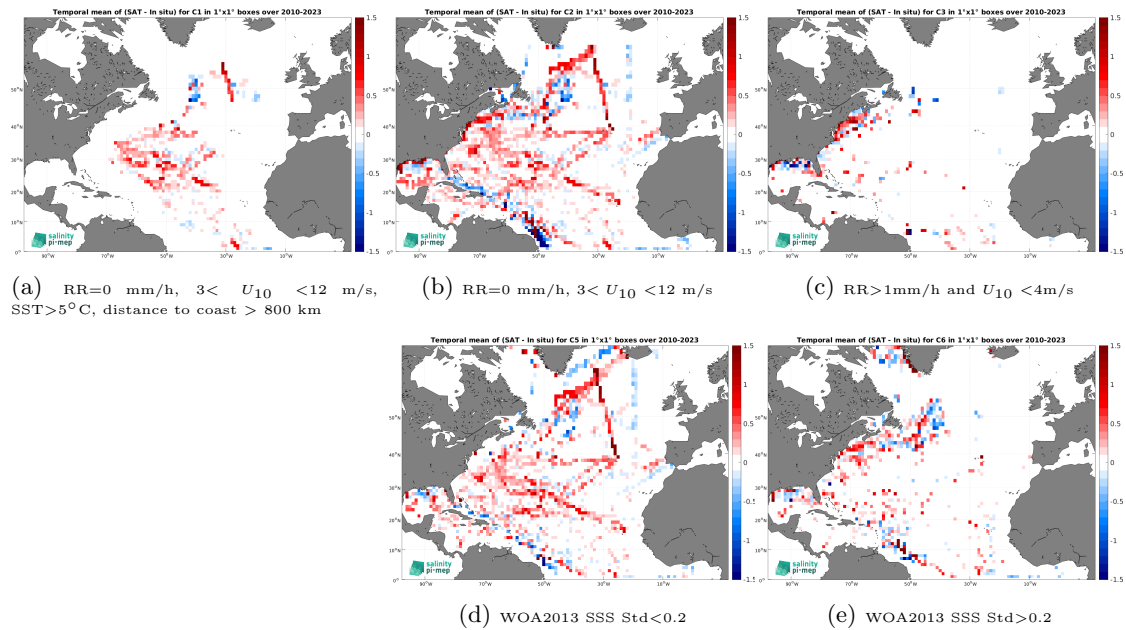
Figure 12: Temporal mean gridded over spatial boxes of size 1^\circ \times 1^\circ of \Delta\text{SSS} (SMOS SSS L3 v9 - 18 Days (CATDS-CEC-LOCEAN) - TSG (SAMOS)) for 5 different subdatasets corresponding to:RR=0 mm/h, 3 < U_{10} < 12 m/s, SST >5^\circ\text{C} , distance to coast > 800 km (a), RR=0 mm/h, 3 < U_{10} < 12 m/s (b), RR >1 mm/h and U_{10} < 4 m/s (c), WOA2013 SSS Std <0.2 (d), WOA2013 SSS Std >0.2 (e).
