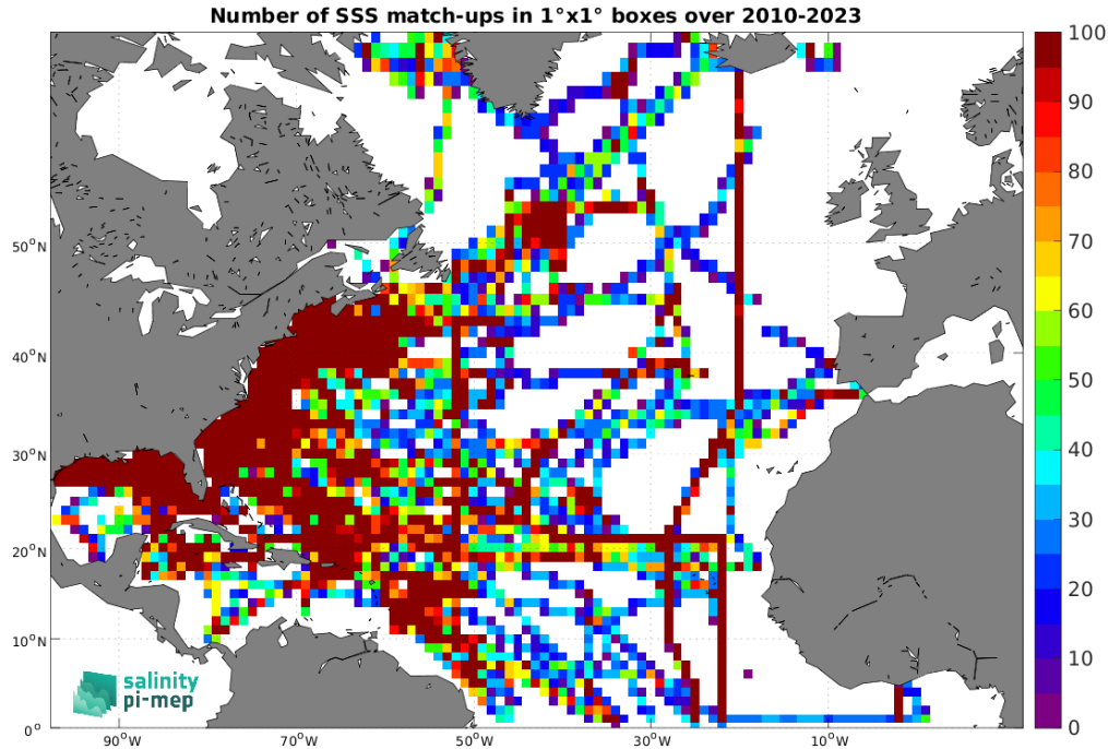
Figure 4: Number of SSS match-ups between TSG (SAMOS) SSS and the SMOS SSS L3 v9 - 18 Days (CATDS-CEC-LOCEAN) SSS product for the North Atlantic Ocean Pi-MEP region over 1^\circ \times 1^\circ boxes and for the full satellite product period.
