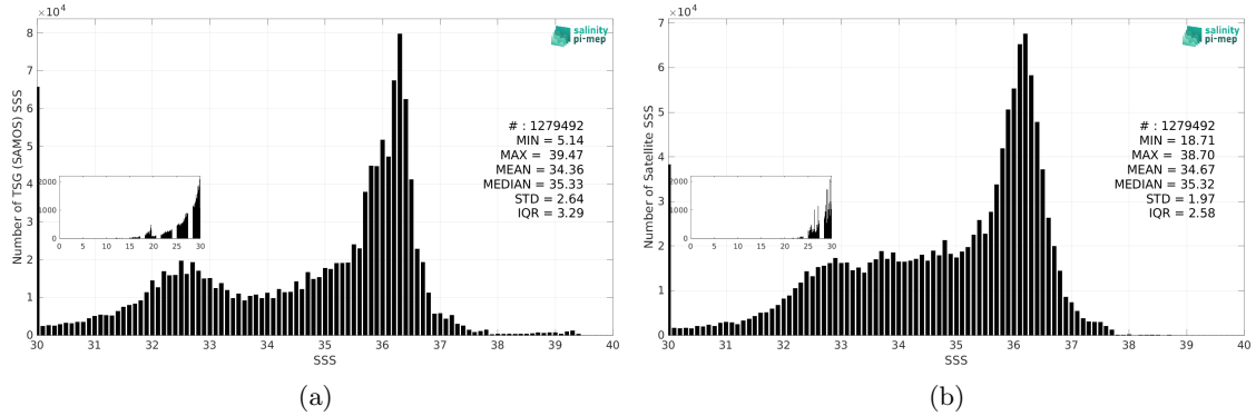
Figure 2: Histograms of SSS from TSG (SAMOS) (a) and SMOS SSS L3 v9 - 18 Days (CATDS-CEC-LOCEAN) (b) considering all match-up pairs per bins of 0.1 over the North Atlantic Ocean Pi-MEP region and for the full satellite product period.
