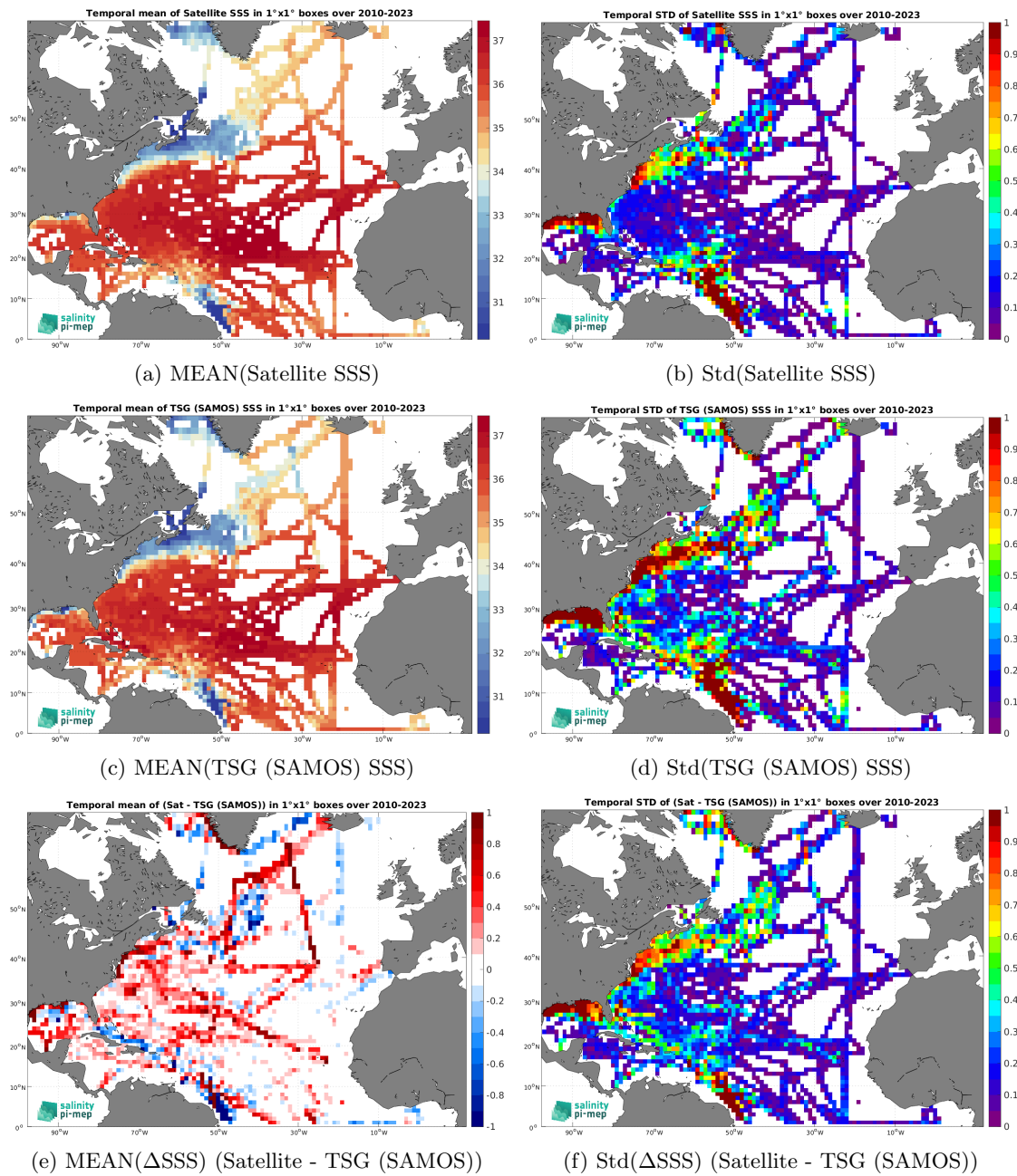
Figure 6: Temporal mean (left) and Std (right) of SSS from SMOS SSS L3 v9 - 18 Days (CATDS-CEC-LOCEAN) (top), TSG (SAMOS) (middle), and of \Delta SSS (Satellite - TSG (SAMOS)). Only match-up pairs are used to generate these maps.
