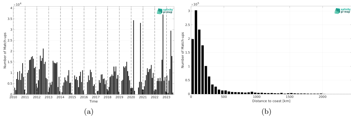
Figure 1: Number of match-ups between TSG (SAMOS) and SMOS SSS L3 v9 - 18 Days (CATDS-CEC-LOCEAN) SSS as a function of time (a) and as function of the distance to coast (b) over the North Atlantic Ocean Pi-MEP region and for the full satellite product period.
