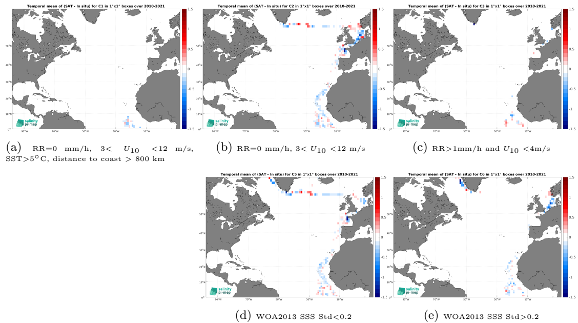
Figure 12: Temporal mean gridded over spatial boxes of size 1^\circ \times 1^\circ of \Delta\text{SSS} (SMOS SSS L3 v9 - 18 Days (CATDS-CEC-LOCEAN) - TSG (Polarstern)) for 5 different subdatasets corresponding to:RR=0 mm/h, 3 < U_{10} < 12 m/s, SST >5^\circ\text{C} , distance to coast > 800 km (a), RR=0 mm/h, 3 < U_{10} < 12 m/s (b), RR >1 mm/h and U_{10} < 4 m/s (c), WOA2013 SSS Std <0.2 (d), WOA2013 SSS Std >0.2 (e).
