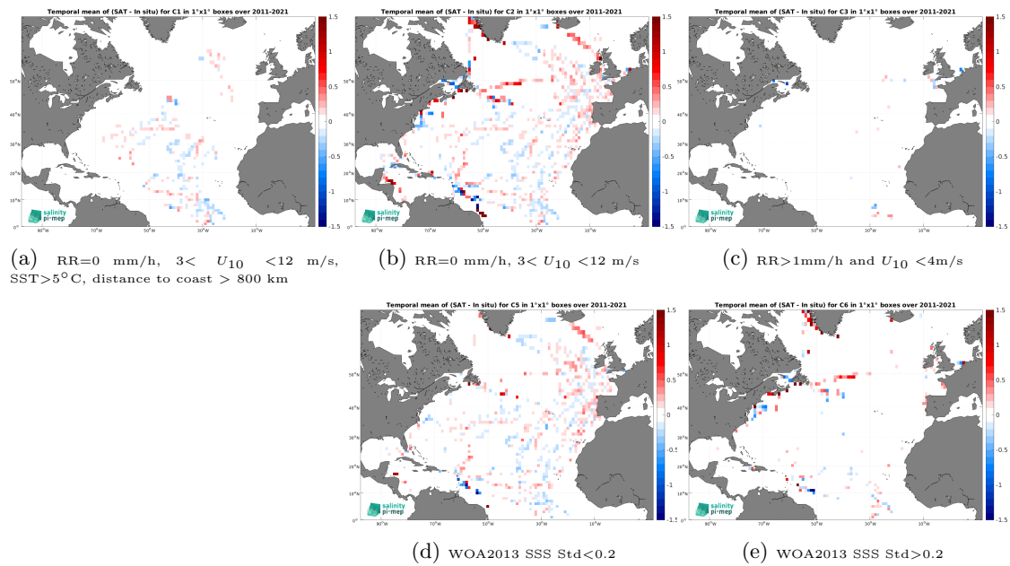
Figure 14: Temporal mean gridded over spatial boxes of size 1^\circ \times 1^\circ of \Delta\text{SSS} (SMOS SSS L3 v9 - 18 Days (CATDS-CEC-LOCEAN) - TSG (GOSUD-Sailing-ship)) for 5 different subdatasets corresponding to:RR=0 mm/h, 3 < U_{10} < 12 m/s, SST>5°C, distance to coast > 800 km (a), RR=0 mm/h, 3 < U_{10} < 12 m/s (b), RR>1mm/h and U_{10} < 4 m/s (c), WOA2013 SSS Std<0.2 (d), WOA2013 SSS Std>0.2 (e).
