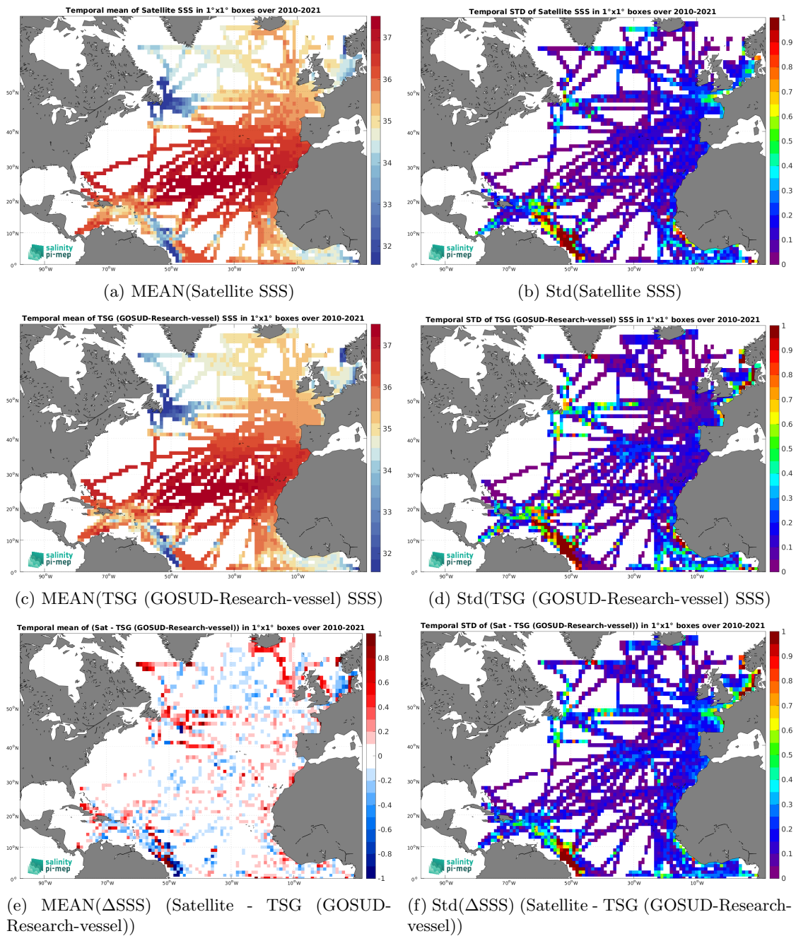
Figure 6: Temporal mean (left) and Std (right) of SSS from SMOS SSS L3 v9 - 18 Days (CATDS-CEC-LOCEAN) (top), TSG (GOSUD-Research-vessel) (middle), and of \Delta SSS (Satellite - TSG (GOSUD-Research-vessel)). Only match-up pairs are used to generate these maps.
