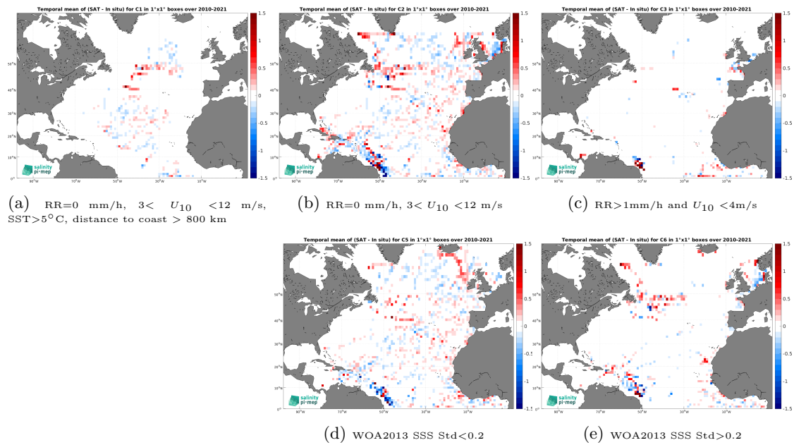
Figure 12: Temporal mean gridded over spatial boxes of size 1^\circ \times 1^\circ of \Delta\text{SSS} (SMOS SSS L3 v9 - 18 Days (CATDS-CEC-LOCEAN) - TSG (GOSUD-Research-vessel)) for 5 different subdatasets corresponding to:RR=0 mm/h, 3 < U_{10} < 12 m/s, SST >5^\circ\text{C} , distance to coast > 800 km (a), RR=0 mm/h, 3 < U_{10} < 12 m/s (b), RR >1 mm/h and U_{10} < 4 m/s (c), WOA2013 SSS Std <0.2 (d), WOA2013 SSS Std >0.2 (e).
