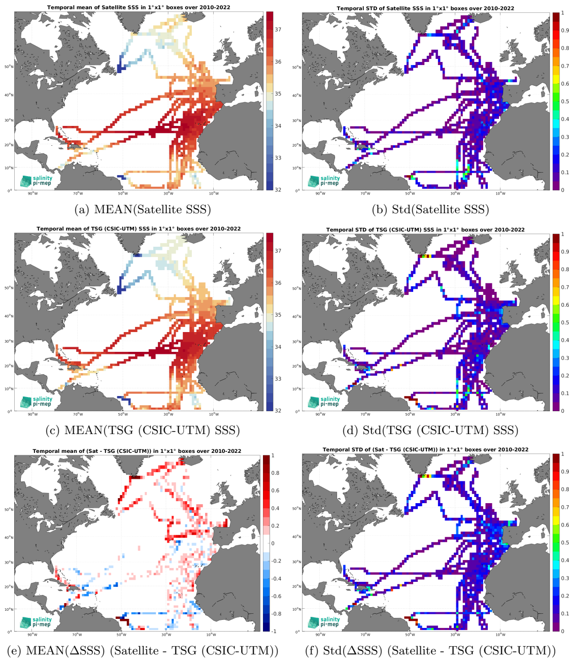
Figure 6: Temporal mean (left) and Std (right) of SSS from SMOS SSS L3 v9 - 18 Days (CATDS-CEC-LOCEAN) (top), TSG (CSIC-UTM) (middle), and of \Delta SSS (Satellite - TSG (CSIC-UTM)). Only match-up pairs are used to generate these maps.
