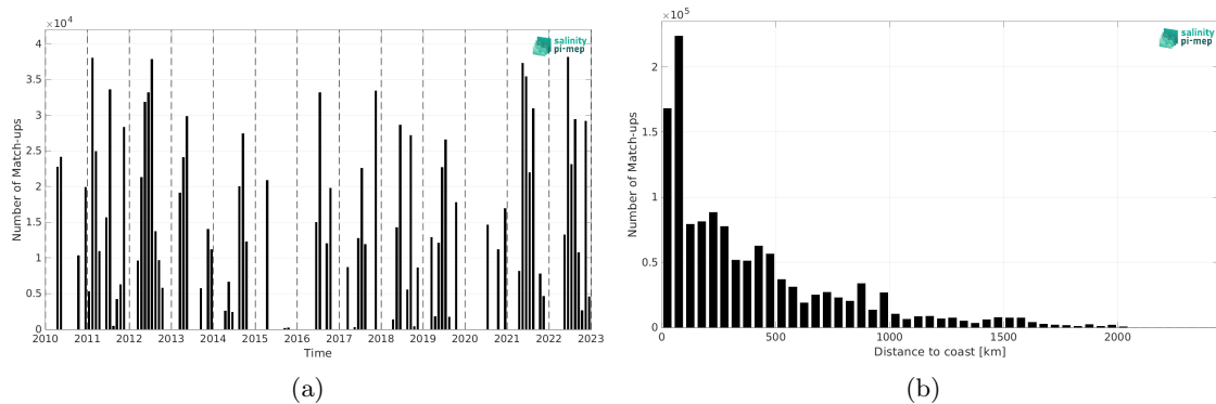
Figure 1: Number of match-ups between TSG (CSIC-UTM) and SMOS SSS L3 v9 - 18 Days (CATDS-CEC-LOCEAN) SSS as a function of time (a) and as function of the distance to coast (b) over the North Atlantic Ocean Pi-MEP region and for the full satellite product period.
