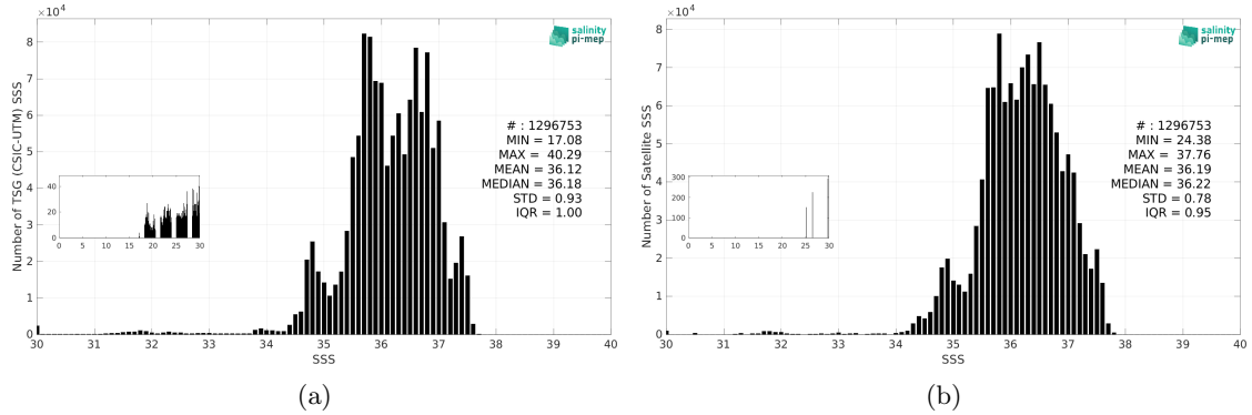
Figure 2: Histograms of SSS from TSG (CSIC-UTM) (a) and SMOS SSS L3 v9 - 18 Days (CATDS-CEC-LOCEAN) (b) considering all match-up pairs per bins of 0.1 over the North Atlantic Ocean Pi-MEP region and for the full satellite product period.
