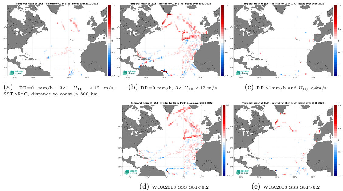
Figure 12: Temporal mean gridded over spatial boxes of size 1^\circ \times 1^\circ of \Delta\text{SSS} (SMOS SSS L3 v9 - 18 Days (CATDS-CEC-LOCEAN) - TSG (CSIC-UTM)) for 5 different subdatasets corresponding to:RR=0 mm/h, 3 < U_{10} < 12 m/s, SST >5^\circ\text{C} , distance to coast > 800 km (a), RR=0 mm/h, 3 < U_{10} < 12 m/s (b), RR >1 mm/h and U_{10} < 4 m/s (c), WOA2013 SSS Std <0.2 (d), WOA2013 SSS Std >0.2 (e).
